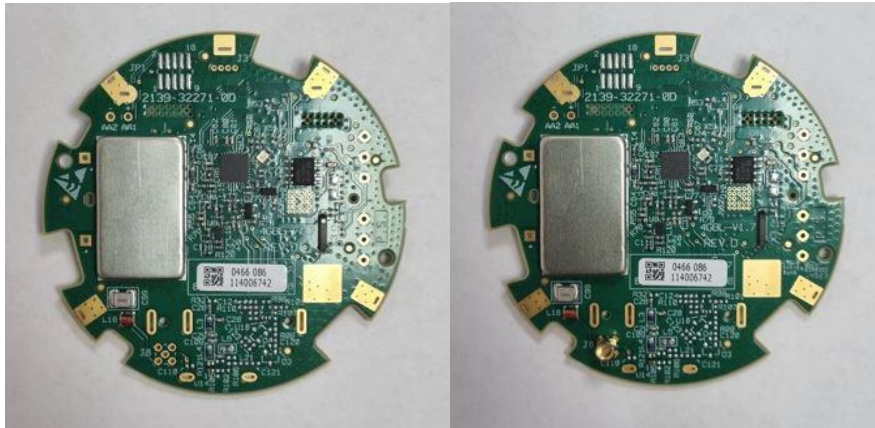
RF card- bottom, identical but extra mmc connector for external antenna configuration (right card)
