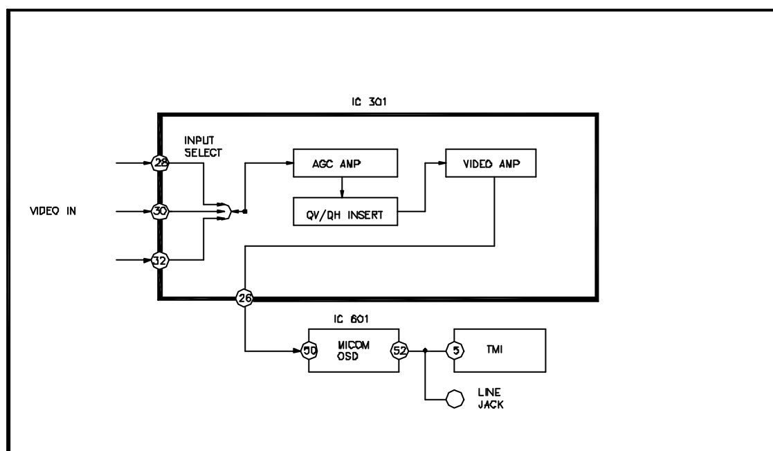
Fig. 3-1 EE mode process
