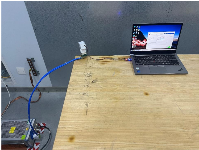
POWERLINE CONDUCTED EMISSIONS MEASUREMENT SETUP
