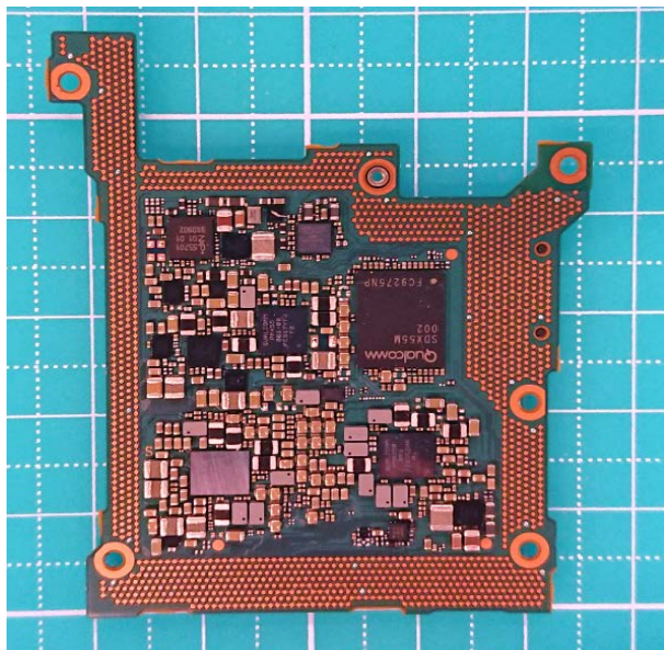
Internal Main-PWB of Rear (Front-side)
