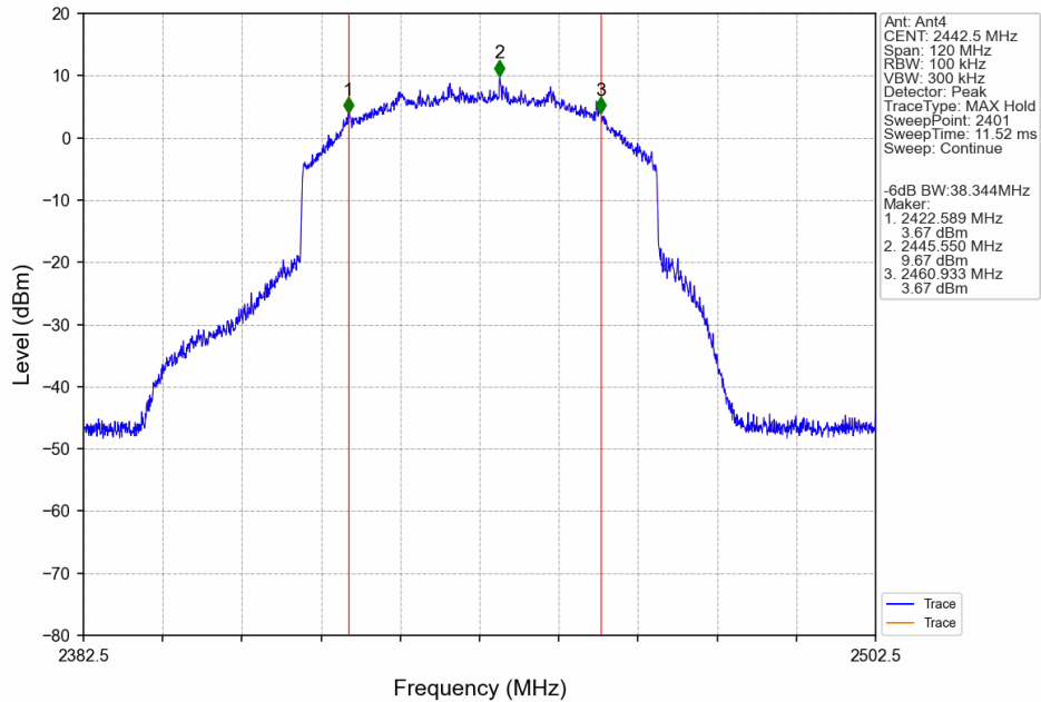
60M_HCH_2442.5MHz_Ant4_NTNV
