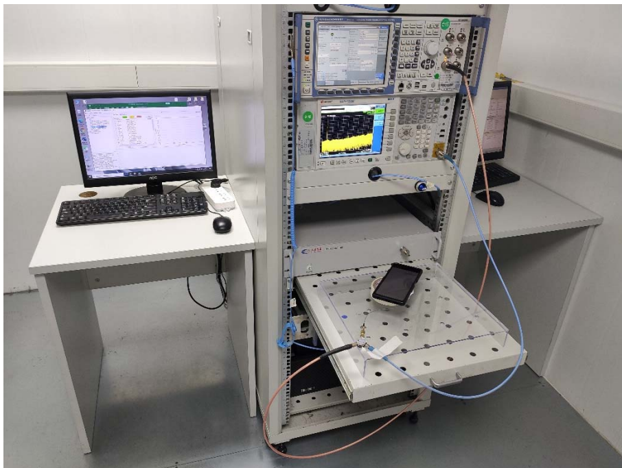
Conducted Test-BR&EDR
