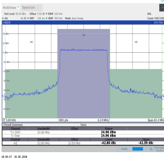
Band48-20MHz-QPSK-56640-100RB#0-PASS
