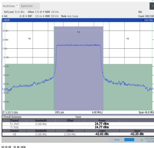
Band48-15MHz-QPSK-55315-75RB#0-PASS
