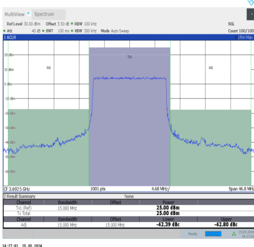
Band48-15MHz-QPSK-56665-75RB#0-PASS
