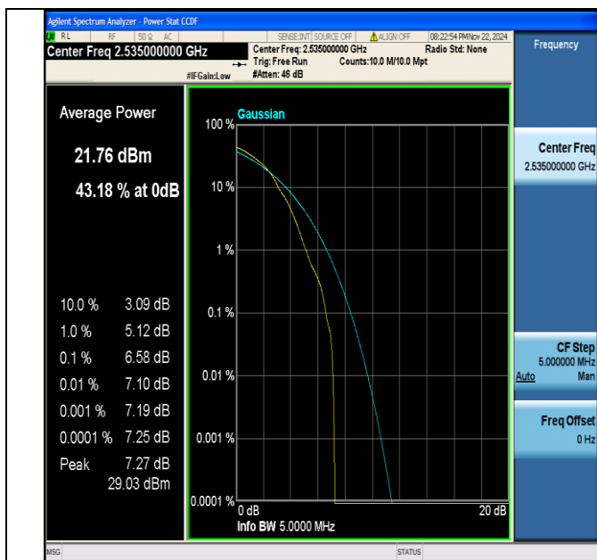
Band7-5MHz-64QAM-21100-1RB#0-PASS
