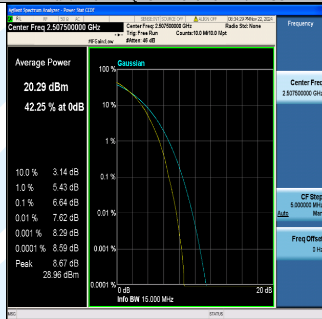
Band7-15MHz-64QAM-20825-75RB#0-PASS
