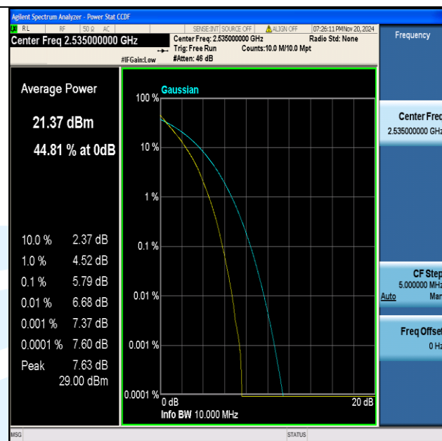
Band7-10MHz-QPSK-21100-50RB#0-PASS
