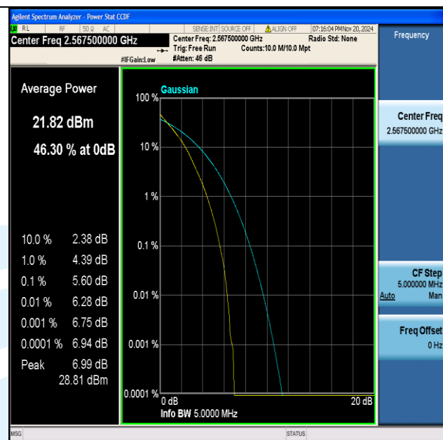
Band7-5MHz-QPSK-21425-25RB#0-PASS
