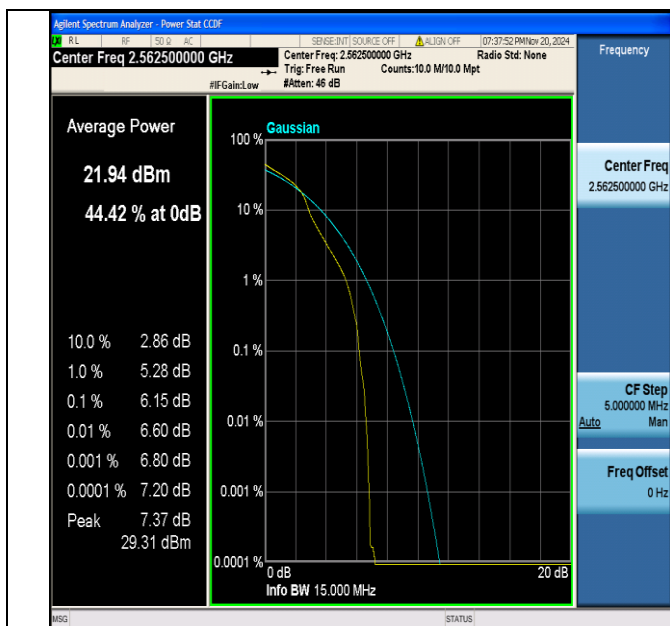
Band7-15MHz-16QAM-21375-1RB#0-PASS
