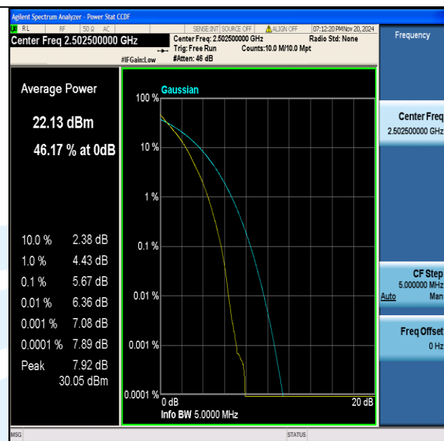
Band7-5MHz-QPSK-20775-25RB#0-PASS
