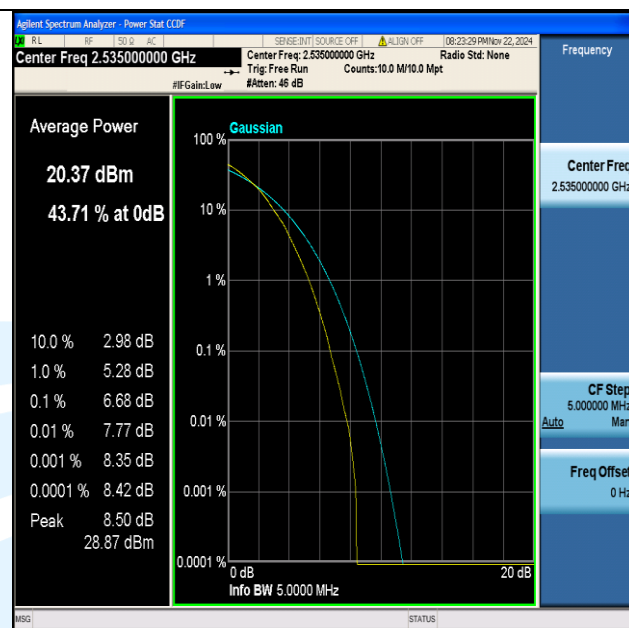
Band7-5MHz-64QAM-21100-25RB#0-PASS
