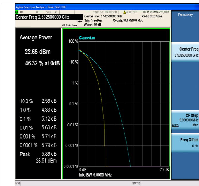
Band7-5MHz-QPSK-20775-1RB#0-PASS
