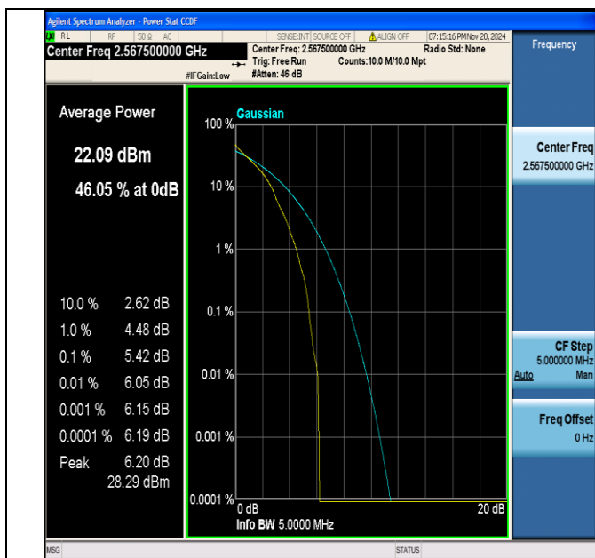
Band7-5MHz-QPSK-21425-1RB#0-PASS
