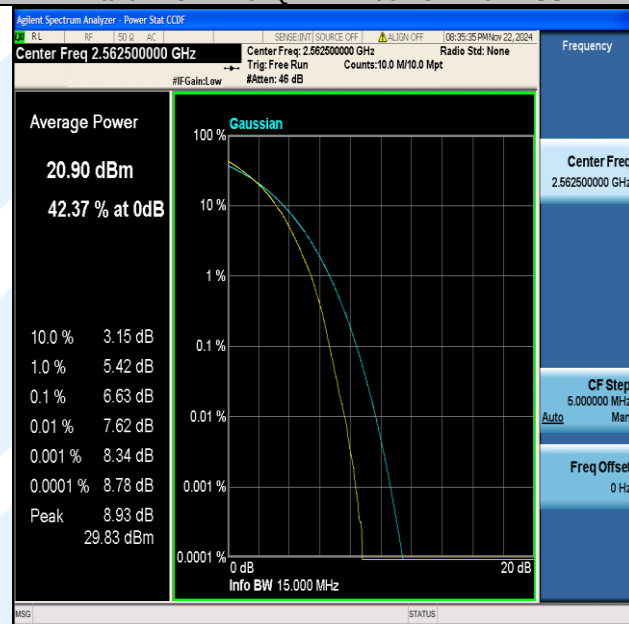
Band7-15MHz-64QAM-21375-75RB#0-PASS
