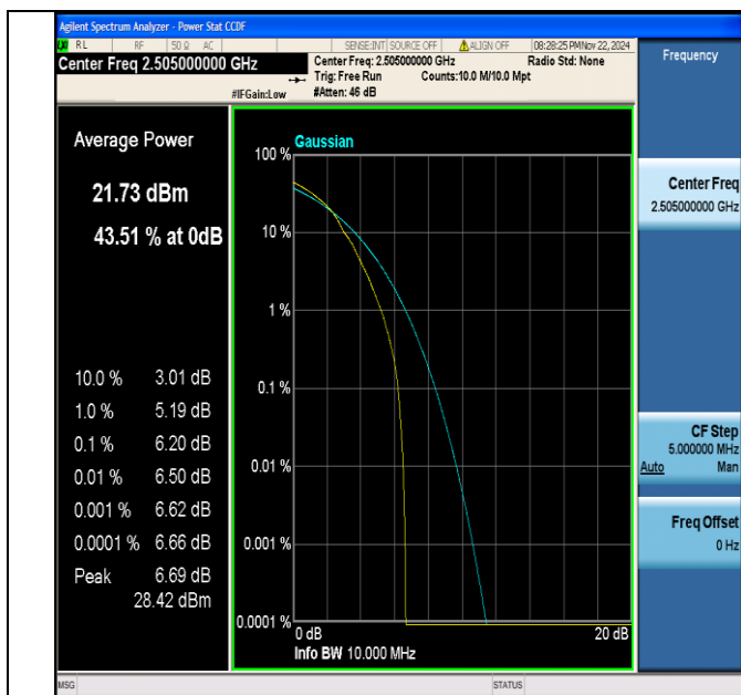
Band7-10MHz-64QAM-20800-1RB#0-PASS
