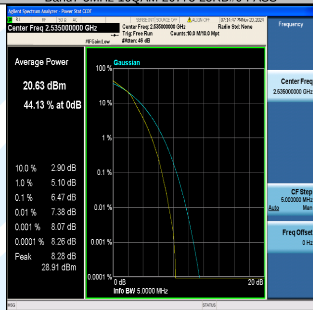
Band7-5MHz-16QAM-21100-25RB#0-PASS
