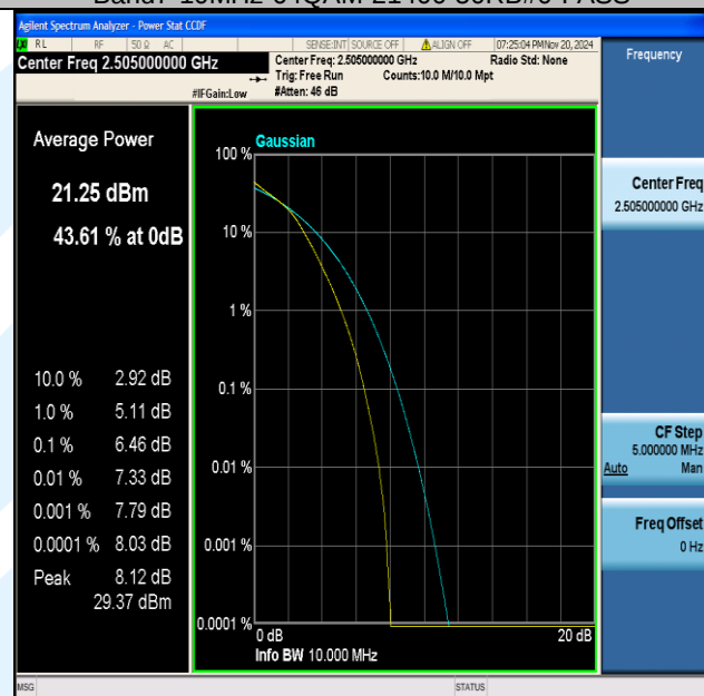
Band7-10MHz-16QAM-20800-50RB#0-PASS
