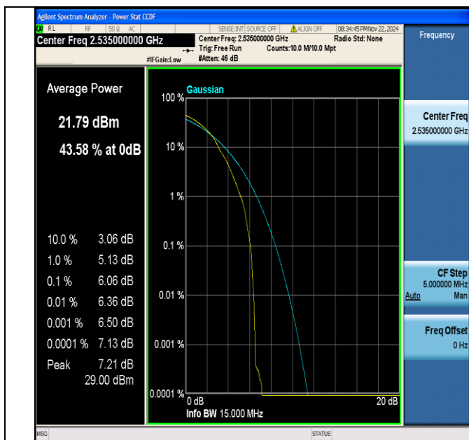
Band7-15MHz-64QAM-21100-1RB#0-PASS
