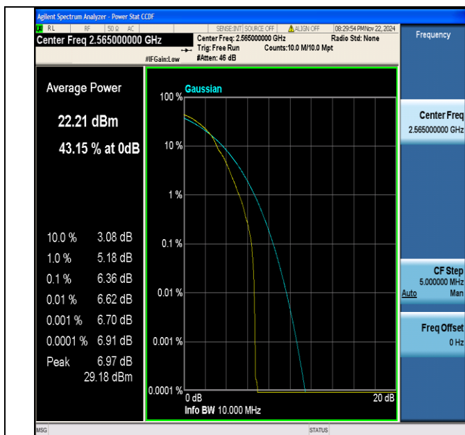
Band7-10MHz-64QAM-21400-1RB#0-PASS
