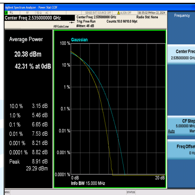
Band7-15MHz-64QAM-21100-75RB#0-PASS
