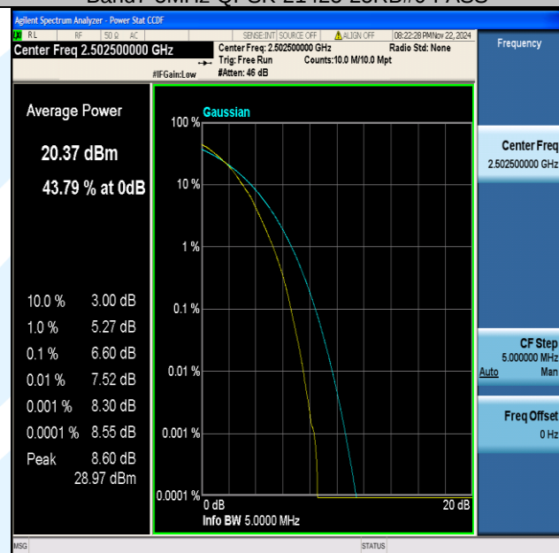
Band7-5MHz-64QAM-20775-25RB#0-PASS
