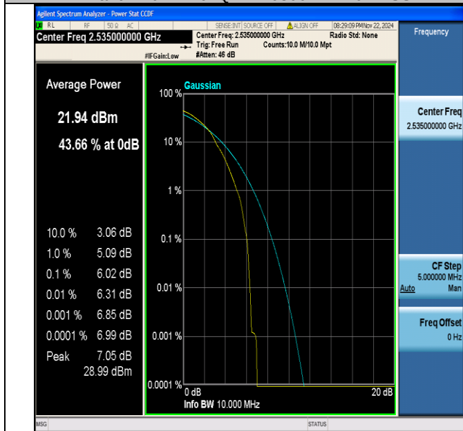
Band7-10MHz-64QAM-21100-1RB#0-PASS
