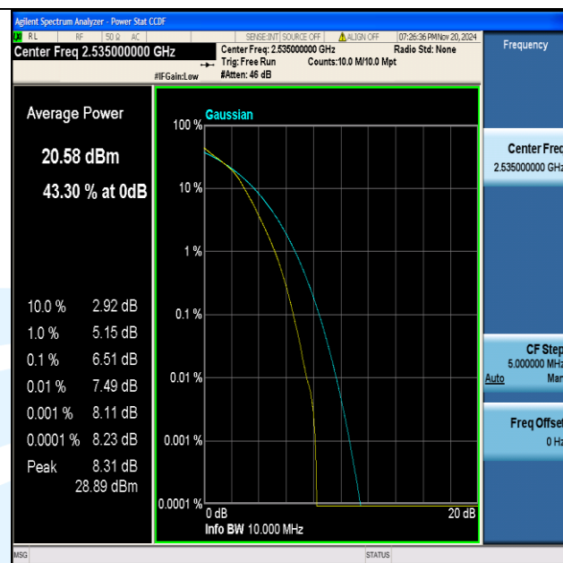
Band7-10MHz-16QAM-21100-50RB#0-PASS
