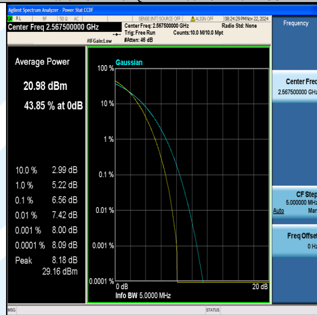
Band7-5MHz-64QAM-21425-25RB#0-PASS
