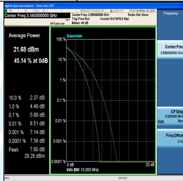
Band7-10MHz-QPSK-21400-50RB#0-PASS
