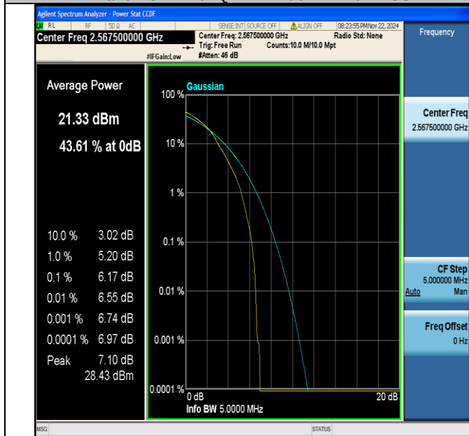
Band7-5MHz-64QAM-21425-1RB#0-PASS
