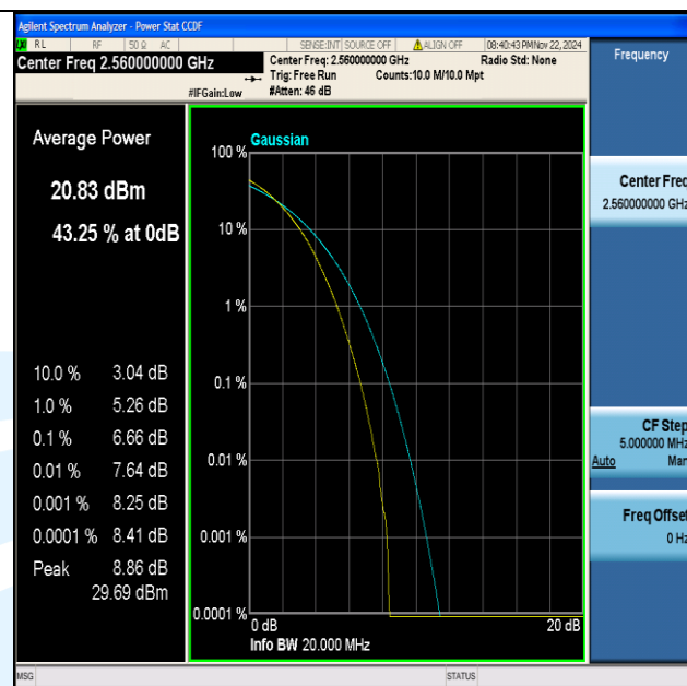
Band7-20MHz-64QAM-21350-100RB#0-PASS
