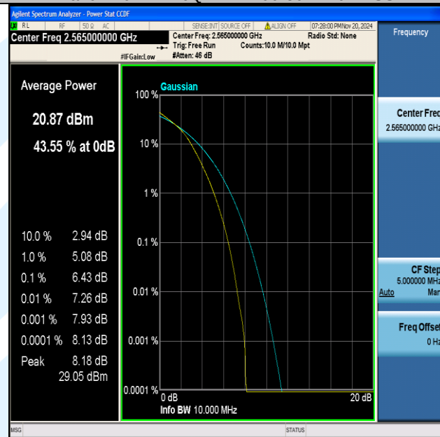
Band7-10MHz-16QAM-21400-50RB#0-PASS
