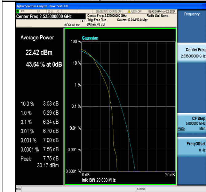
Band7-20MHz-64QAM-21100-1RB#0-PASS
