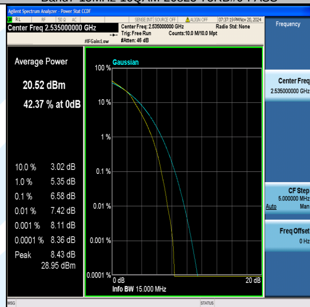
Band7-15MHz-16QAM-21100-75RB#0-PASS
