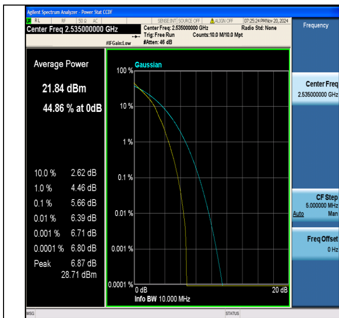
Band7-10MHz-QPSK-21100-1RB#0-PASS
