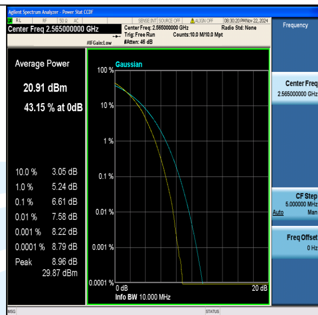
Band7-10MHz-64QAM-21400-50RB#0-PASS
