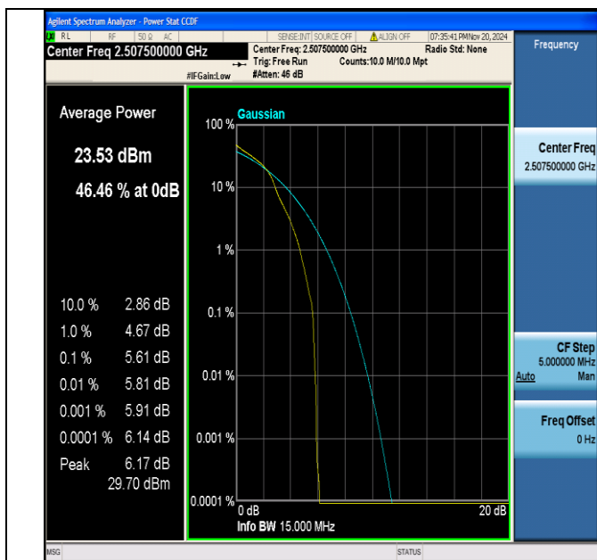
Band7-15MHz-16QAM-20825-1RB#0-PASS
