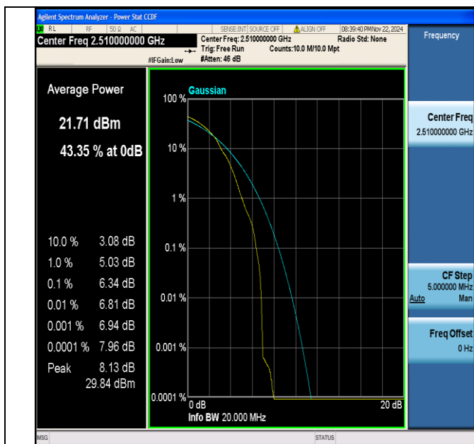
Band7-20MHz-64QAM-20850-1RB#0-PASS
