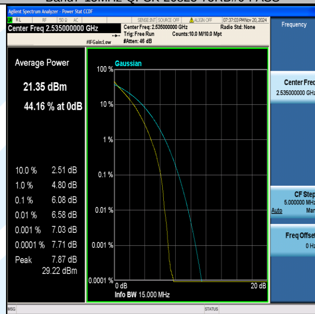
Band7-15MHz-QPSK-21100-75RB#0-PASS
