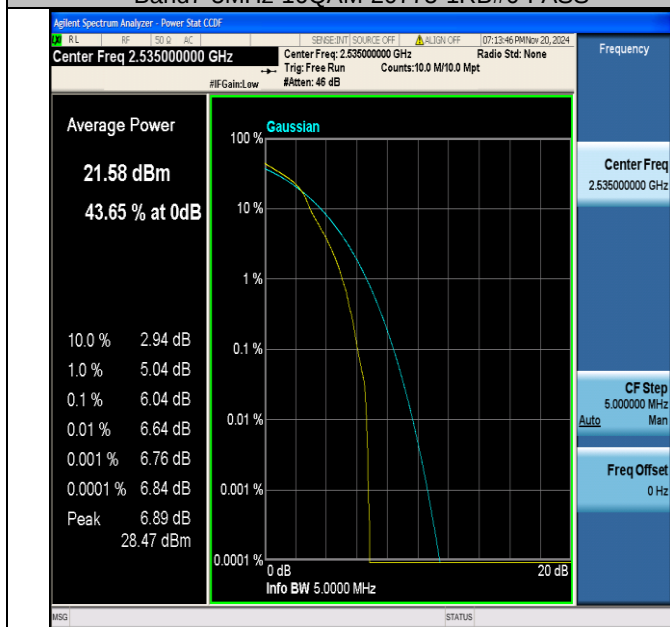
Band7-5MHz-16QAM-21100-1RB#0-PASS
