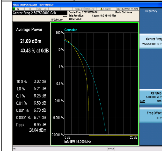
Band7-15MHz-64QAM-20825-1RB#0-PASS
