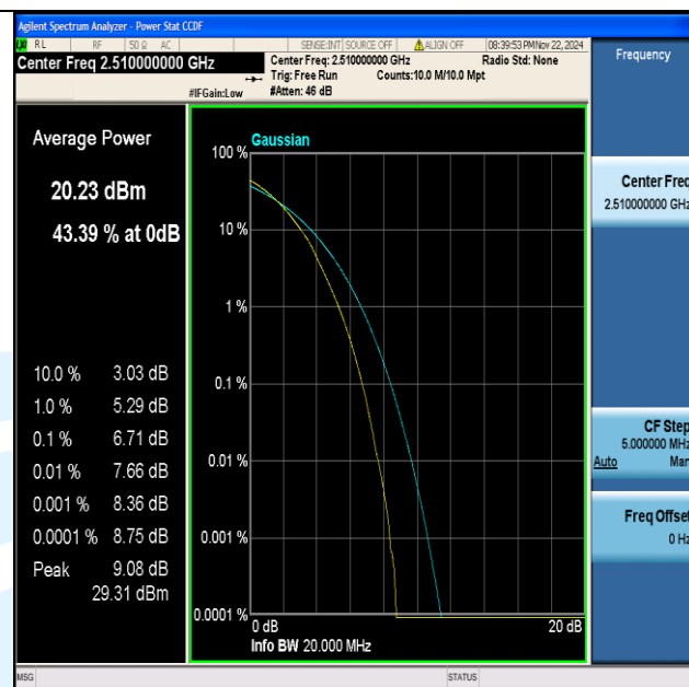
Band7-20MHz-64QAM-20850-100RB#0-PASS
