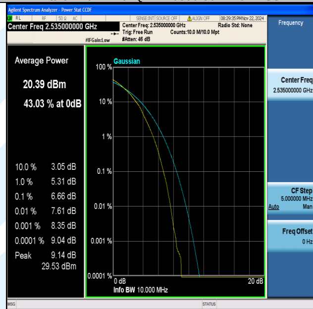
Band7-10MHz-64QAM-21100-50RB#0-PASS
