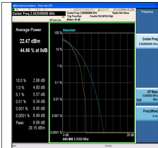
Band7-5MHz-16QAM-20775-1RB#0-PASS
