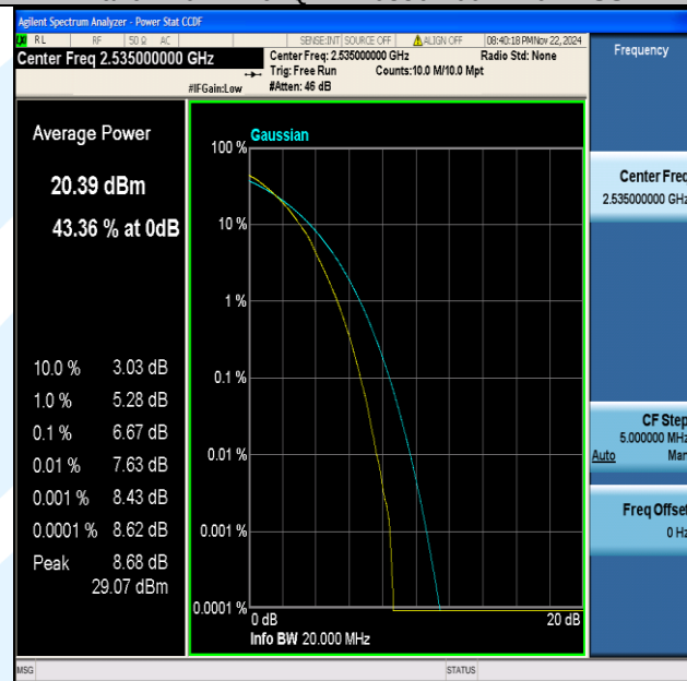
Band7-20MHz-64QAM-21100-100RB#0-PASS
