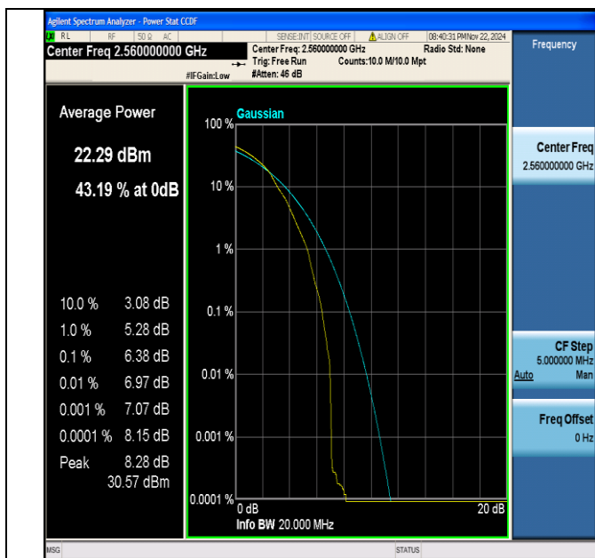
Band7-20MHz-64QAM-21350-1RB#0-PASS
