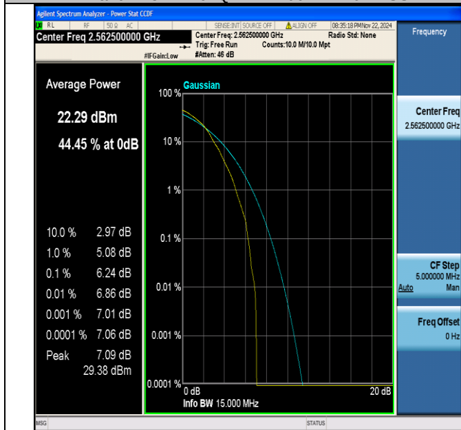
Band7-15MHz-64QAM-21375-1RB#0-PASS
