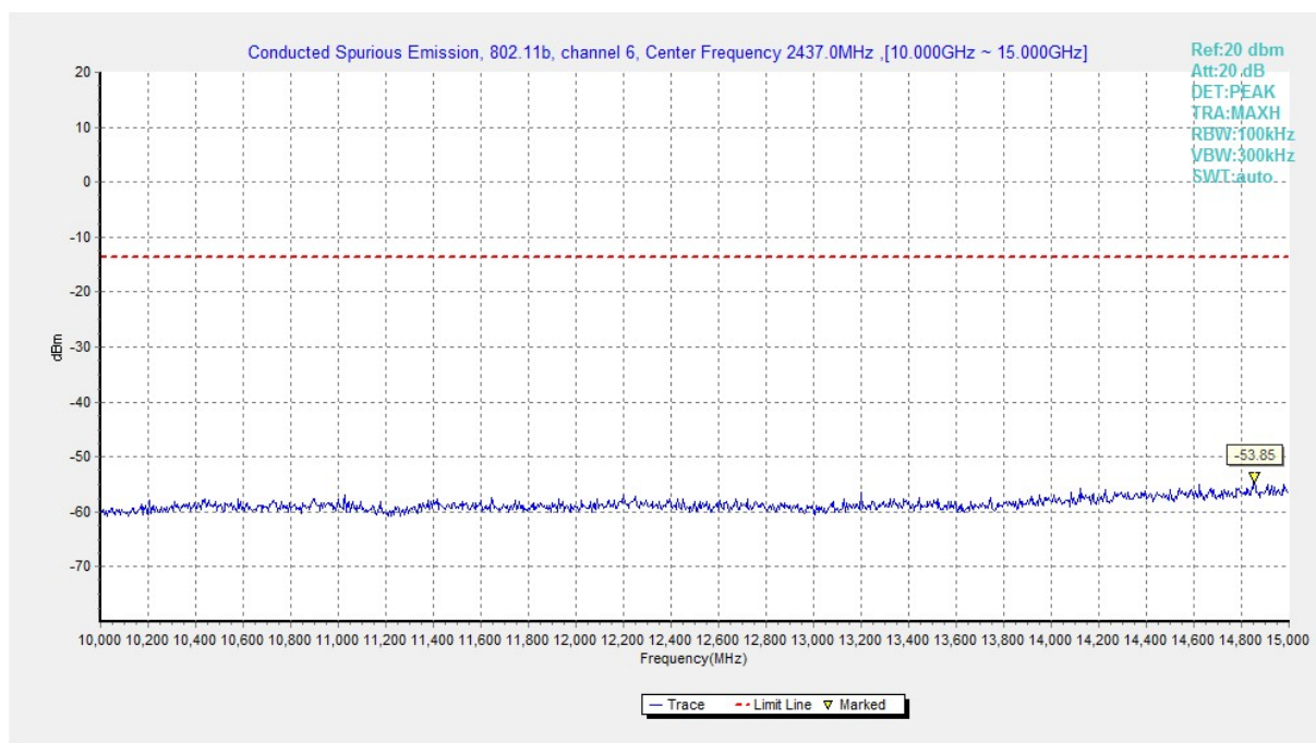
Fig.B.6.1.14 Transmitter Spurious Emission - Conducted (802.11b, Ch6, 10 GHz-15 GHz)
