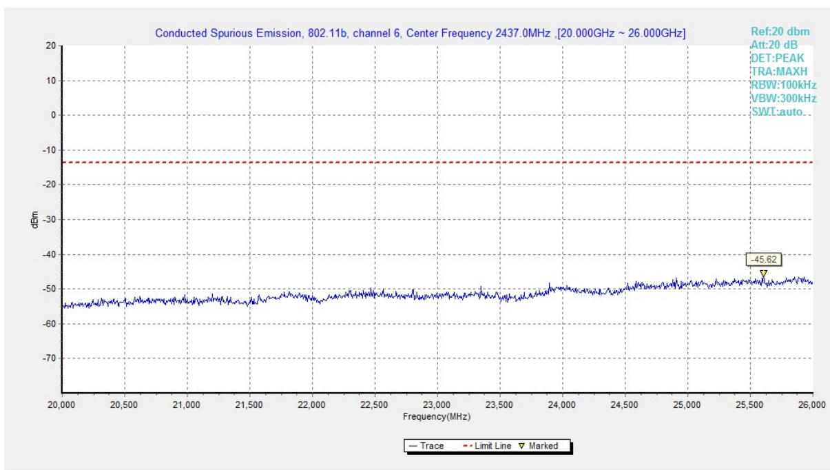
Fig.B.6.1.16 Transmitter Spurious Emission - Conducted (802.11b, Ch6, 20 GHz-26 GHz)
