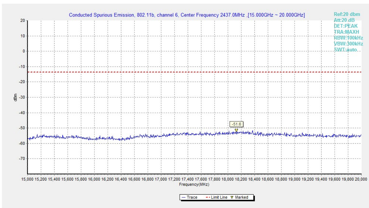
Fig.B.6.1.15 Transmitter Spurious Emission - Conducted (802.11b, Ch6, 15 GHz-20 GHz)
