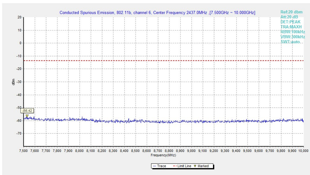
Fig.B.6.1.13 Transmitter Spurious Emission - Conducted (802.11b, Ch6, 7.5 GHz-10 GHz)
