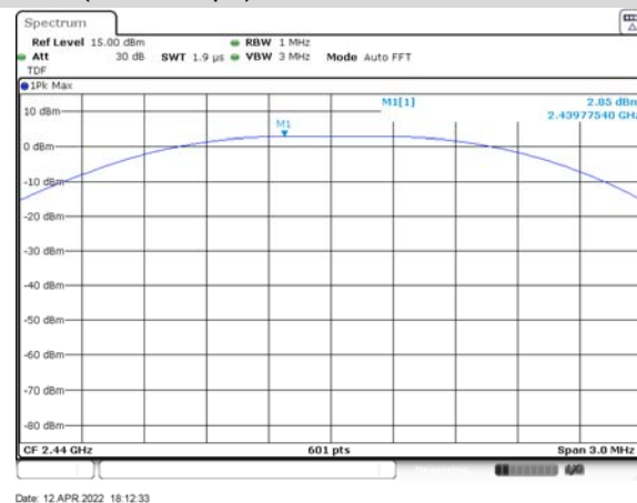
GFSK (BLE 1Mbps) MIDDLE CHANNEL
