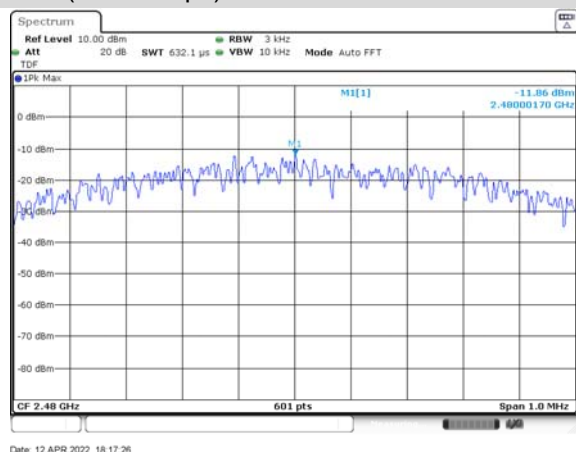
GFSK (BLE 1Mbps) HIGH CHANNEL
