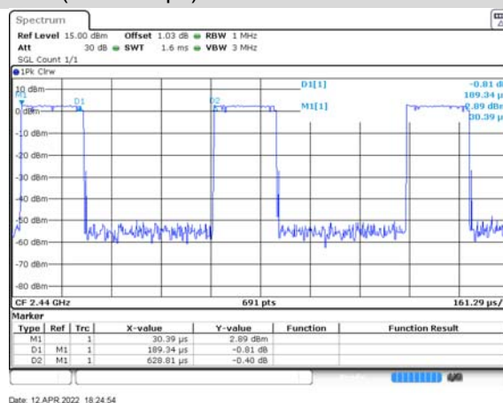
GFSK (BLE 2Mbps)
