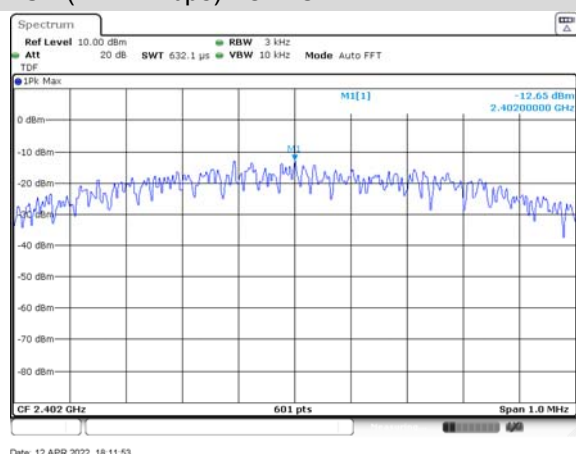
GFSK (BLE 1Mbps) LOW CHANNEL
