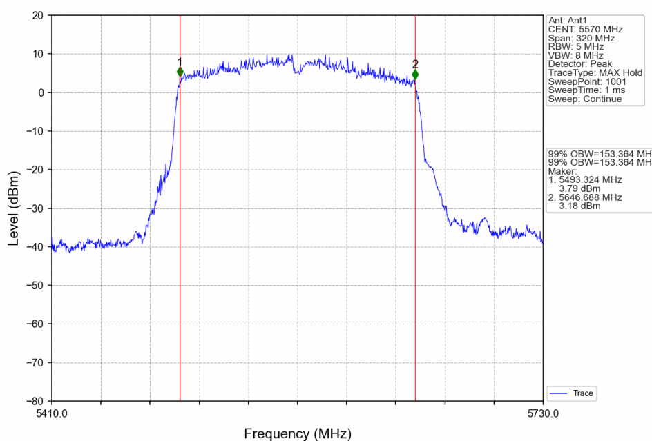
802.11ac(VHT160)_MCH_5570MHz_Ant1_NTNV
