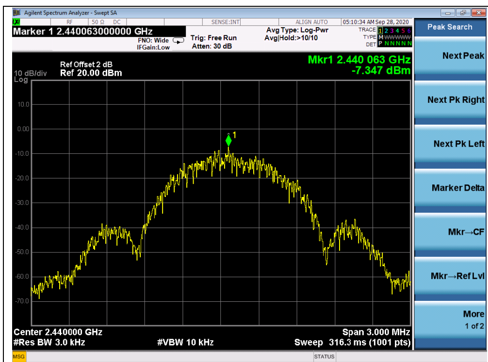
(Channel 19, 2440MHz)
