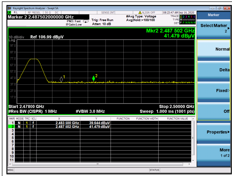
(PEAK, Channel 39)
