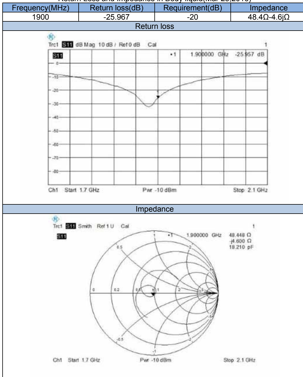
Return Loss and Impedance in Body liquid(Mar 25,2016)
