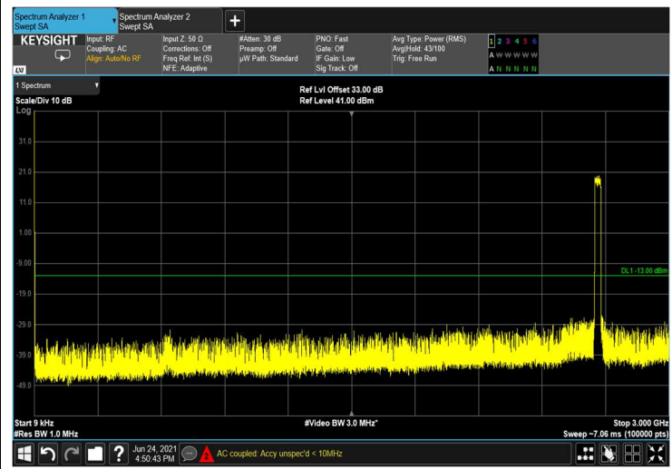
Figure 436: 9kHz-3GHz
