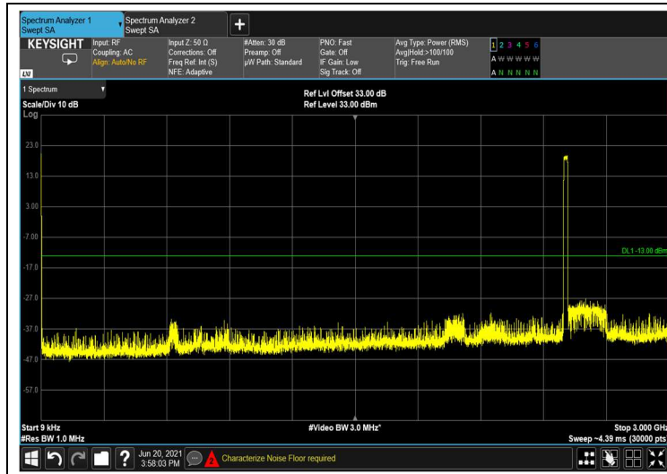
Figure 450: 9kHz-3GHz
