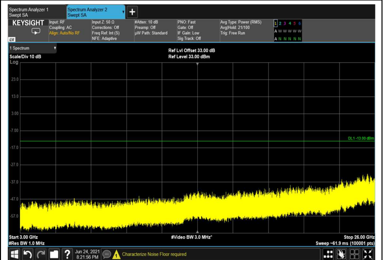
Spurious Emissions at Antenna Terminal QPSK 60MHz B.W.; 2660.0MHz, 30kHz
