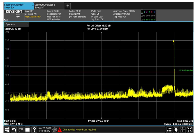
Figure 454: 9kHz-3GHz
