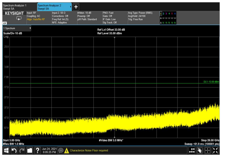
Figure 447: 3GHz-26GHz
