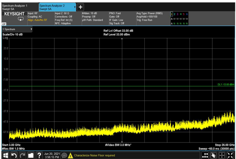
Figure 463: 3GHz-26GHz
