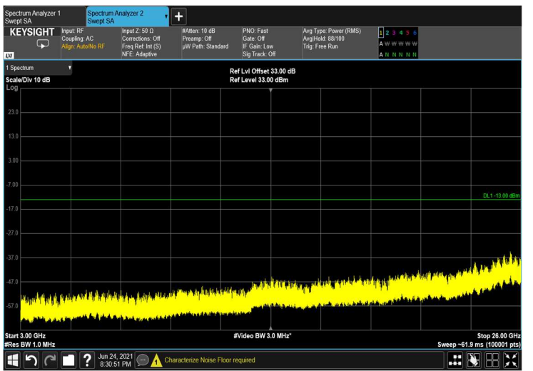
Spurious Emissions at Antenna Terminal QPSK 60MHz B.W.; 2660.0MHz, 60kHz
