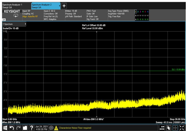
Figure 437: 3GHz-26GHz
