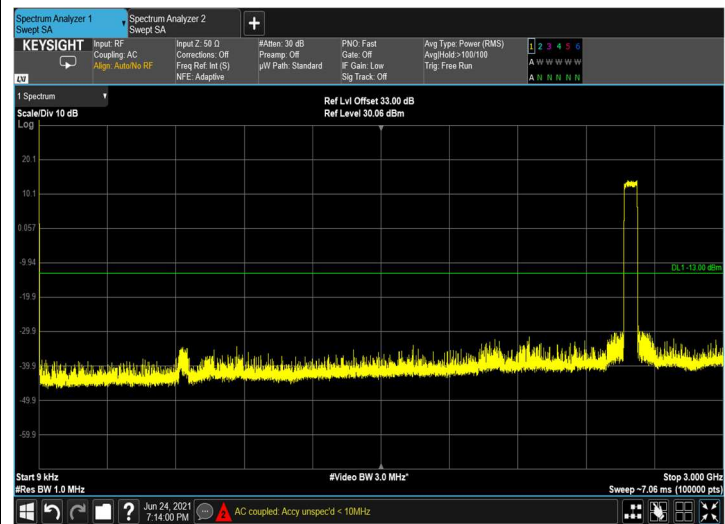
Spurious Emissions at Antenna Terminal QPSK 60MHz B.W.; 2593.0MHz, 30kHz
