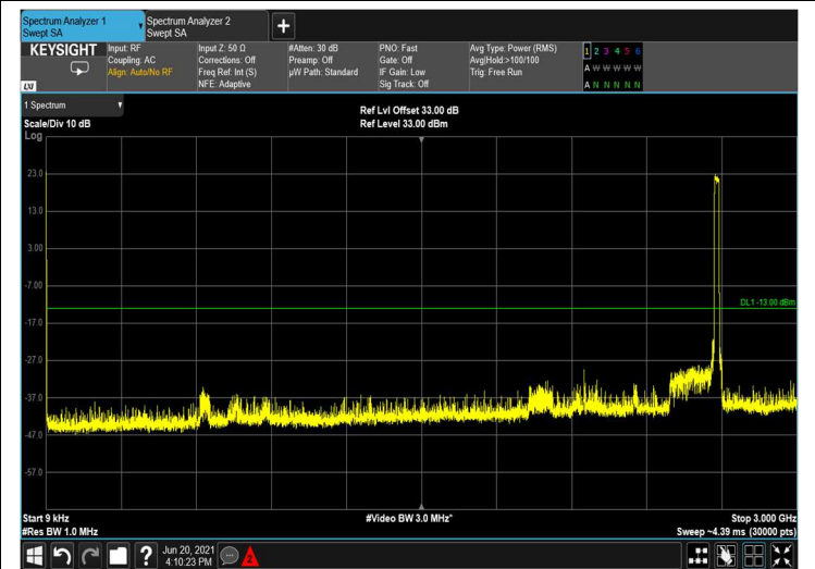
Spurious Emissions at Antenna Terminal 64QAM 20MHz B.W.; 2680.0MHz
