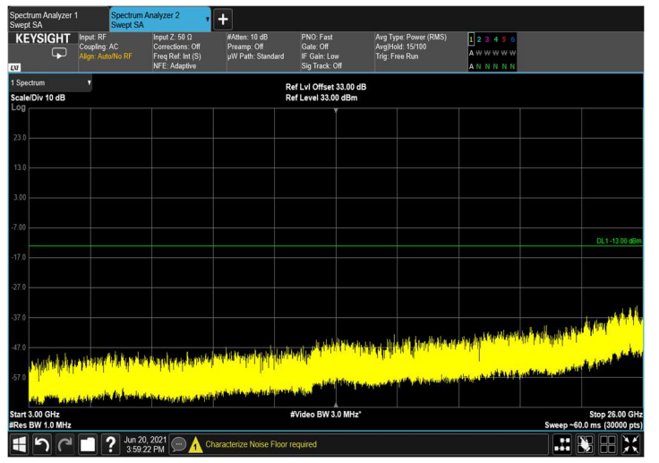
Figure 457: 3GHz-26GHz
