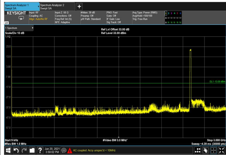
Figure 456: 9kHz-3GHz
