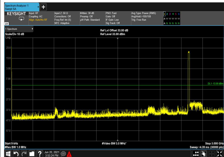
Figure 462: 9kHz-3GHz
