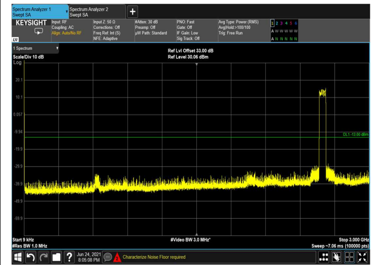
Figure 446: 9kHz-3GHz
