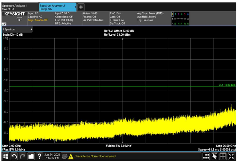
Spurious Emissions at Antenna Terminal QPSK 60MHz B.W.; 2593.0MHz, 30kHz
