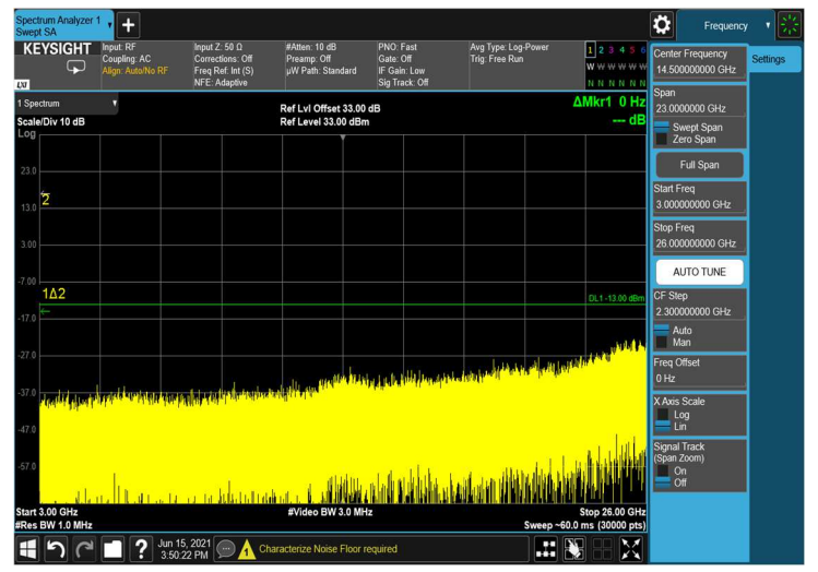
Spurious Emissions at Antenna Terminal 64QAM 20MHz B.W.; 2593.0MHz
