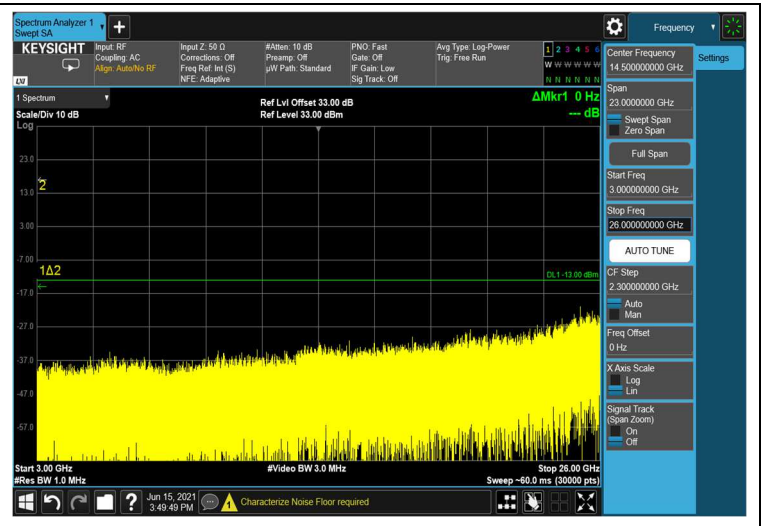
Figure 453: 3GHz-26GHz
