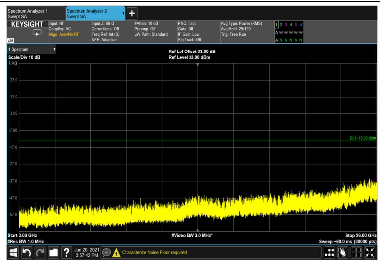
Figure 451: 3GHz-26GHz
