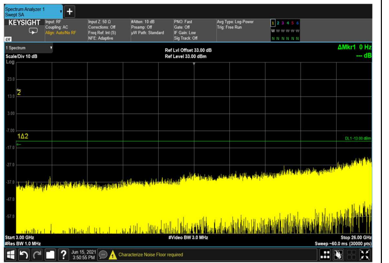
Figure 465: 3GHz-26GHz
