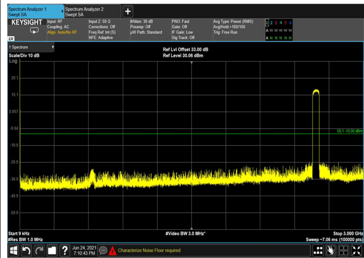
Figure 444: 9kHz-3GHz
