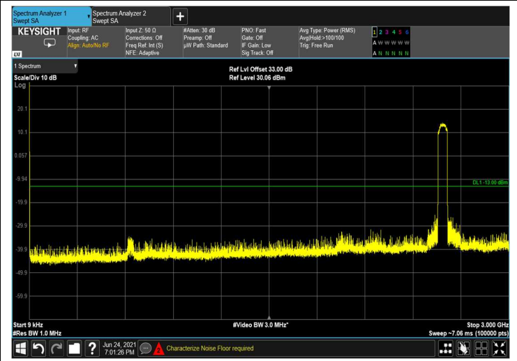
Figure 438: 9kHz-3GHz
