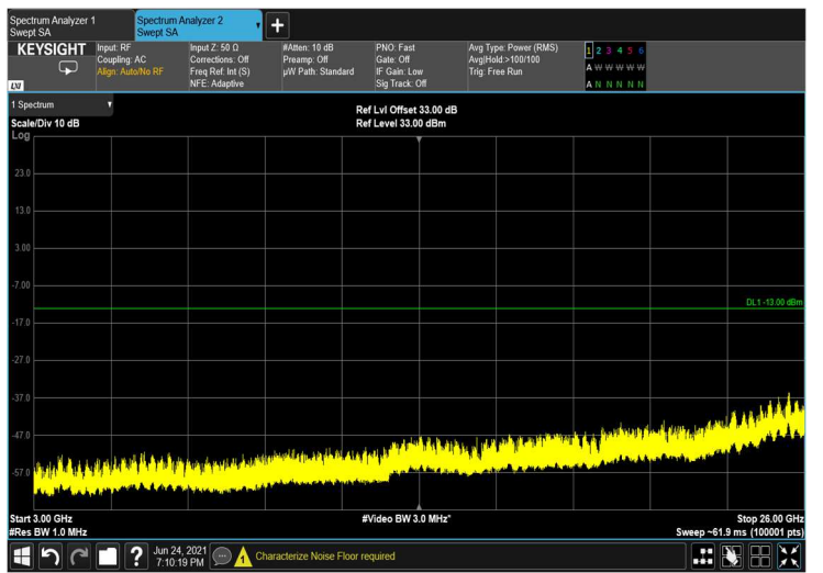
Figure 445: 3GHz-26GHz
