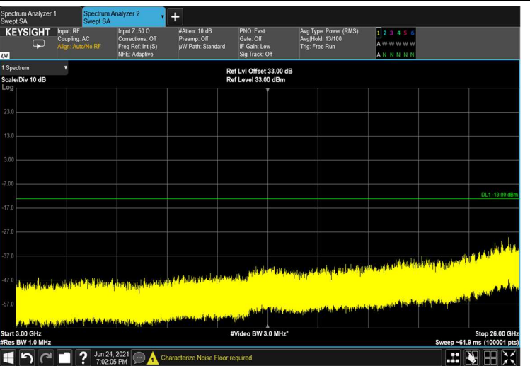
Figure 439: 3GHz-26GHz
