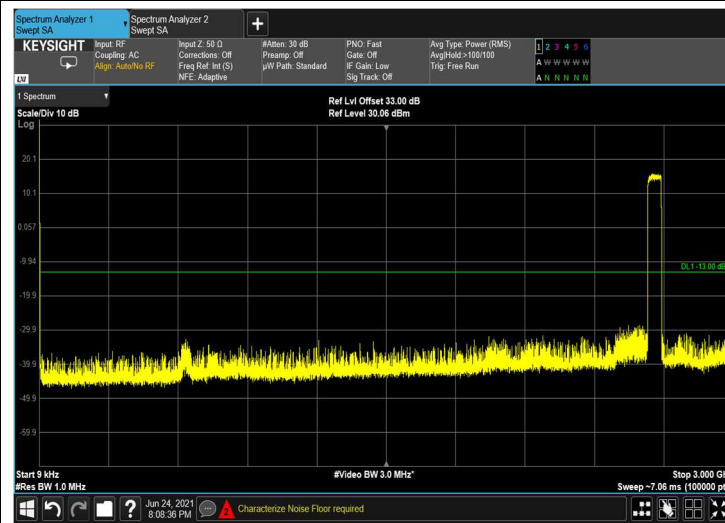
Spurious Emissions at Antenna Terminal QPSK 60MHz B.W.; 2660.0MHz, 30kHz
