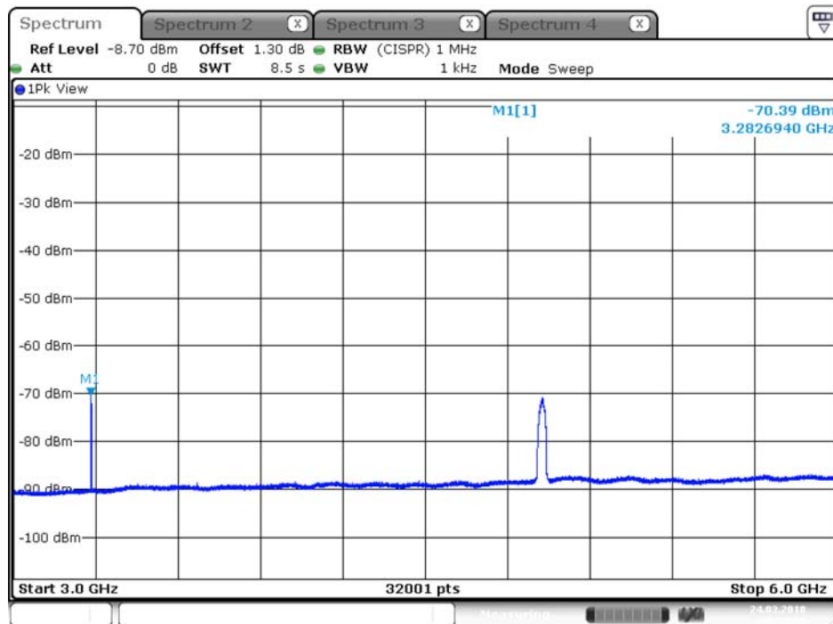
Plot on IEEE 802.11ac Nss1 MCS0 VHT20 / 2462 MHz / Average / Port 1 / 3GHz~6GHz
