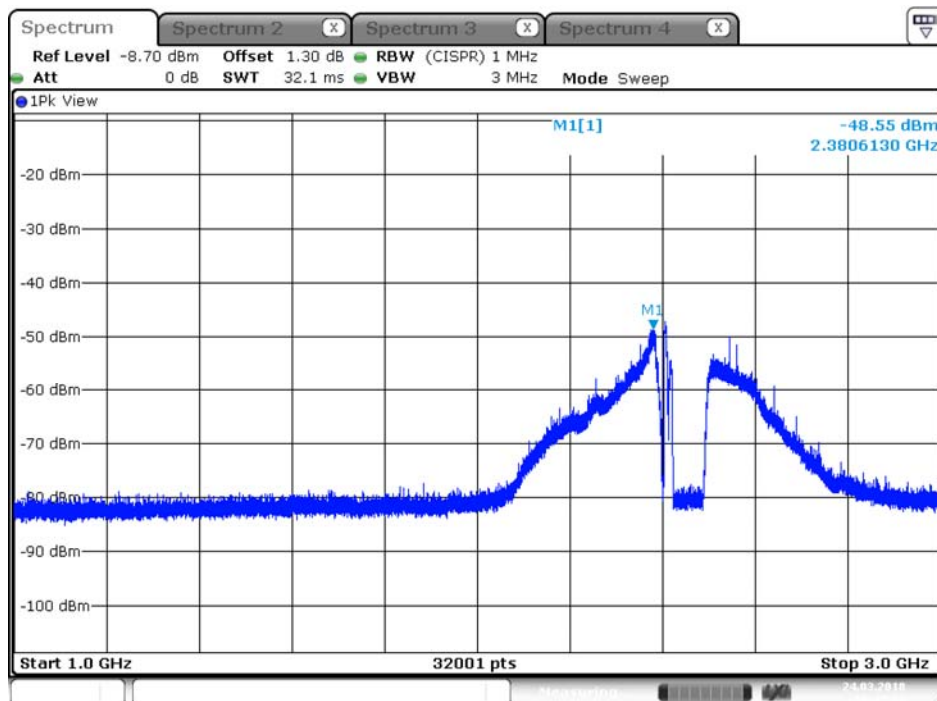
Plot on IEEE 802.11ac Nss1 MCS0 VHT20 / 2412 MHz / Peak / Port 1 / 1GHz~3GHz
