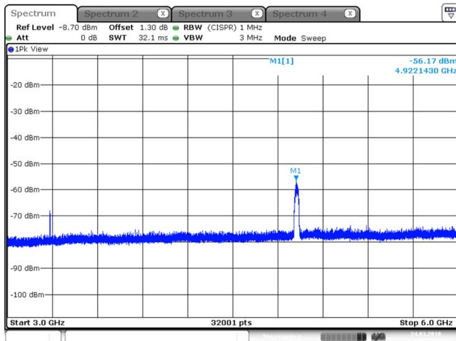
Plot on IEEE 802.11ac Nss1 MCS0 VHT20 / 2462 MHz / Peak / Port 1 / 3GHz~6GHz
