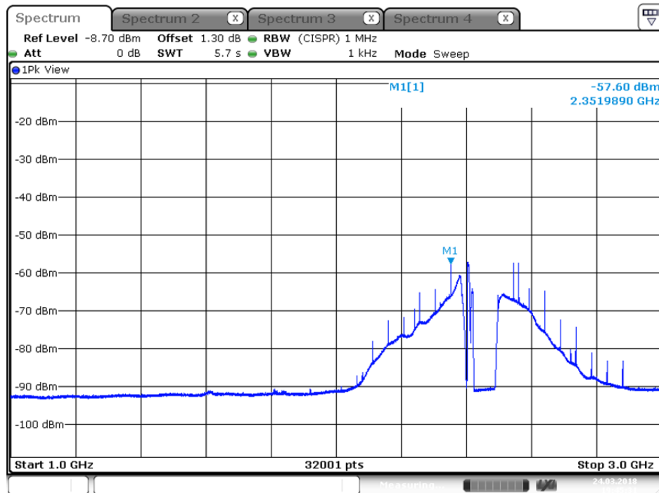
Plot on IEEE 802.11ac Nss1 MCS0 VHT20 / 2412 MHz / Average / Port 1 / 1GHz~3GHz
