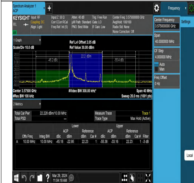
42(3550-3600)-10MHz-16QAM-43340-1RB#0-PASS
