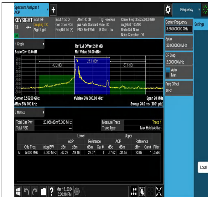
42(3550-3600)-5MHz-QPSK-43115-1RB#0-PASS
