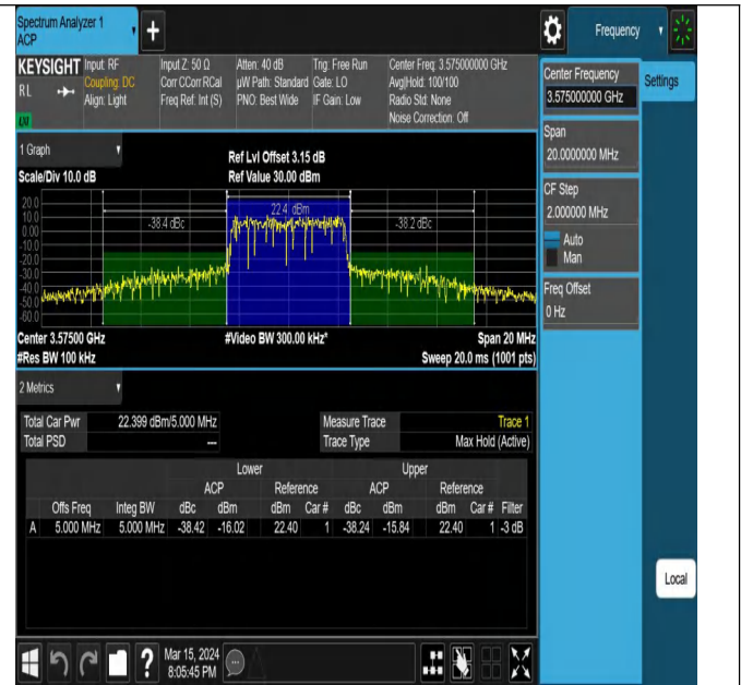
42(3550-3600)-5MHz-QPSK-43340-25RB#0-PASS
