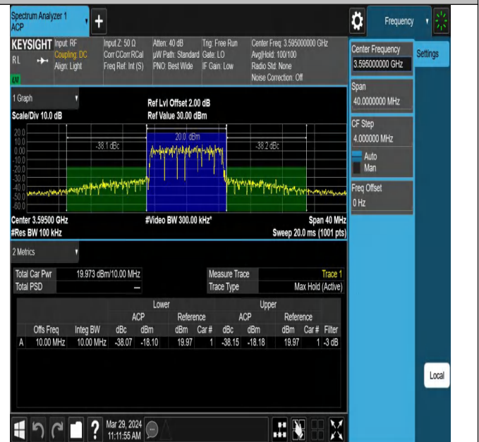
42(3550-3600)-10MHz-16QAM-43540-50RB#0-PASS
