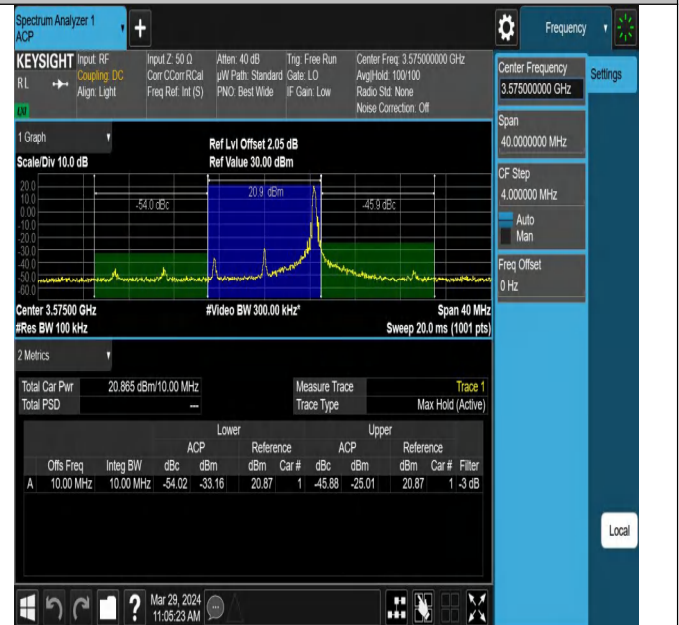
42(3550-3600)-10MHz-16QAM-43340-1RB#49-PASS
