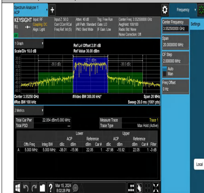
42(3550-3600)-5MHz-QPSK-43115-25RB#0-PASS
