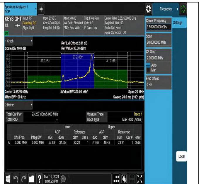
42(3550-3600)-5MHz-QPSK-43115-1RB#24-PASS
