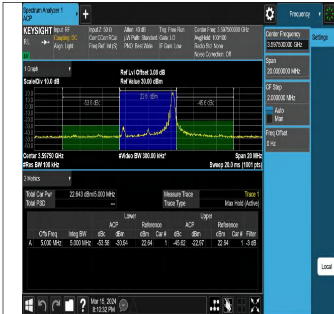
42(3550-3600)-5MHz-16QAM-43565-1RB#24-PASS
