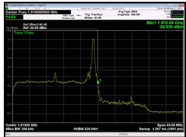
LTE Band 2 20MHz 64QAM 100%RB CH-High
