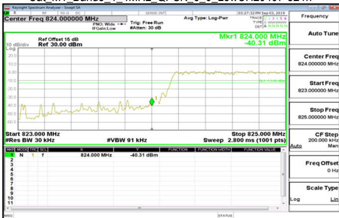
Cat M1_Band5_1_4MHz_QPSK_6_0_LowCH20407-824.7
