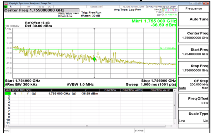
Cat_M1_Band4_20MHz_QPSK_1_5_HighCH20300-1745
