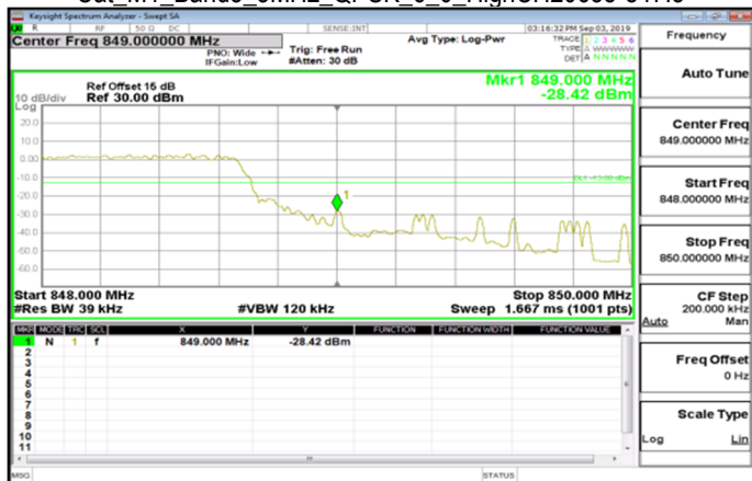
Cat_M1_Band5_3MHz_QPSK_6_0_HighCH20635-847.5
