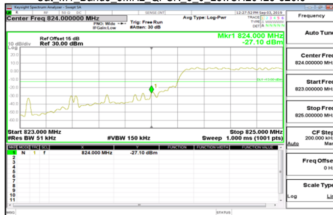
Cat_M1_Band5_5MHz_QPSK_6_0_LowCH20425-826.5
