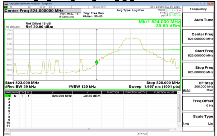
Cat M1_Band5_3MHz_QPSK_1_0_LowCH20415-825.5
