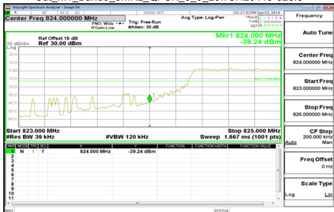
Cat_M1_Band5_3MHz_QPSK_6_0_LowCH20415-825.5
