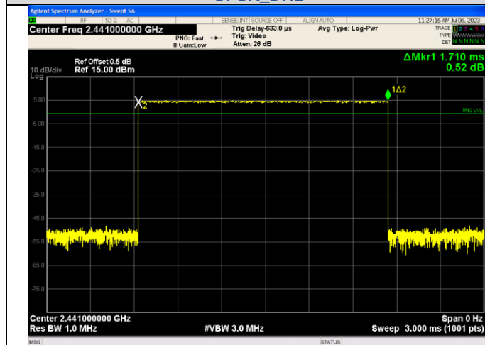
Pulse Width GFSK DH3
