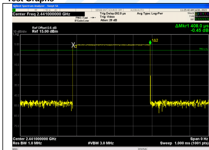
Pulse Width GFSK DH1
