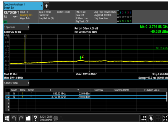
B2&B66_N5(10M)_DFT-s-OFDM_QPSK_Edge_1RB_Left_Mid_CH
