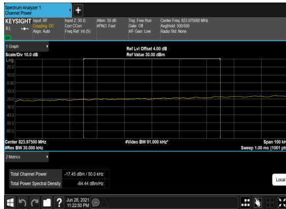
N5(5M)_DFT-s- OFDM_QPSK_Edge_1RB_Left_Low_CH_CHP_PA SS
