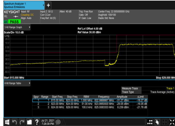
B2&B66_N5(5M)_DFT-s- OFDM_BPSK_Outer_Full_Low_CH
