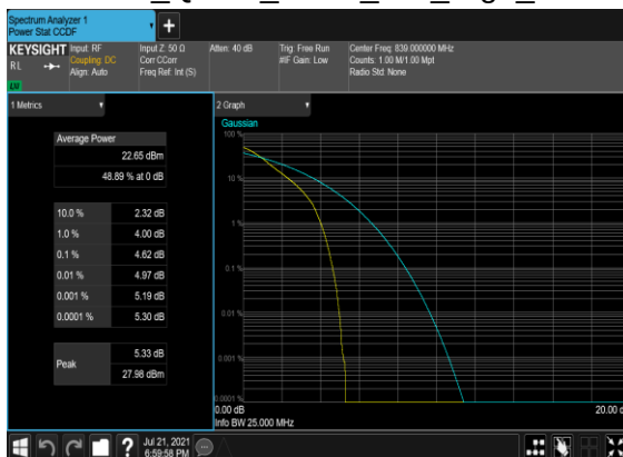
B2&B66_N5(20M)_DFT-s-OFDM_QPSK_Outer_Full_High_CH
