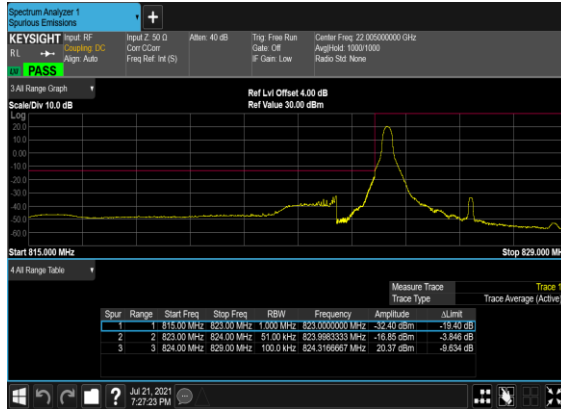
B2&B66_N5(5M)_DFT-s- OFDM_QPSK_Edge_1RB_Left_Low_CH
