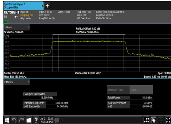
B2&B66_N5(15M)_DFT-s- OFDM_QPSK_Outer_Full_Mid_CH
