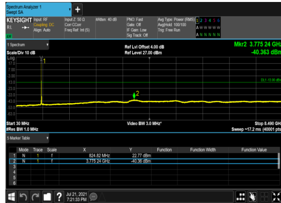
B2&B66_N5(20M)_DFT-s-OFDM_QPSK_Edge_1RB_Left_Low_CH
