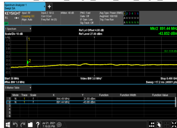
B2&B66_N5(5M)_DFT-s- OFDM_QPSK_Edge_1RB_Left_High_CH
