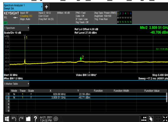
B2&B66_N5(20M)_DFT-s-OFDM_QPSK_Edge_1RB_Left_High_CH
