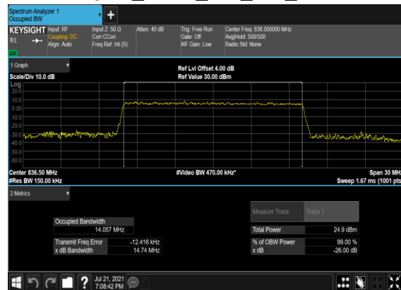
B2&B66_N5(15M)_CP-OFDM_256 QAM_Outer_Full_Mid_CH
