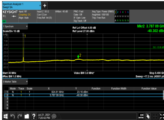
B2&B66_N5(20M)_DFT-s-OFDM_BPSK_Edge_1RB_Left_Low_CH
