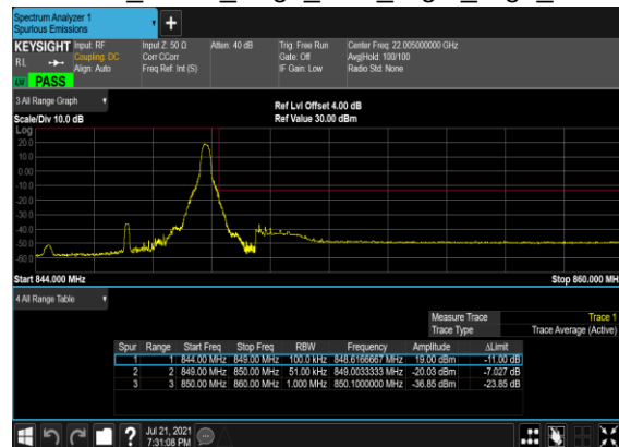
B2&B66_N5(5M)_DFT-s- OFDM_BPSK_Edge_1RB_Right_High_CH
