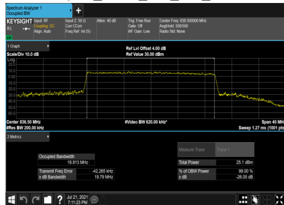
B2&B66_N5(20M)_CP-OFDM_256 QAM_Outer_Full_Mid_CH
