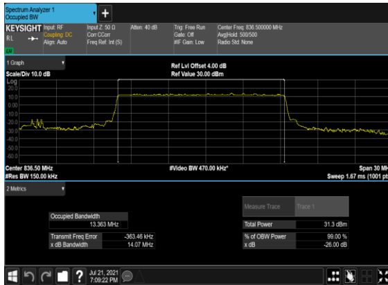
B2&B66_N5(20M)_DFT-s-OFDM_PI_2- BPSK_Outer_Full_Mid_CH
