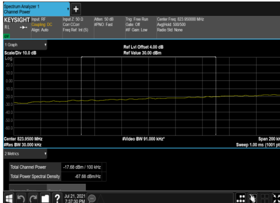
B2&B66_N5(10M)_DFT-s- OFDM_BPSK_Edge_1RB_Left_Low_CH_chp_ PASS
