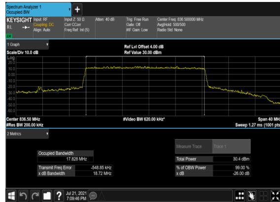
B2&B66_N5(20M)_DFT-s- OFDM_QPSK_Outer_Full_Mid_CH
