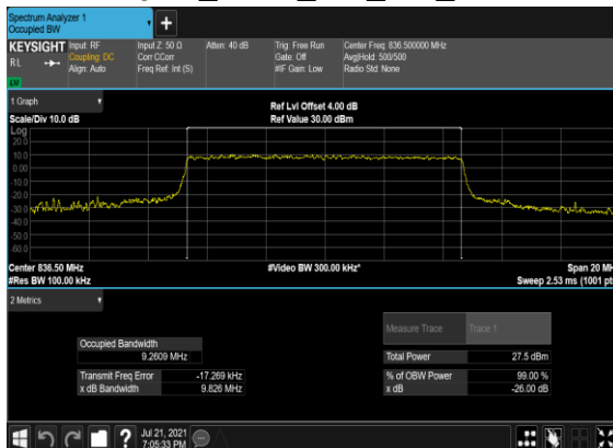
B2&B66_N5(10M)_CP-OFDM_64 QAM_Outer_Full_Mid_CH
