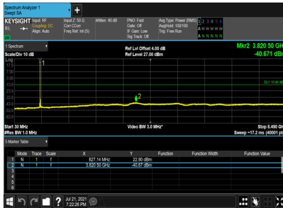
B2&B66_N5(20M)_DFT-s-OFDM_BPSK_Edge_1RB_Left_Mid_CH
