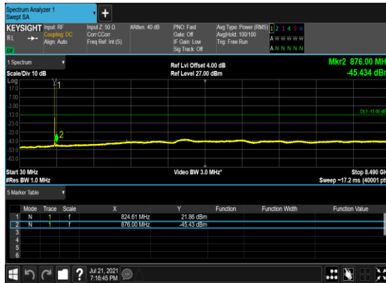
B2&B66_N5(10M)_DFT-s-OFDM_BPSK_Edge_1RB_Left_Low_CH
