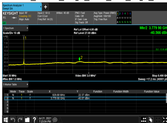
B2&B66_N5(20M)_DFT-s-OFDM_BPSK_Edge_1RB_Left_High_CH
