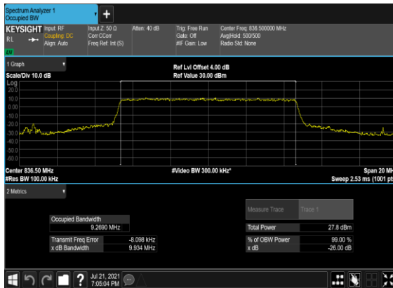
B2&B66_N5(10M)_CP- OFDM_QPSK_Outer_Full_Mid_CH
