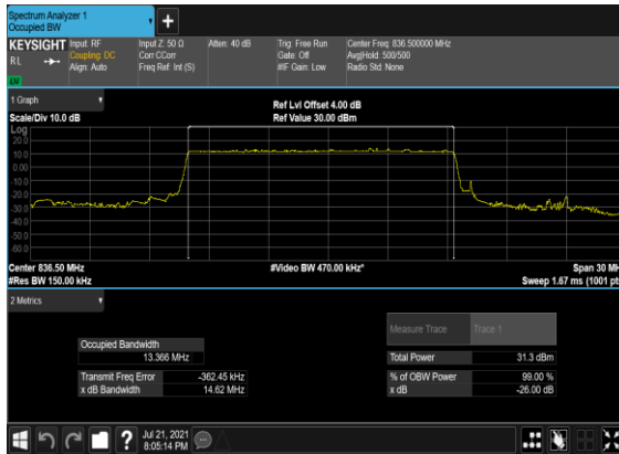
B2&B66_N5(15M)_DFT-s-OFDM_PI_2- BPSK_Outer_Full_Mid_CH
