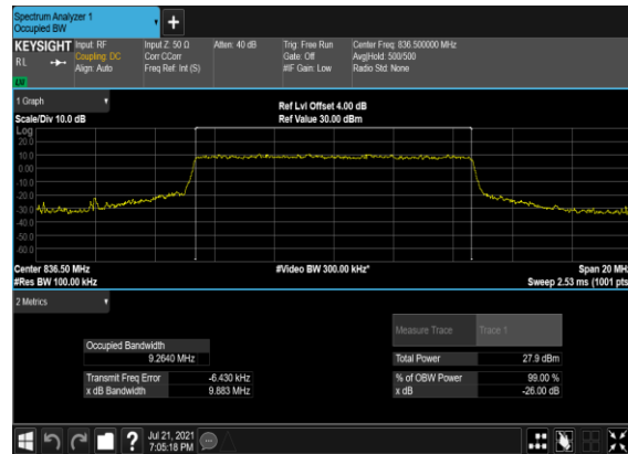
B2&B66_N5(10M)_CP-OFDM_16 QAM_Outer_Full_Mid_CH
