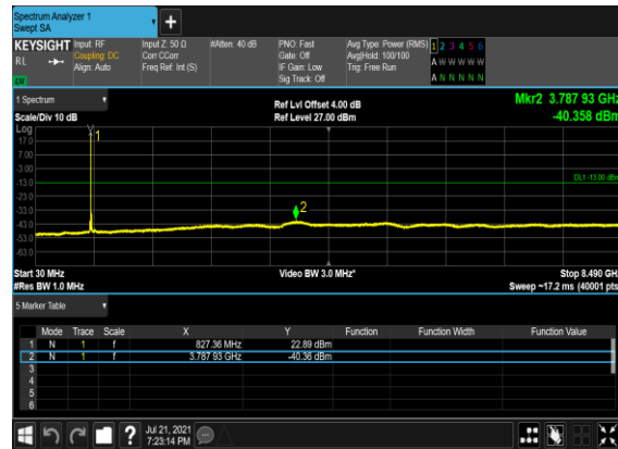
B2&B66_N5(20M)_DFT-s-OFDM_QPSK_Edge_1RB_Left_Mid_CH
