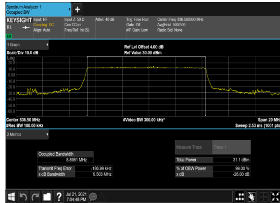
B2&B66_N5(10M)_DFT-s- OFDM_QPSK_Outer_Full_Mid_CH
