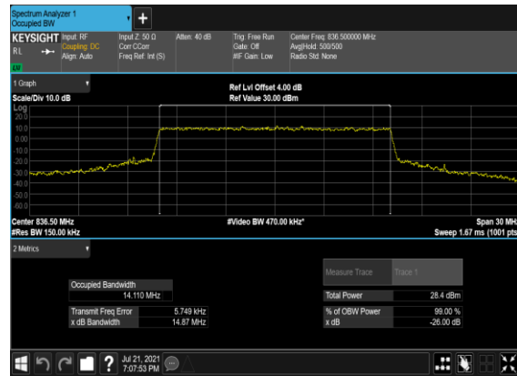
B2&B66_N5(15M)_CP-OFDM_16 QAM_Outer_Full_Mid_CH
