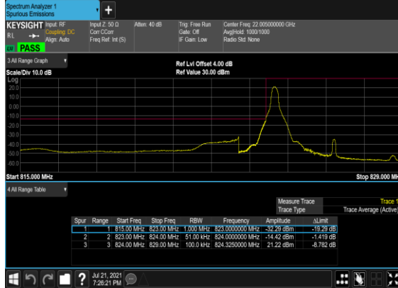
B2&B66_N5(5M)_DFT-s- OFDM_BPSK_Edge_1RB_Left_Low_CH
