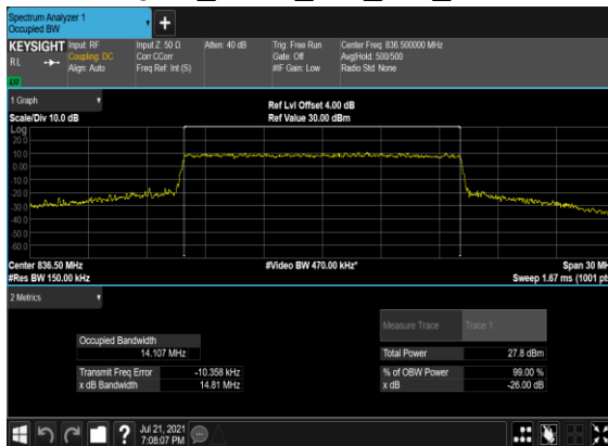
B2&B66_N5(15M)_CP-OFDM_64 QAM_Outer_Full_Mid_CH
