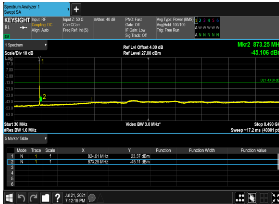
B2&B66_N5(5M)_DFT-s- OFDM_BPSK_Edge_1RB_Left_Low_CH
