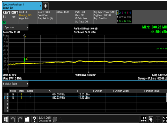
B2&B66_N5(5M)_DFT-s- OFDM_BPSK_Edge_1RB_Left_Mid_CH
