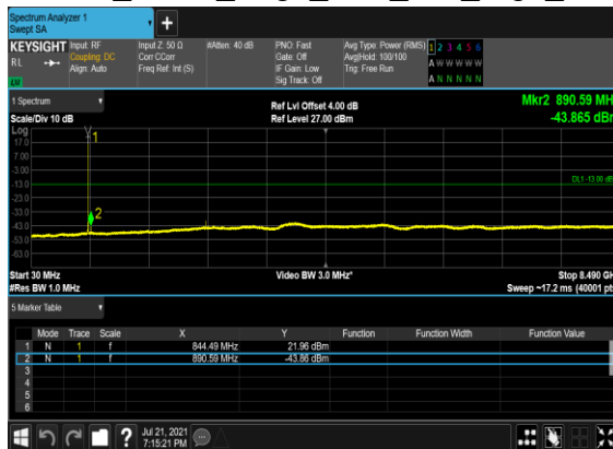
B2&B66_N5(5M)_DFT-s- OFDM_BPSK_Edge_1RB_Left_High_CH
