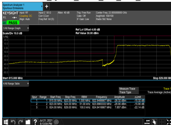
B2&B66_N5(5M)_DFT-s- OFDM_QPSK_Outer_Full_Low_CH
