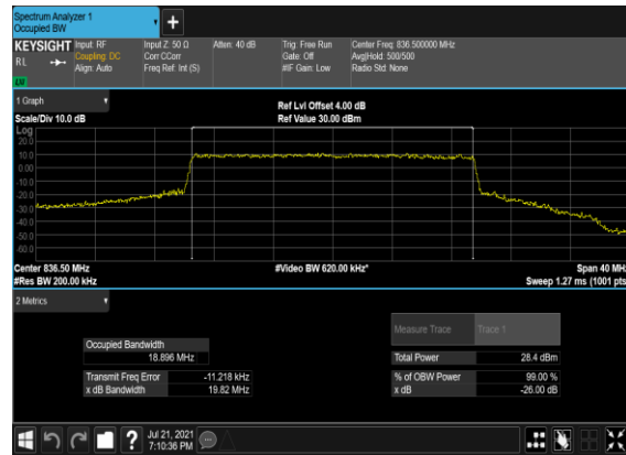
B2&B66_N5(20M)_CP-OFDM_16 QAM_Outer_Full_Mid_CH
