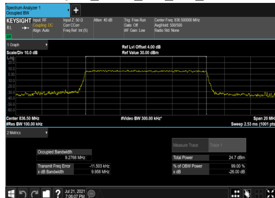
B2&B66_N5(10M)_CP-OFDM_256 QAM_Outer_Full_Mid_CH
