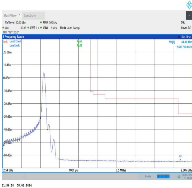
15MHz-15MHz_QPSK@QPSK-QPSK@QPSK_21225-21375_1 RB#74@75RB#0-0RB#0@75RB#0
