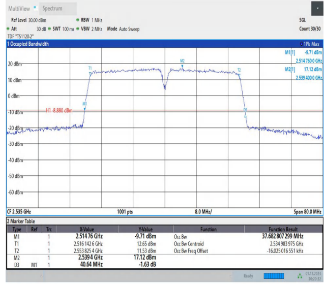
7-7-20MHz-20MHz-QPSK-QPSK-21001-21199-100RB#0-100 RB#0-PASS
