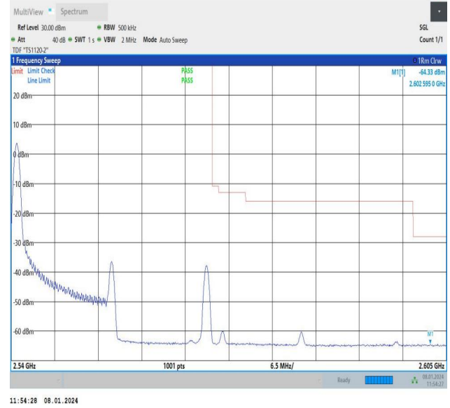
15MHz-15MHz_16QAM@16QAM-16QAM@16QAM_21225-21375_1 RB#0@75RB#0-0RB#0@75RB#0
