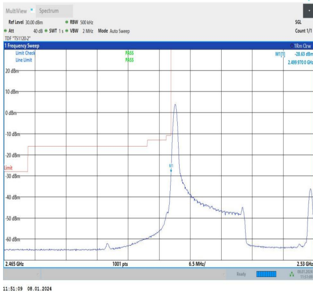
15MHz-15MHz_QPSK@QPSK-QPSK@QPSK_20825-20975_1 RB#0@75RB#0-0RB#0@75RB#0
