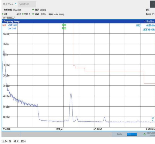
15MHz-15MHz_QPSK@QPSK-QPSK@QPSK_21225-21375_1 RB#0@75RB#0-0RB#0@75RB#0
