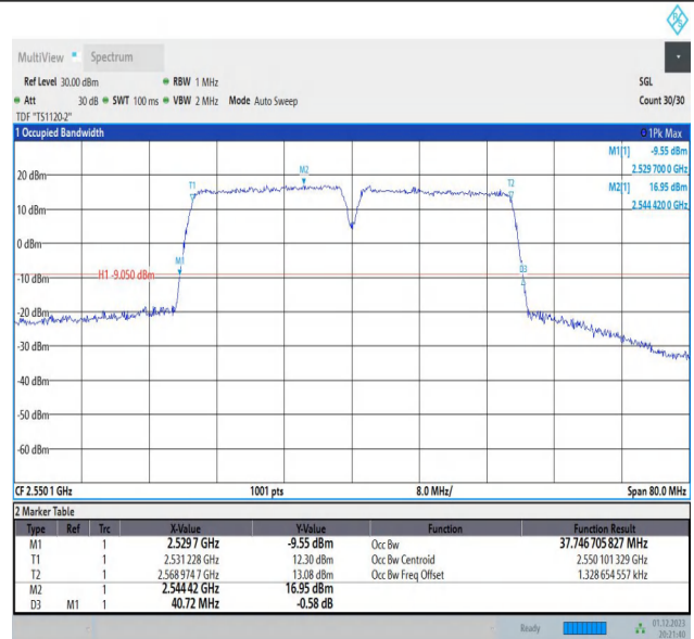
7-7-20MHz-20MHz-QPSK-QPSK-21001-21199-100RB#0-100 RB#0-PASS
