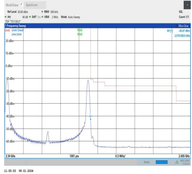
15MHz-15MHz_16QAM@16QAM-16QAM@16QAM_21225-21375_1RB#0@75RB#0-1RB#74@75RB#0
