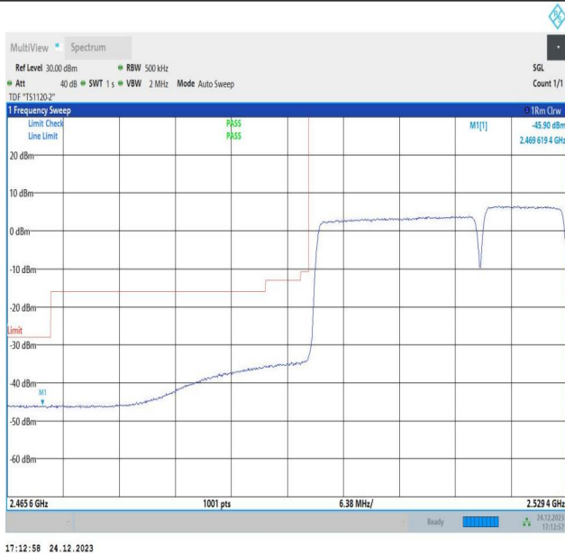
20MHz-10MHz_16QAM@16QAM-16QAM@16QAM_20850-20994_100RB#0@100RB#0-50RB#0@50RB#0
