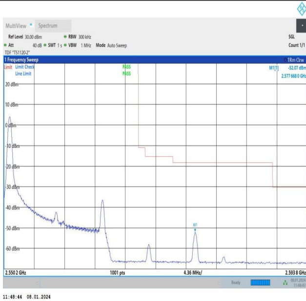
15MHz-5MHz_QPSK@QPSK-QPSK@QPSK_21327-21420_1 RB#0@75RB#0-0RB#0@25RB#0
