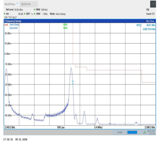
15MHz-10MHz_16QAM@16QAM-16QAM@16QAM_21277-21397_1 RB#0@75RB#0-1RB#49@50RB#0
