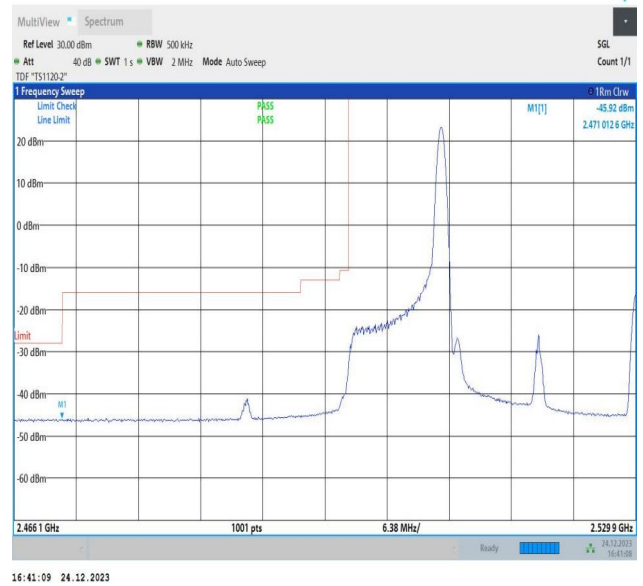
10MHz-20MHz_QPSK@QPSK-QPSK@QPSK_20805-20949_1RB#49@50RB#0-0RB#0@100RB#0
