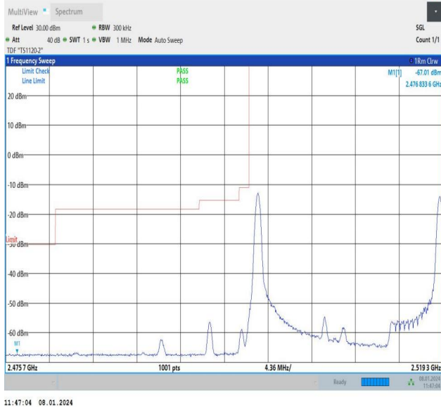
15MHz-5MHz_QPSK@QPSK-QPSK@QPSK_20825-20918_1 RB#0@75RB#0-1RB#24@25RB#0
