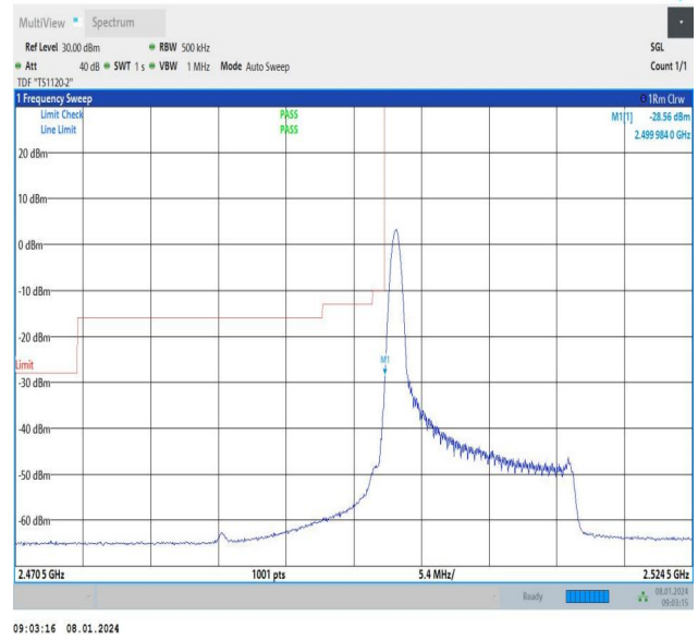
15MHz-10MHz_16QAM@16QAM-16QAM@16QAM_20825-20945_1 RB#0@75RB#0-0RB#0@50RB#0
