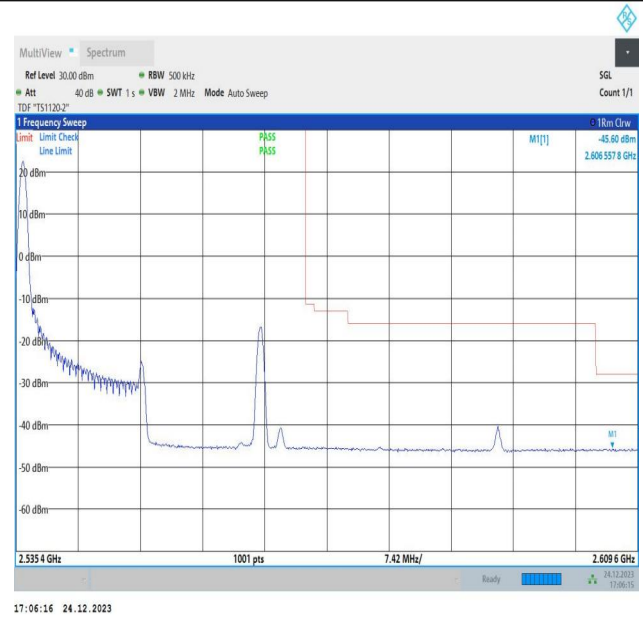
15MHz-20MHz_16QAM@16QAM-16QAM@16QAM_21179-21350_1RB#0@75RB#0-0RB#0@100RB#0
