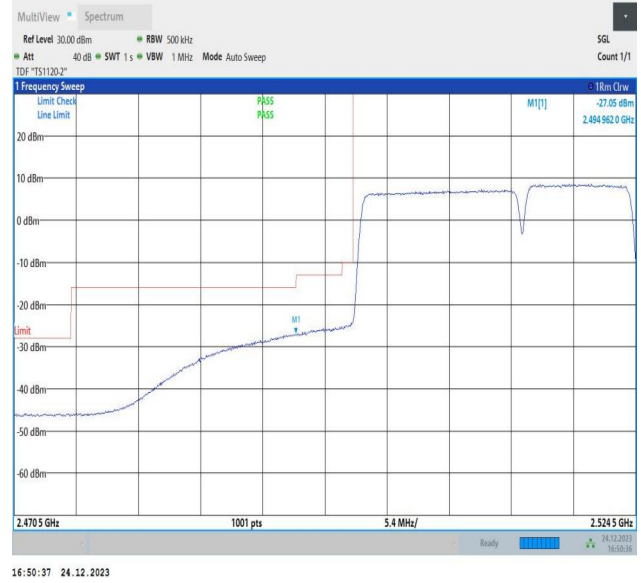
15MHz-10MHz_QPSK@QPSK-QPSK@QPSK_20825-20945_75RB#0@75RB#0-50RB#0@50RB#0
