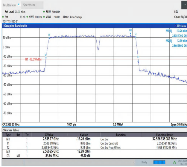
7-7-20MHz-15MHz-64QAM-64QAM-21201-21372-100RB#0-7 5RB#0-PASS
