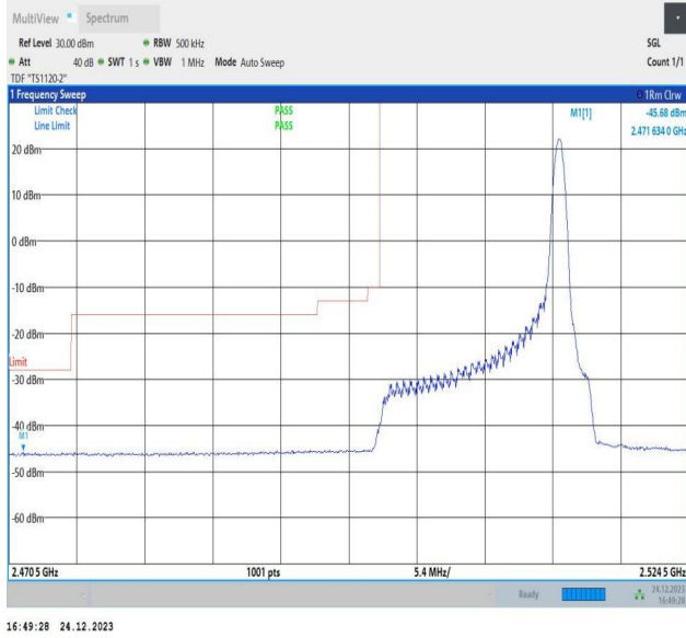
15MHz-10MHz_16QAM@16QAM-16QAM@16QAM_20825-20945_1RB#74@75RB#0-0RB#0@50RB#0
