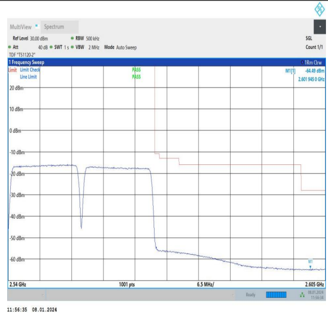
15MHz-15MHz_16QAM@16QAM-16QAM@16QAM_21225-21375_75RB#0@75RB#0-75RB#0@75RB#0
