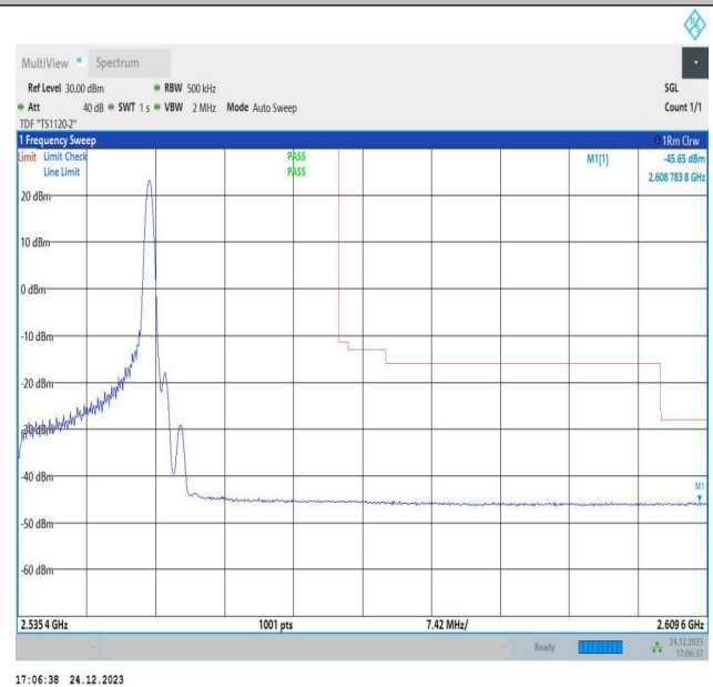
15MHz-20MHz_QPSK@QPSK-QPSK@QPSK_21179-21350_1RB#74@75RB#0-0RB#0@100RB#0
