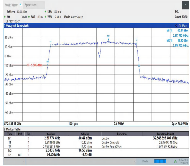
7-7-20MHz-15MHz-QPSK-QPSK-21026-21197-100RB#0-75R B#0-PASS
