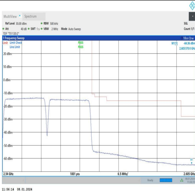
15MHz-15MHz_QPSK@QPSK-QPSK@QPSK_21225-21375_7 5RB#0@75RB#0-75RB#0@75RB#0
