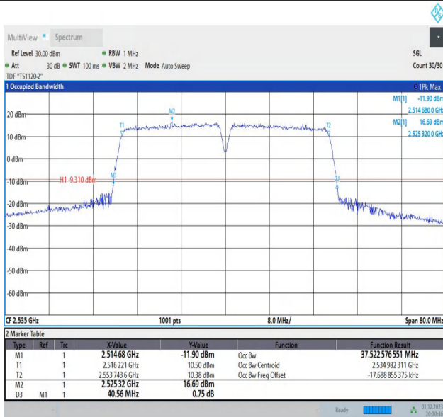
7-7-20MHz-15MHz-64QAM-64QAM-21201-21372-100RB#0-7 5RB#0-PASS
