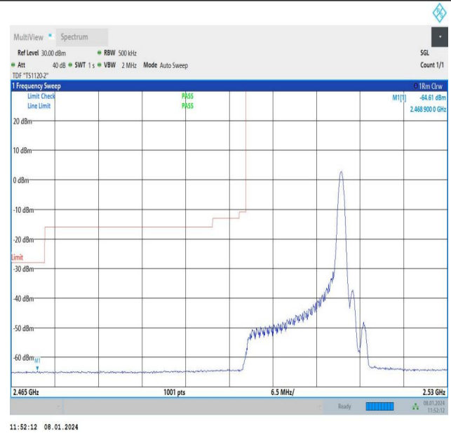
15MHz-15MHz_16QAM@16QAM-16QAM@16QAM_20825-20975_1 RB#74@75RB#0-0RB#0@75RB#0
