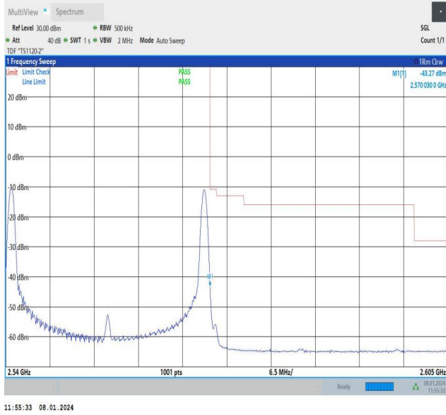
15MHz-15MHz_QPSK@QPSK-QPSK@QPSK_21225-21375_1 RB#0@75RB#0-1RB#74@75RB#0
