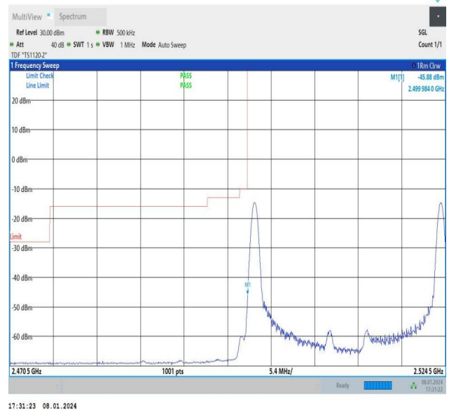
15MHz-10MHz_16QAM@16QAM-16QAM@16QAM_20825-20945_1RB#0@75RB#0-1RB#49@50RB#0
