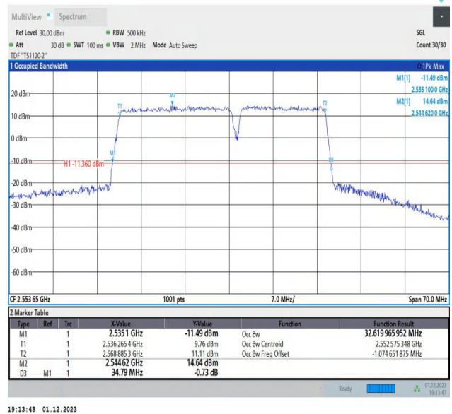
7-7-20MHz-15MHz-QPSK-QPSK-21201-21372-100RB#0-75R B#0-PASS
