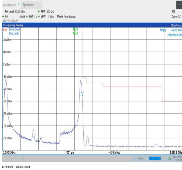
15MHz-5MHz_QPSK@QPSK-QPSK@QPSK_21327-21420_1 RB#0@75RB#0-1RB#24@25RB#0
