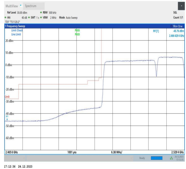
20MHz-10MHz_QPSK@QPSK-QPSK@QPSK_20850-20994_100RB#0@100RB#0-50RB#0@50RB#0
