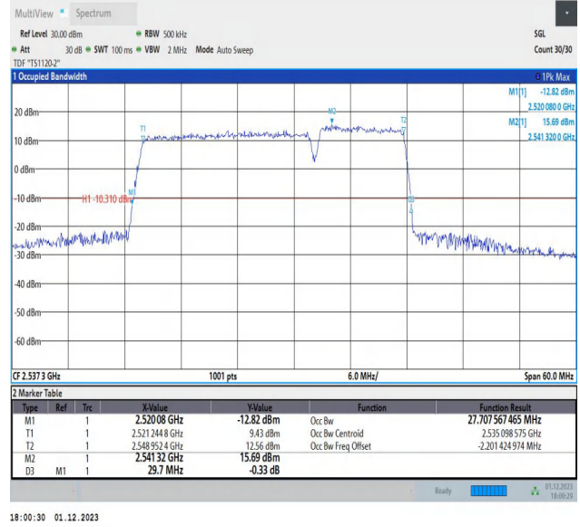
7-7-20MHz-10MHz-16QAM-16QAM-21051-21195-100RB#0-50 RB#0-PASS
