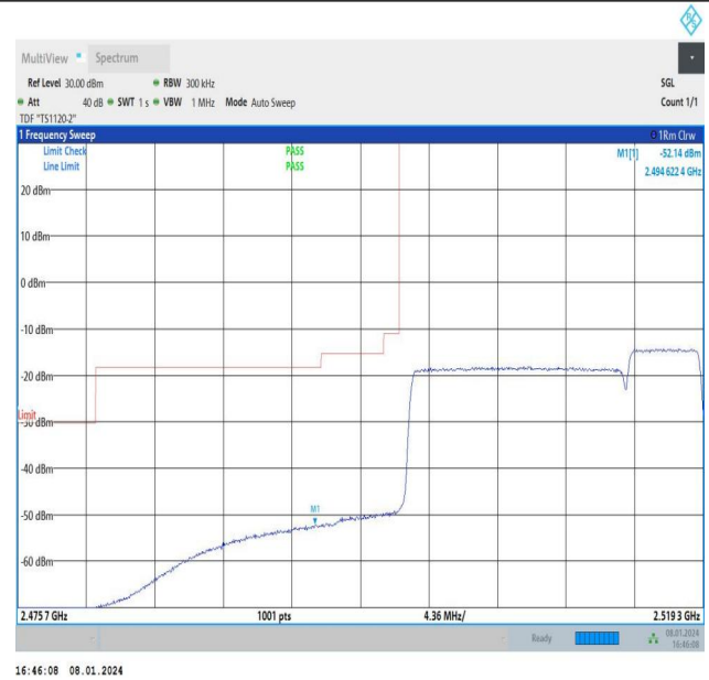
15MHz-5MHz_QPSK@QPSK-QPSK@QPSK_20825-20918_75RB#0@75RB#0-25RB#0@25RB#0
