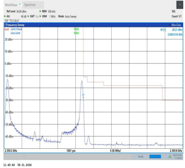
15MHz-5MHz_16QAM@16QAM-16QAM@16QAM_21327-21420_1RB#0@75RB#0-1RB#24@25RB#0
