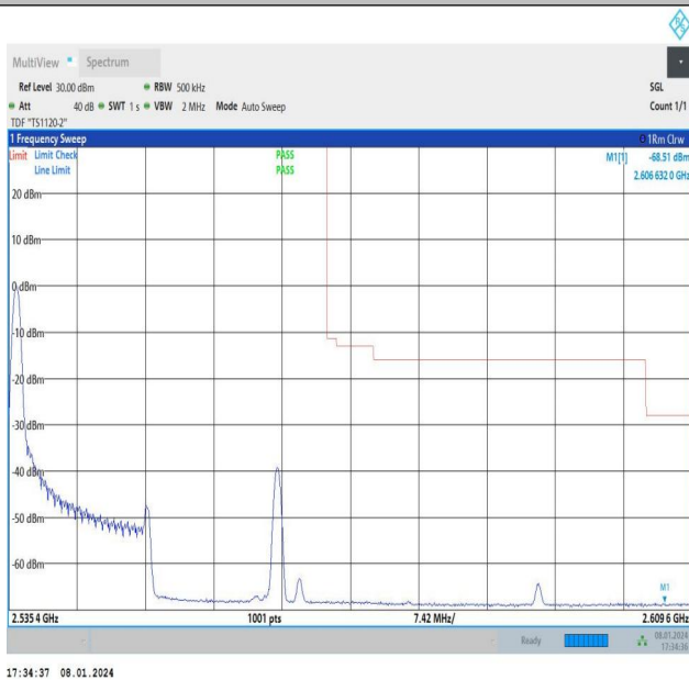
15MHz-20MHz_QPSK@QPSK-QPSK@QPSK_21179-21350_1RB#0@75RB#0-0RB#0@100RB#0
