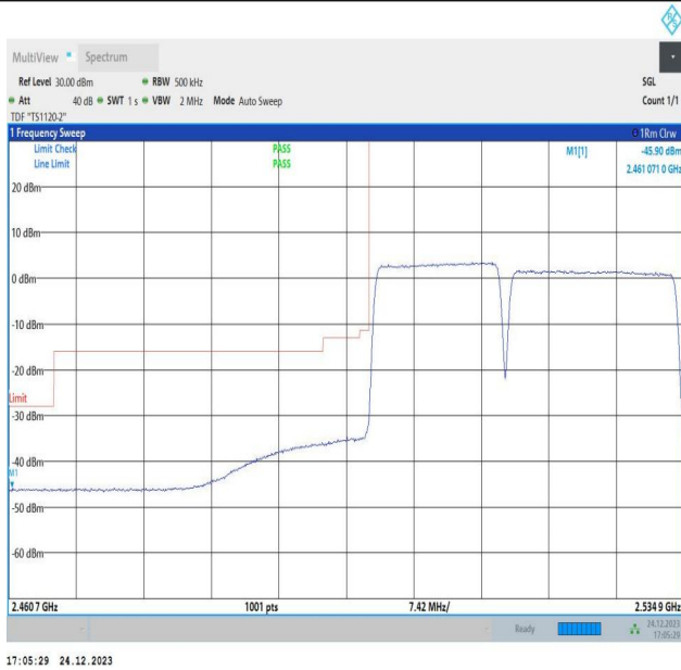
15MHz-20MHz_16QAM@16QAM-16QAM@16QAM_20828-20999_75RB#0@75RB#0-100RB#0@100RB#0
