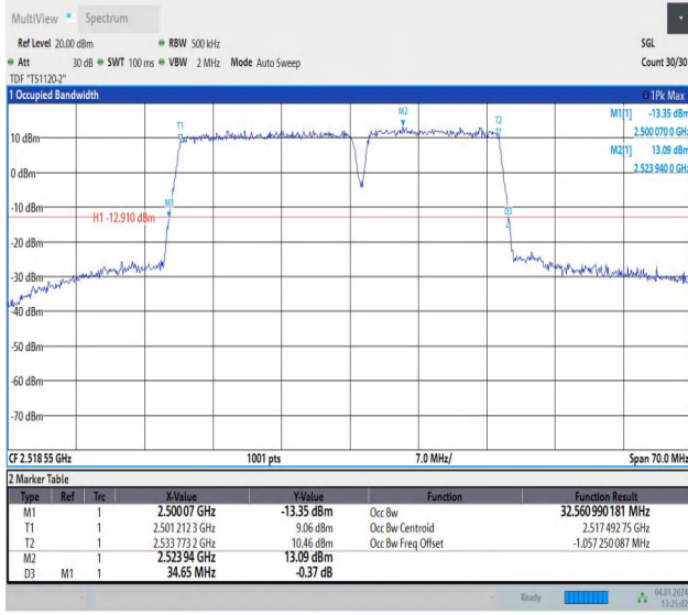
7-7-20MHz-15MHz-64QAM-64QAM-20850-21021-100RB#0-7 5RB#0-PASS
