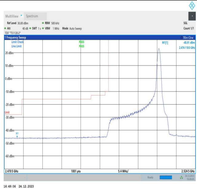
15MHz-10MHz_QPSK@QPSK-QPSK@QPSK_20825-20945_1 RB#74@75RB#0-0RB#0@50RB#0
