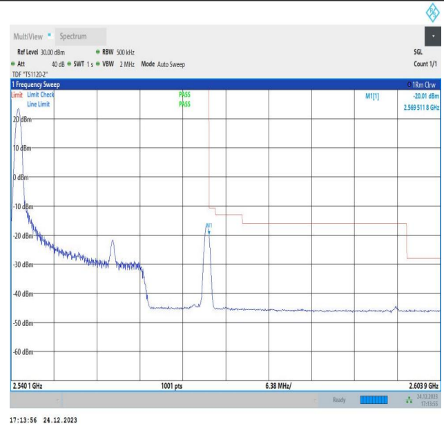
20MHz-10MHz_QPSK@QPSK-QPSK@QPSK_21251-21395_1RB#0@100RB#0-0RB#0@50RB#0
