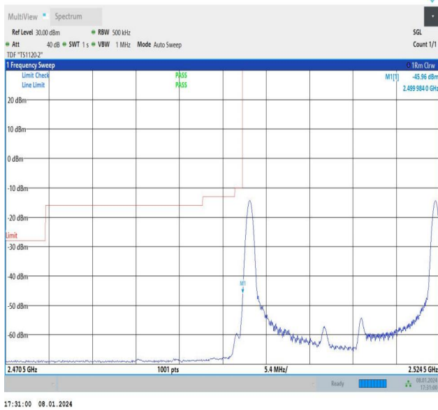
15MHz-10MHz_QPSK@QPSK-QPSK@QPSK_20825-20945_1RB#0@75RB#0-1RB#49@50RB#0
