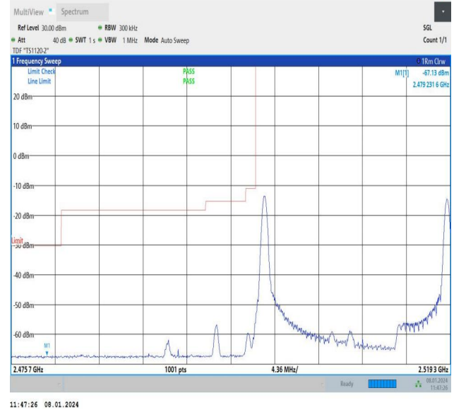
15MHz-5MHz_16QAM@16QAM-16QAM@16QAM_20825-20918_1 RB#0@75RB#0-1RB#24@25RB#0
