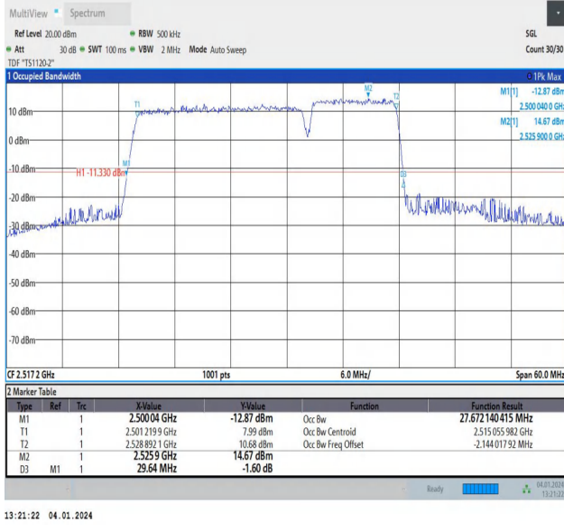
7-7-20MHz-10MHz-64QAM-64QAM-20850-20994-100RB#0-5 ORB#0-PASS
