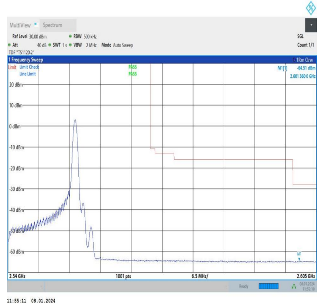
15MHz-15MHz_16QAM@16QAM-16QAM@16QAM_21225-21375_1 RB#74@75RB#0-0RB#0@75RB#0
