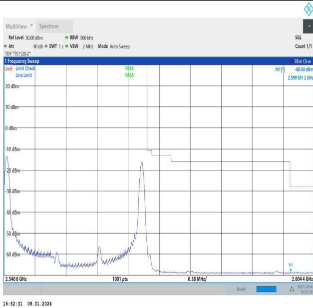
10MHz-20MHz_16QAM@16QAM-16QAM@16QAM_21206-21350_1 RB#0@50RB#0-1RB#99@100RB#0
