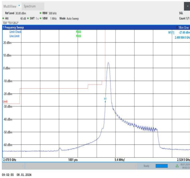
15MHz-10MHz_QPSK@QPSK-QPSK@QPSK_20825-20945_1 RB#0@75RB#0-0RB#0@50RB#0
