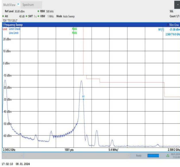
15MHz-10MHz_QPSK@QPSK-QPSK@QPSK_21277-21397_1 RB#0@75RB#0-1RB#49@50RB#0
