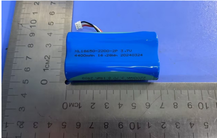
Photo 15 Appearance of Battery
