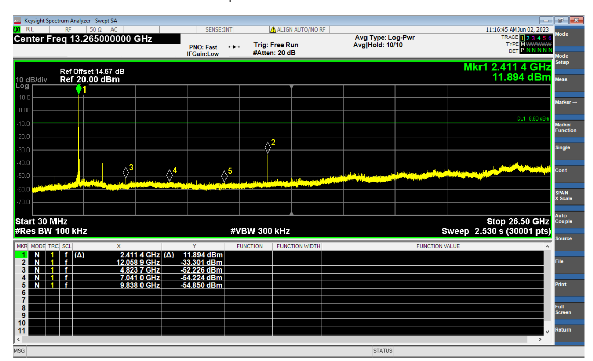
Tx. Spurious NVNT 2412MHz Emission
