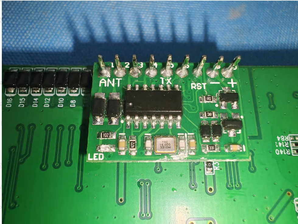
WiFi-ANT
