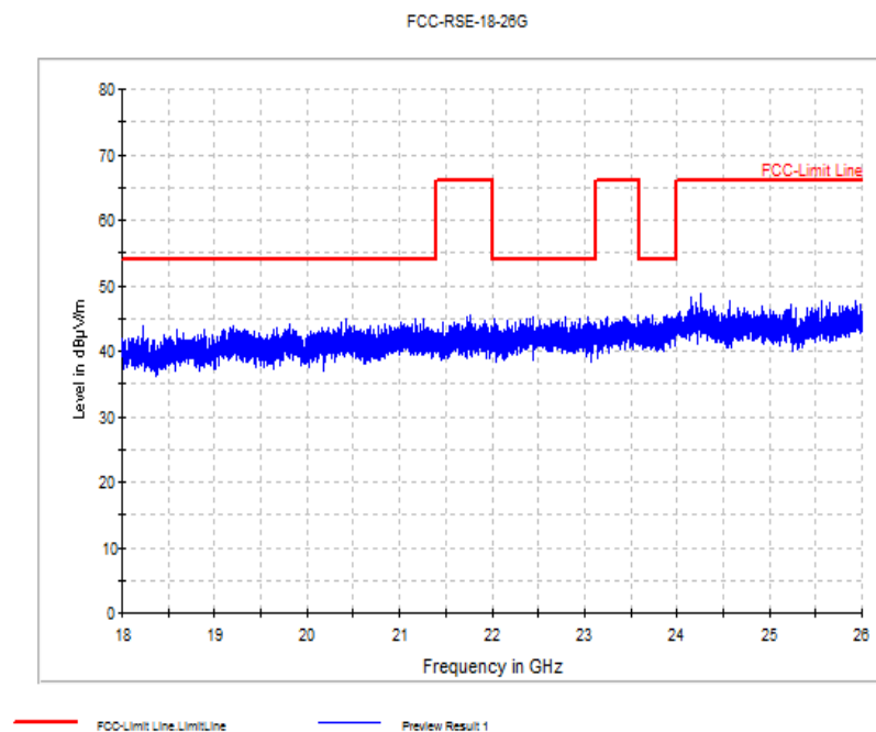
Fig. 86 Radiated emission: 18 GHz - 26 GHz
