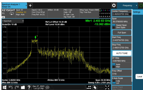
11AX20SISO-Ant1-2462-26Tone-RU0-PASS
