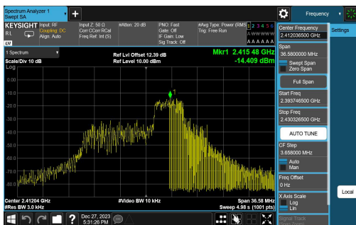
11AX20SISO-Ant1-2412-106Tone-RU53-PASS
