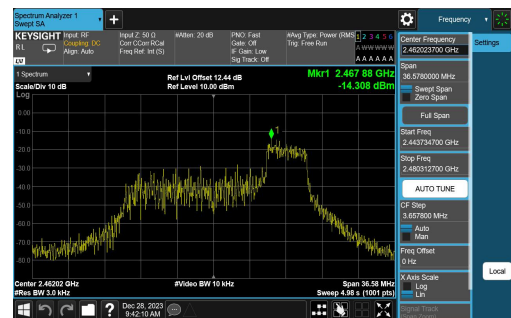
11AX20SISO-Ant1-2462-106Tone-RU54-PASS
