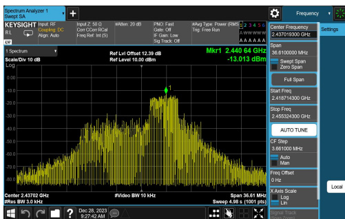
11AX20SISO-Ant1-2437-106Tone-RU53-PASS
