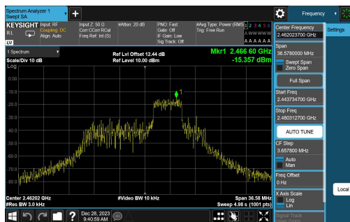
11AX20SISO-Ant1-2462-106Tone-RU53-PASS
