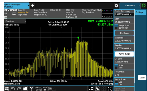
11AX20SISO-Ant1-2412-106Tone-RU54-PASS
