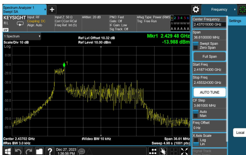
11AX20SISO-Ant1-2437-26Tone-RU0-PASS
