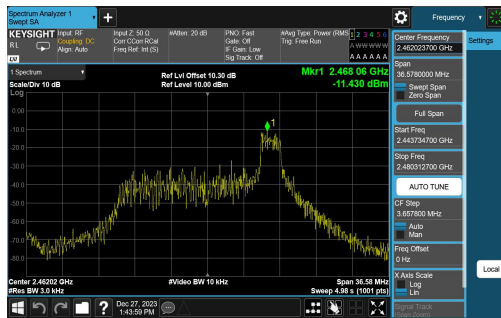
11AX20SISO-Ant1-2462-52Tone-RU39-PASS
