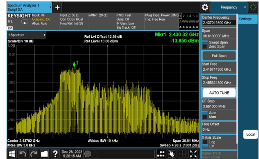
11AX20SISO-Ant1-2437-52Tone-RU40-PASS
