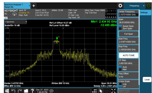
11AX20SISO-Ant1-2437-26Tone-RU4-PASS
