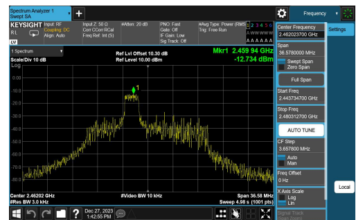
11AX20SISO-Ant1-2462-26Tone-RU4-PASS
