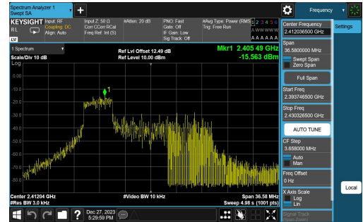
11AX20SISO-Ant1-2412-52Tone-RU40-PASS
