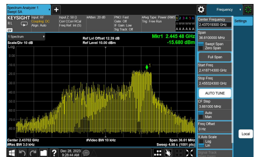
11AX20SISO-Ant1-2437-106Tone-RU54-PASS
