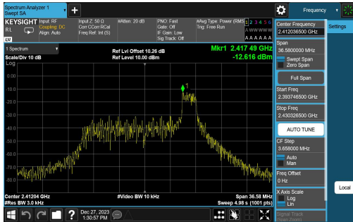
11AX20SISO-Ant1-2412-52Tone-RU39-PASS
