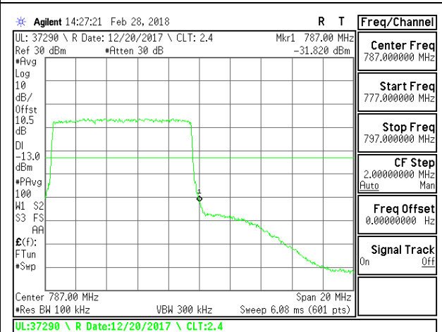
LTE B13 10MHz QPSK High Channel RB50-0
