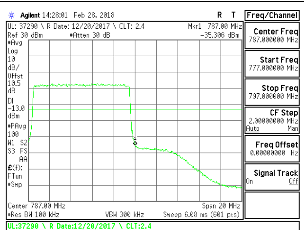
LTE B13 10MHz 16QAM High Channel RB50-0
