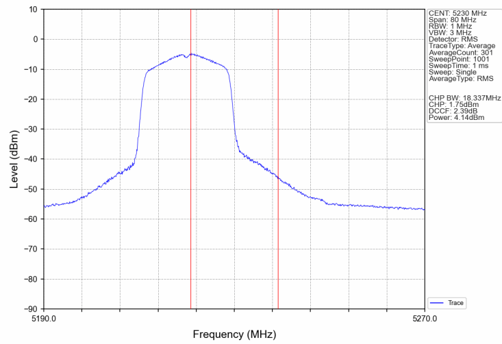
802.11ax(HEW40)_HCH_5230MHz_SU_Ant2_NTNV
