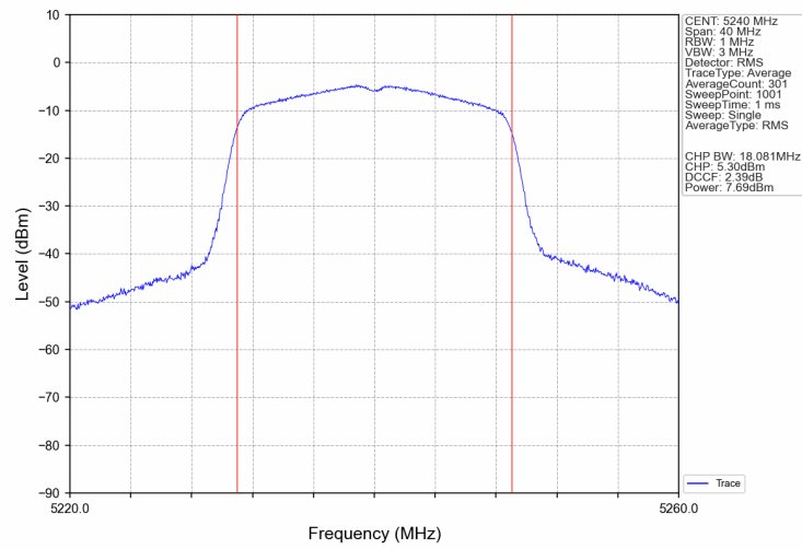
802.11ax(HEW20)_HCH_5240MHz_SU_Ant2_NTNV
