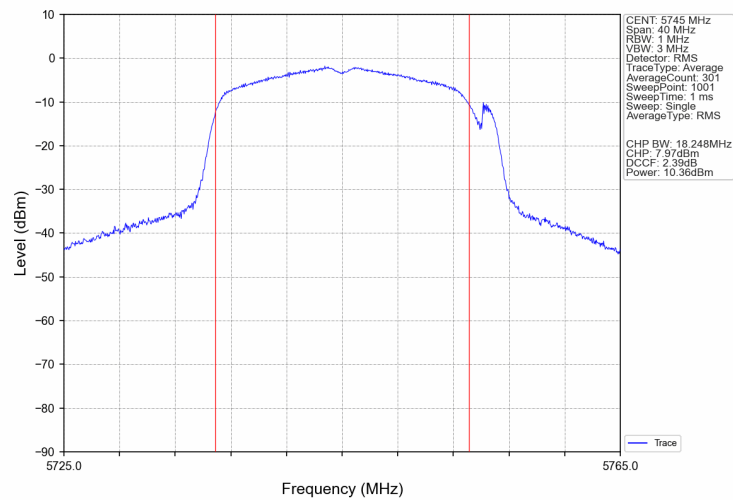
802.11ax(HEW20)_LCH_5745MHz_SU_Ant2_NTNV
