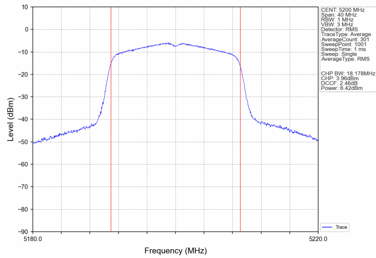
802.11ax(HEW20)_MCH_5200MHz_SU_Ant2_NTNV
