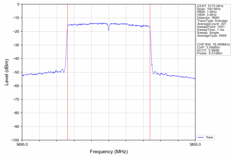
802.11ac(VHT80)_MCH_5775MHz_Ant2_NTNV
