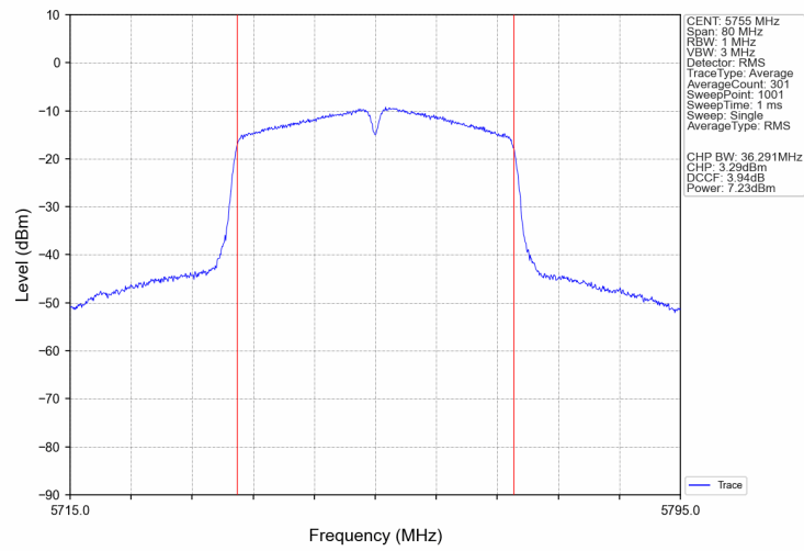
802.11ax(HEW40)_LCH_5755MHz_SU_Ant2_NTNV
