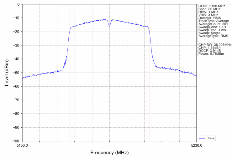
802.11ax(HEW40)_LCH_5190MHz_SU_Ant2_NTNV
