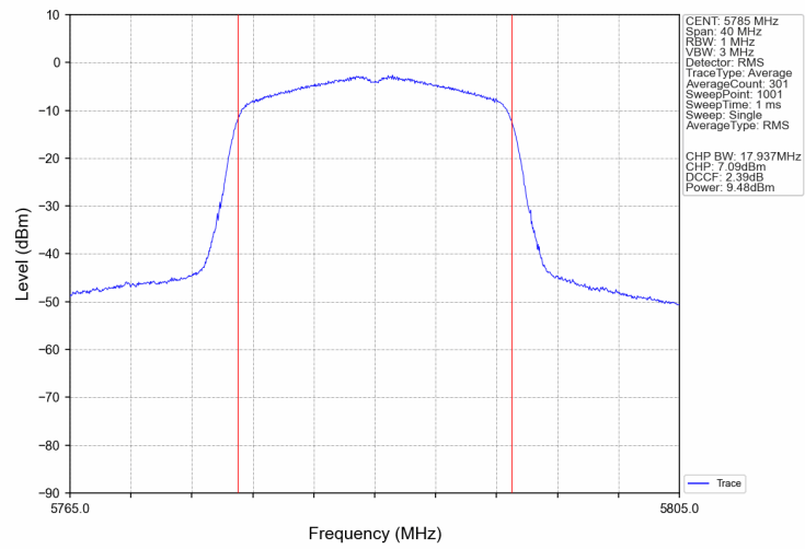
802.11ac(VHT20)_MCH_5785MHz_Ant2_NTNV
