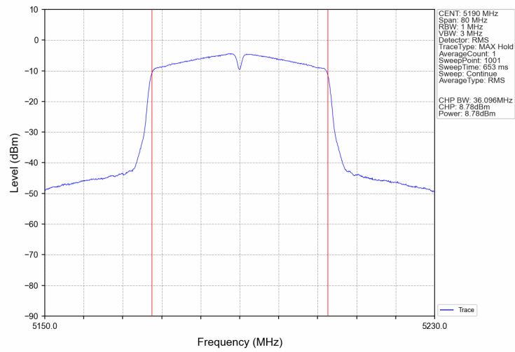
802.11ac(VHT40)_LCH_5190MHz_Ant2_NTNV
