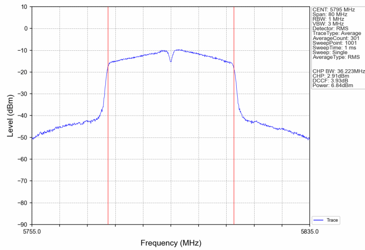
802.11ax(HEW40)_HCH_5795MHz_SU_Ant2_NTNV
