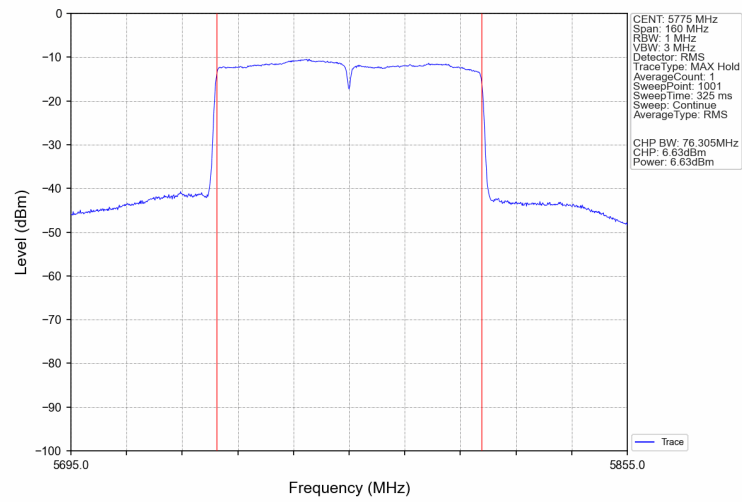
802.11ax(HEW80)_MCH_5775MHz_SU_Ant2_NTNV
