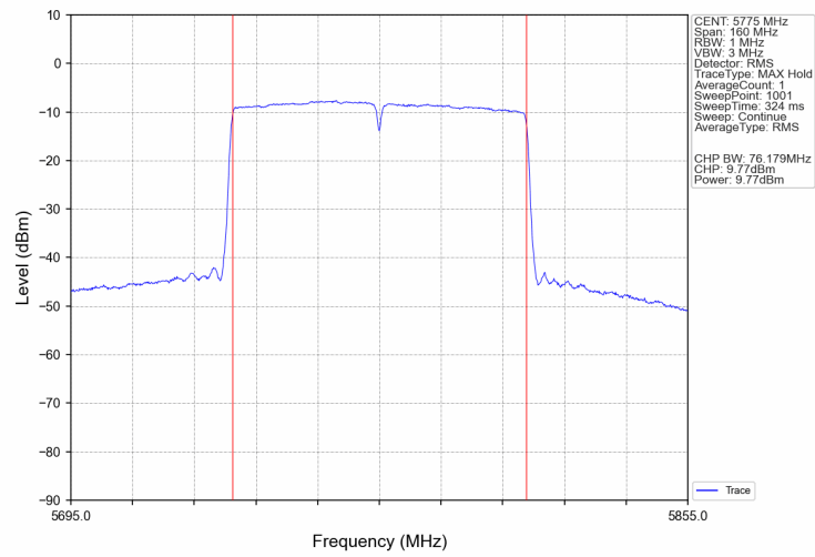
802.11ac(VHT80)_MCH_5775MHz_Ant2_NTNV
