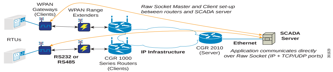
Figure 5-4 Raw Socket Client/Server Setup between Routers and SCADA Server with Direct RAW Socket Communication
