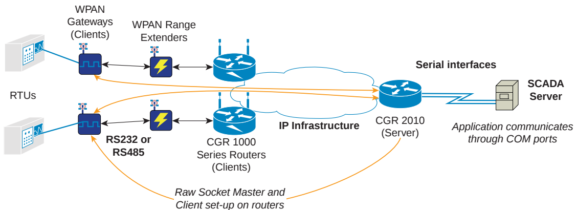
Figure 5-2 Raw Socket and Client/Server Setup on Routers
