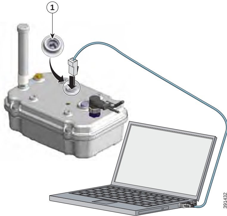
Figure 5-10 Connecting the Console Cable
