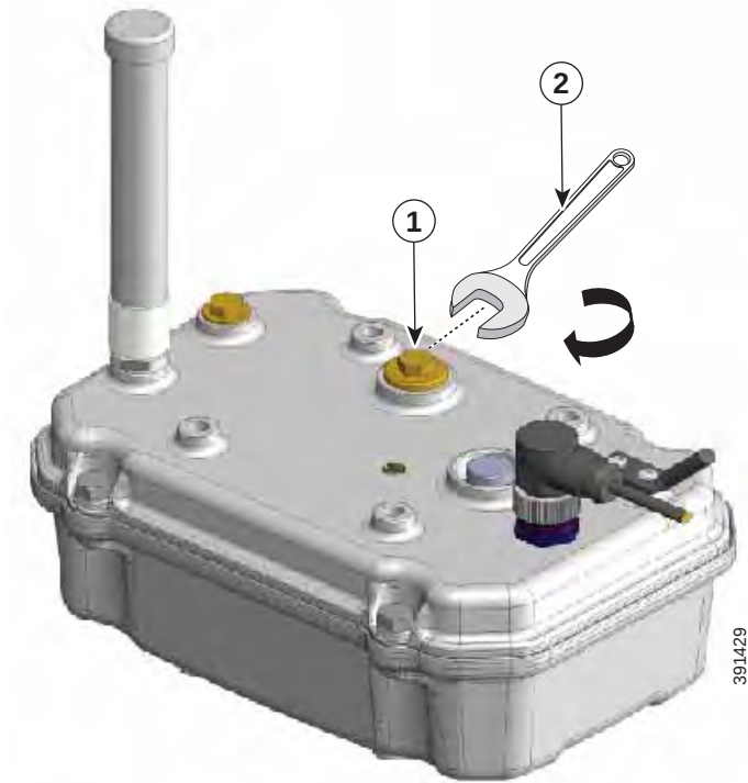
Figure 5-11 Covering the Console Port
