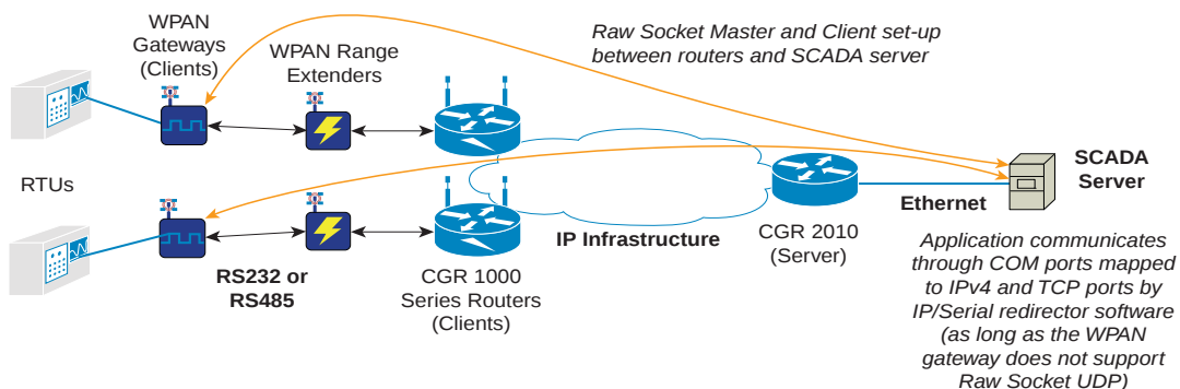
Figure 5-3 Raw Socket Client/Server Setup between Routers and SCADA Server with IP/Serial Redirector Software
