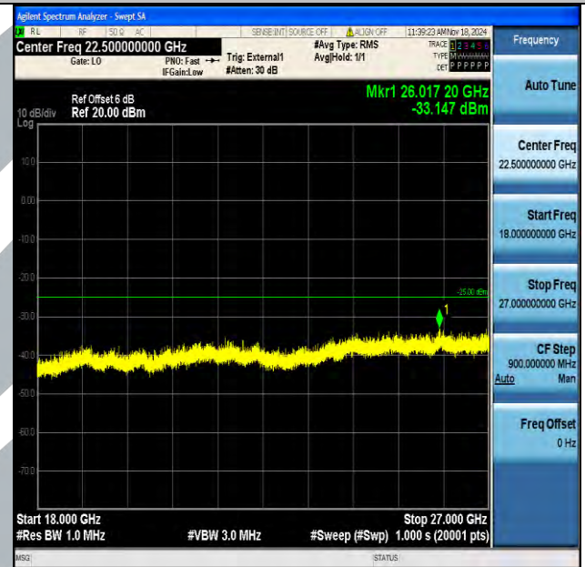
Band41_10MHz_16QAM_40590_1RB#0_18000~27000_18000~27000
