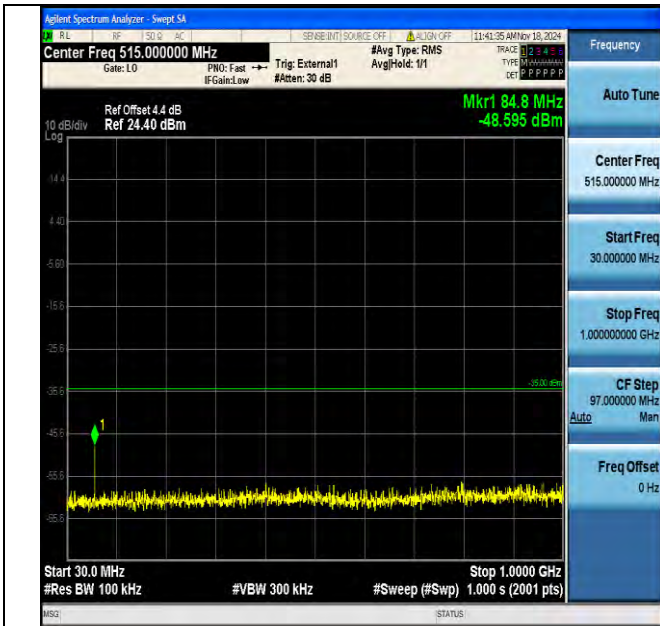
Band41_10MHz_16QAM_41190_1RB#0_30~1000_30~1000
