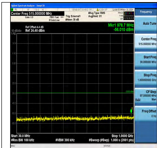
Band41 15MHz QPSK 40115 1RB#0 30~1000 30~1000
