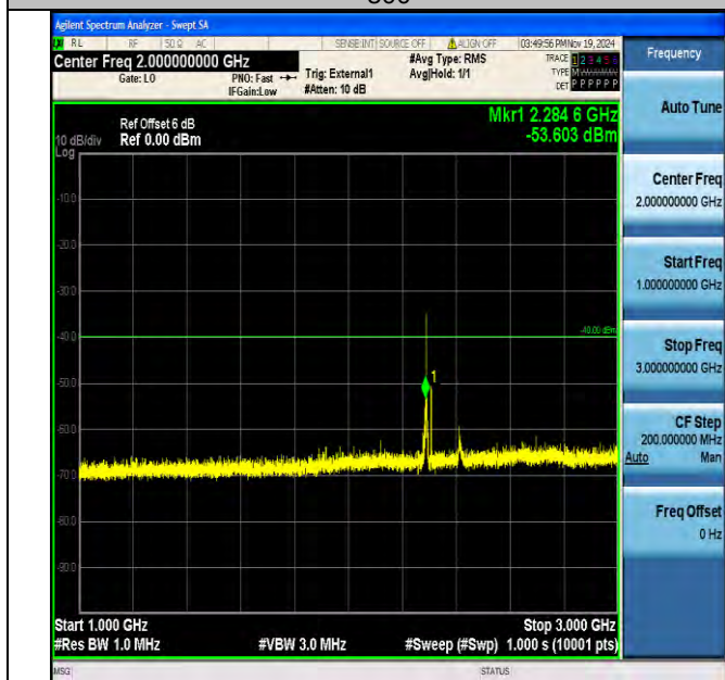
Band40_10MHz_16QAM_38750_1RB#0_1000~3000_1000~3000
