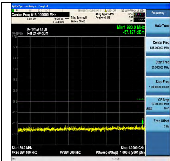
Band41_15MHz_16QAM_40590_1RB#0_30~1000_30~1000
