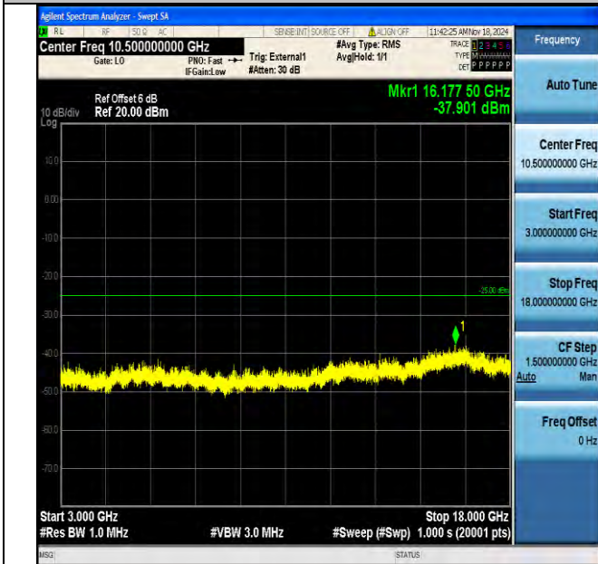
Band41_10MHz_16QAM_41190_1RB#0_3000~18000_3000~18000
