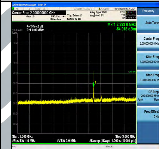
Band40_10MHz_QPSK_38750_1RB#0_1000~3000_1000~3000
