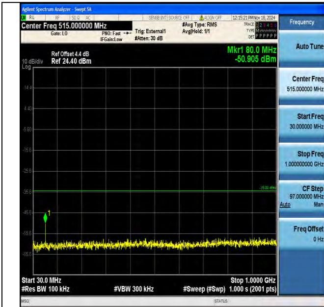
Band41_15MHz_16QAM_41165_1RB#0_30~1000_30~1000
