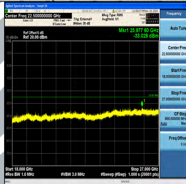
Band41_15MHz_QPSK_40115_1RB#0_18000~27000_18000~27000
