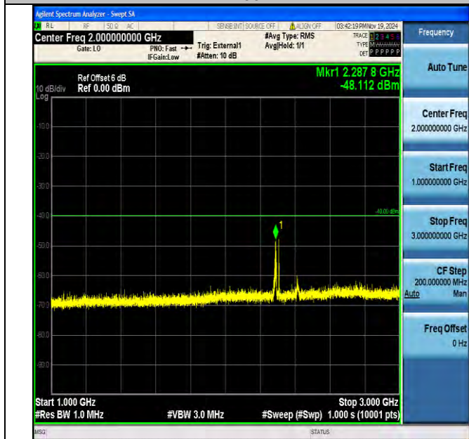
Band40_5MHz_16QAM_38725_1RB#0_1000~3000_1000~3000
