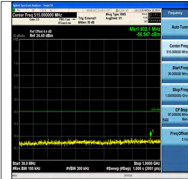
Band41 5MHz QPSK 40590 1RB#0 30~1000 30~1000
