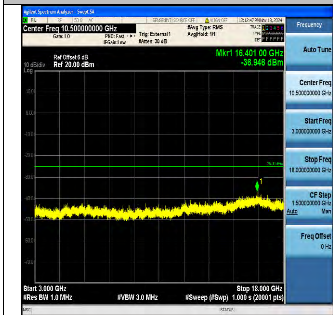
Band41_15MHz_16QAM_40590_1RB#0_3000~18000_3000~18000
