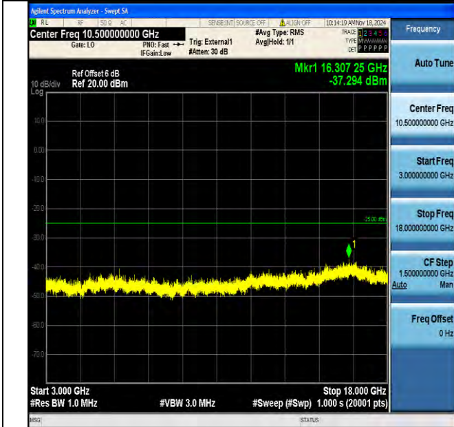
Band41_5MHz_QPSK_40590_1RB#0_3000~18000_3000~18000
