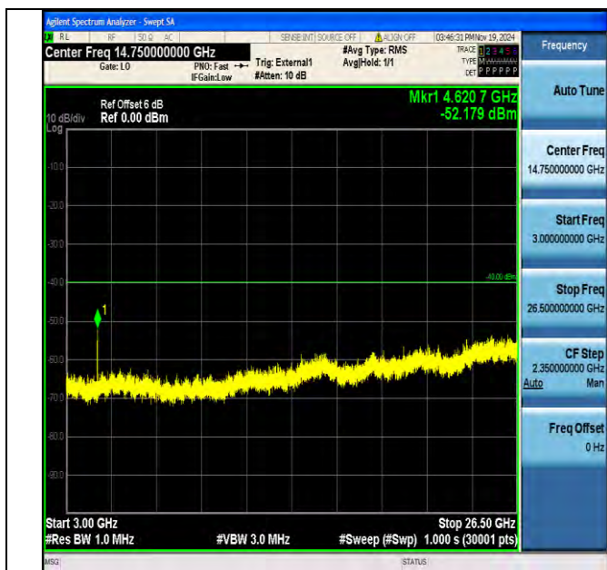
Band40_5MHz_QPSK_38775_1RB#0_3000~26500_3000~26500
