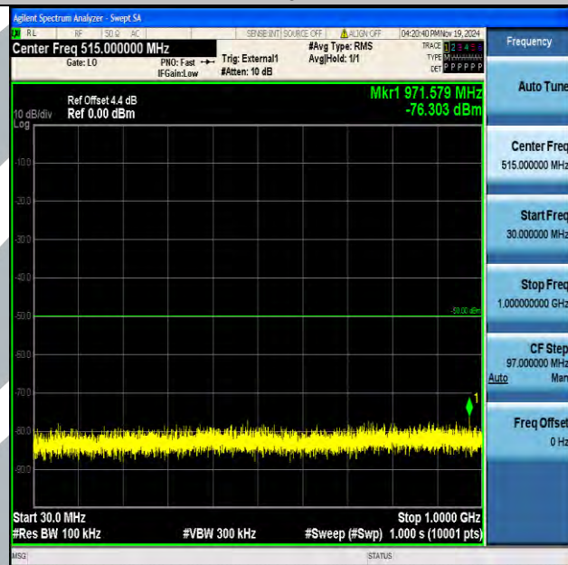
Band40_5MHz_16QAM_39225_1RB#0_30~1000_30~1000
