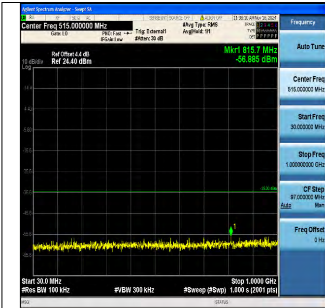
Band41_10MHz_16QAM_40590_1RB#0_30~1000_30~1000
