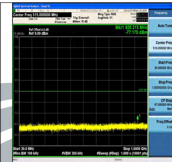
Band40_5MHz_16QAM_38725_1RB#0_30~1000_30~1000
