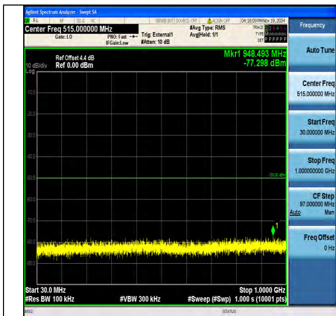
Band40_5MHz_16QAM_39200_1RB#0_30~1000_30~1000
