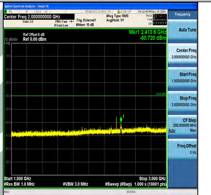
Band40_5MHz_QPSK_39225_1RB#0_1000~3000_1000~3000
