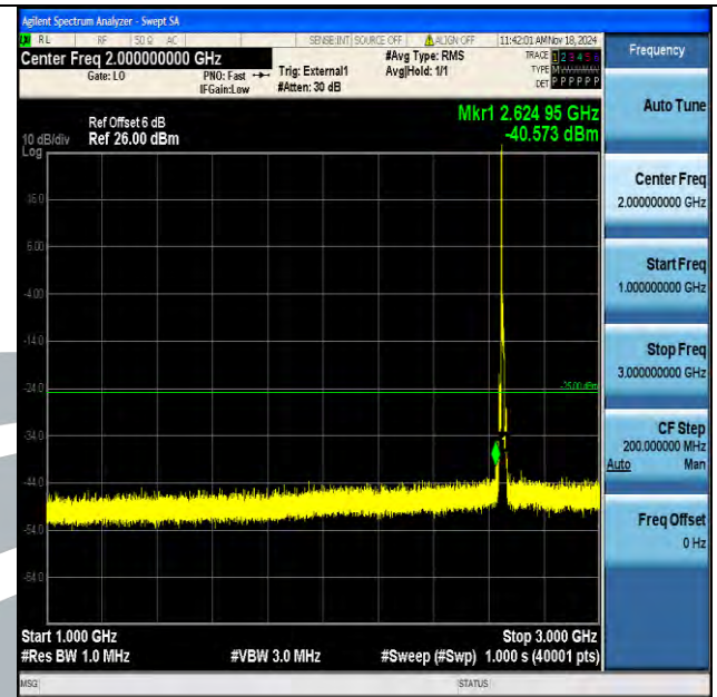
Band41_10MHz_16QAM_41190_1RB#0_1000~3000_1000~3000
