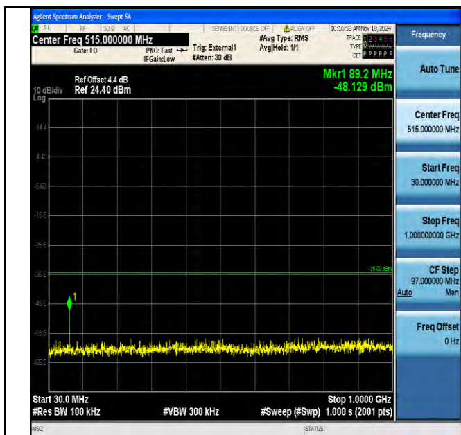
Band41 5MHz QPSK 41215 1RB#0 30~1000 30~1000
