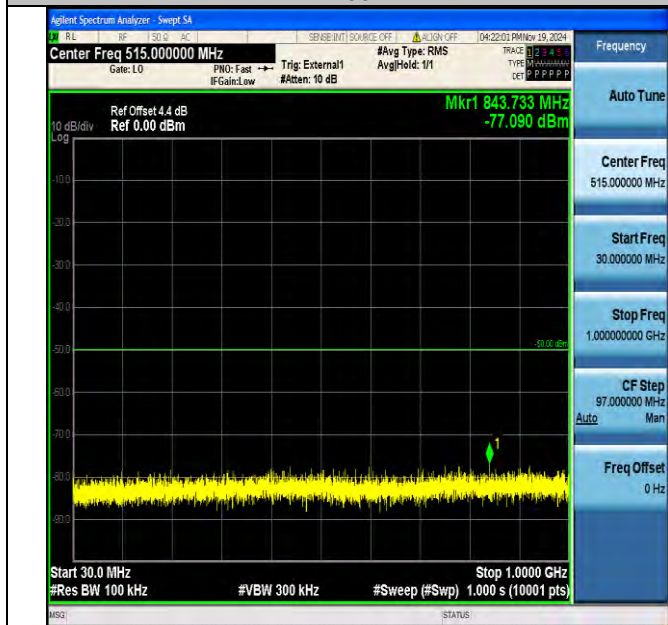
Band40_10MHz_QPSK_39200_1RB#0_30~1000_30~1000
