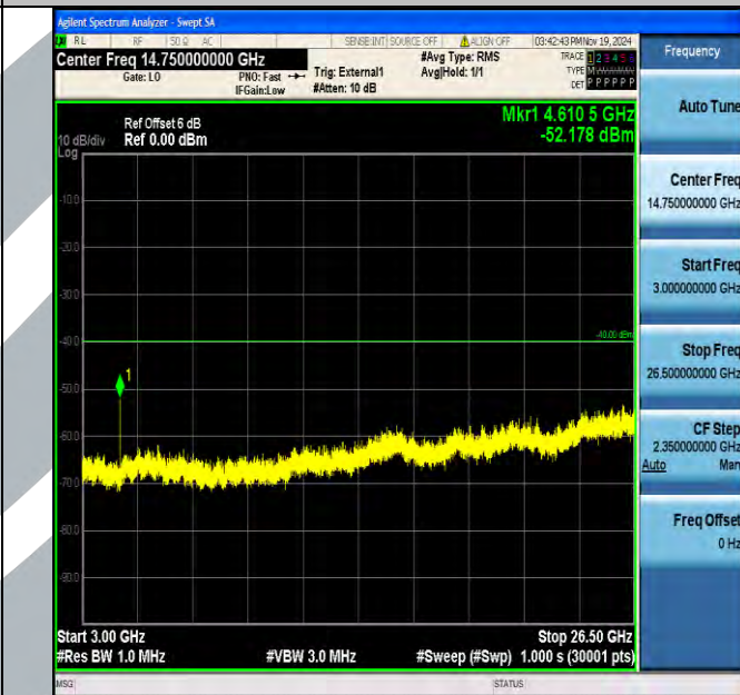
Band40_5MHz_16QAM_38725_1RB#0_3000~26500_3000~26500
