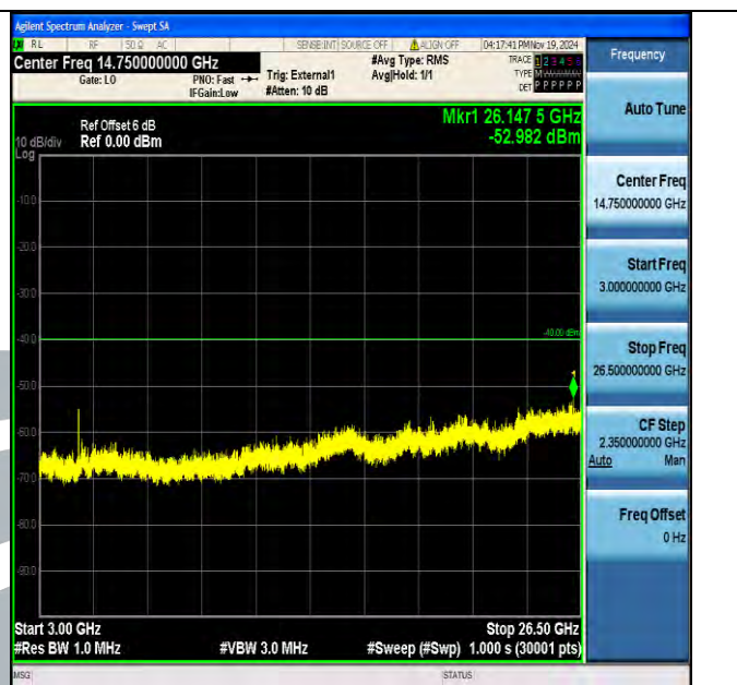
Band40_5MHz_QPSK_39200_1RB#0_3000~26500_3000~26500
