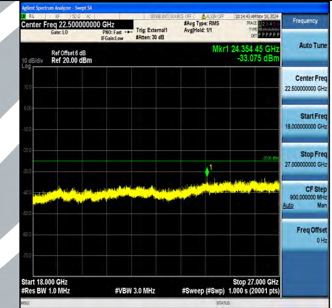
Band41_5MHz_QPSK_40590_1RB#0_18000~27000_18000~27000
