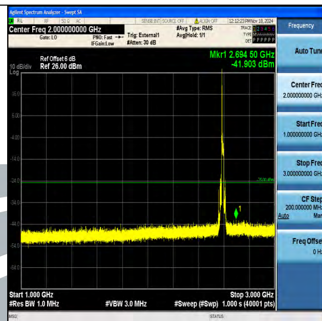
Band41_15MHz_16QAM_40590_1RB#0_1000~3000_1000~3000
