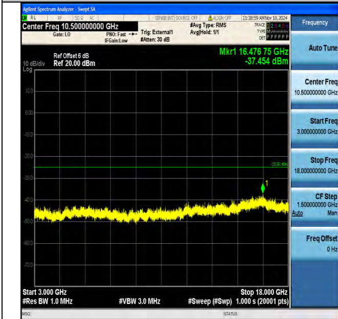
Band41_10MHz_16QAM_40590_1RB#0_3000~18000_3000~18000
