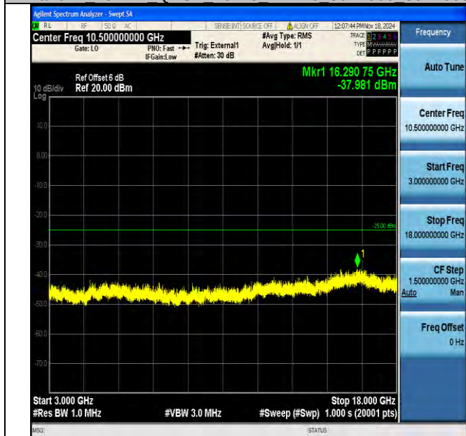
Band41_15MHz_QPSK_40115_1RB#0_3000~18000_3000~18000
