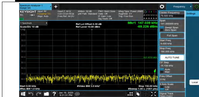
Band4-20MHz-QPSK-20300-1RB#0-0.009~0.15-PASS
