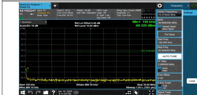
Band4-10MHz-QPSK-20350-50RB#0-0.15~30-PASS
