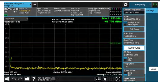
Band4-15MHz-QPSK-20025-75RB#0-0.15~30-PASS
