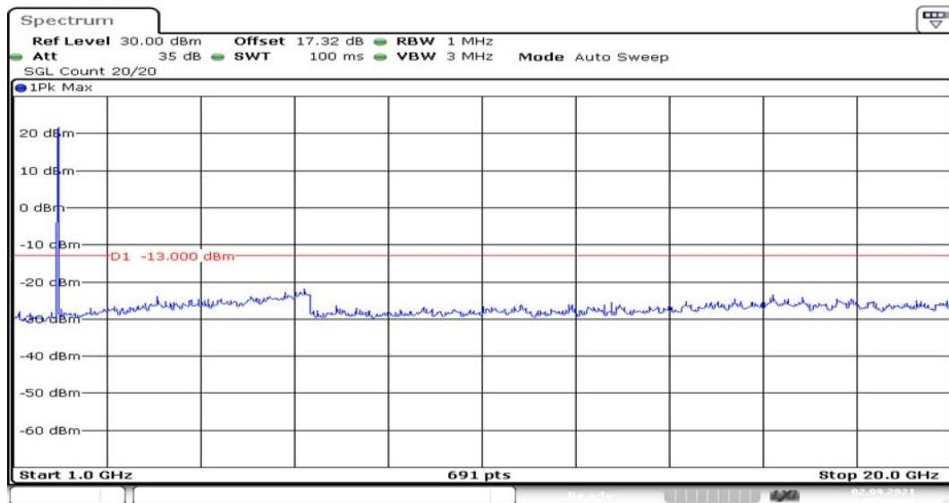
Channel 9400 1GHz~20GHz(dBm)
