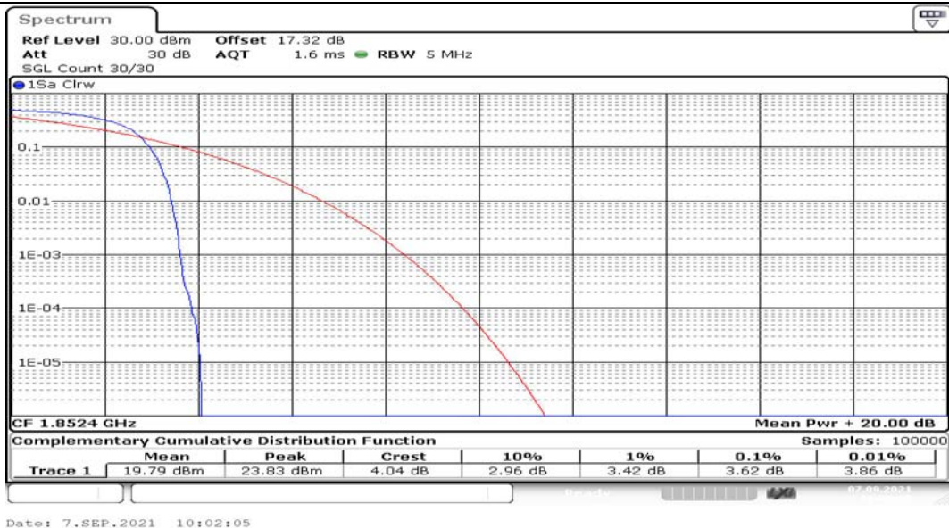
Channel 9262
