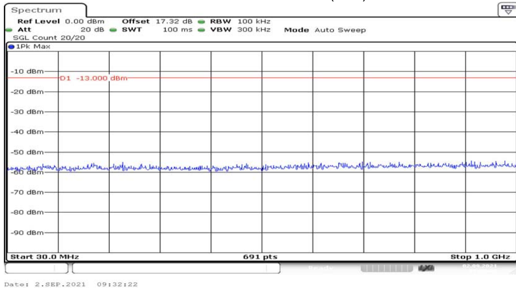
Channel 9400 30MHz~1GHz(dBm)
