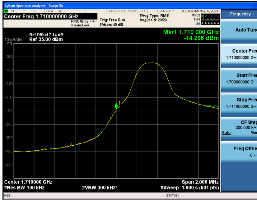
Band4-5MHz-QPSK-19975-1RB#24
