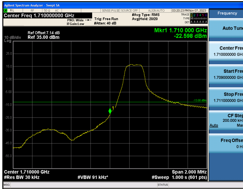
Band4-1.4MHz-QPSK-19957-1RB#5
