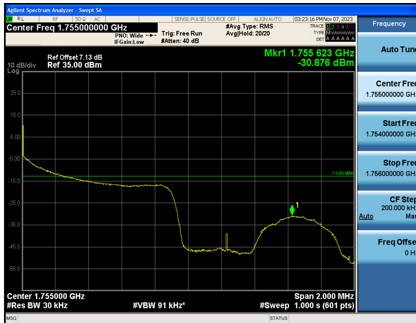
Band4-1.4MHz-QPSK-20393-1RB#5
