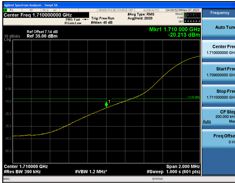
Band4-20MHz-16QAM-20050-1RB#99
