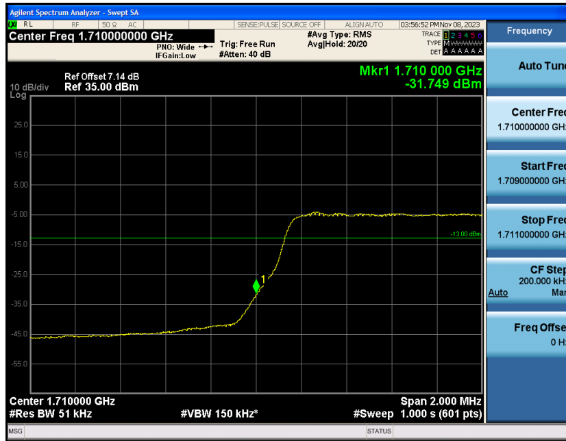
Band4-3MHz-QPSK-20385-1RB#0
