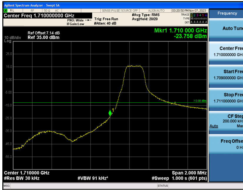
Band4-1.4MHz-16QAM-19957-1RB#5
