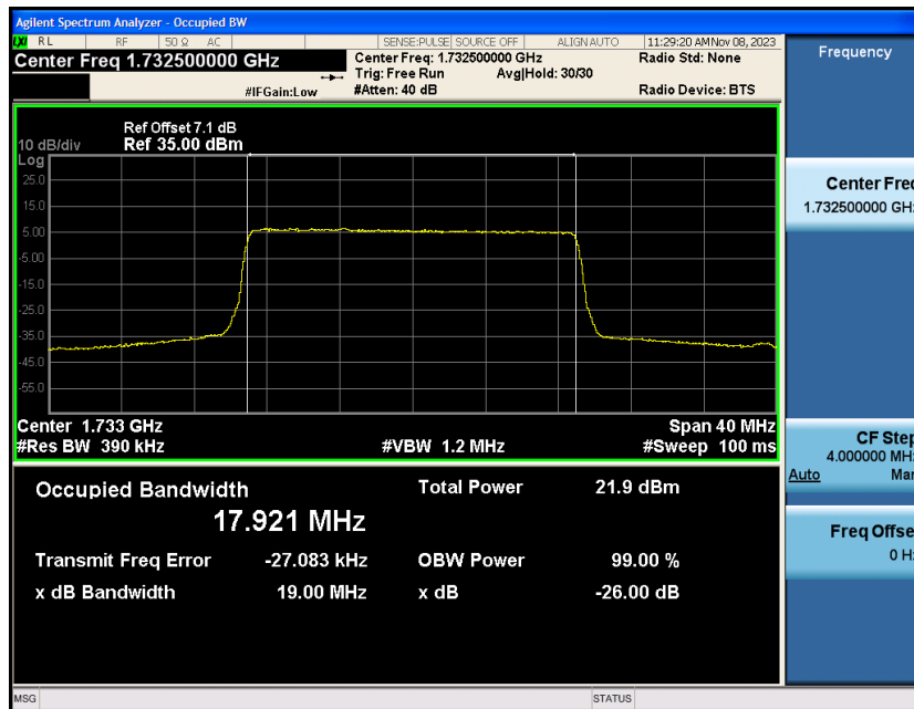
Band4-20MHz-QPSK-20300-100RB#0
