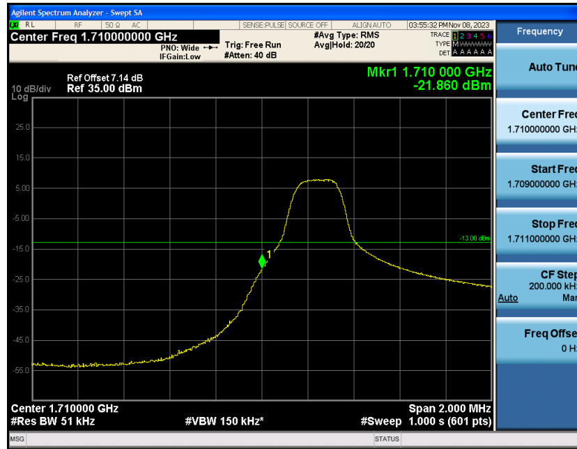
Band4-3MHz-16QAM-19965-1RB#14
