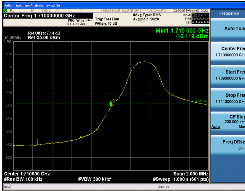
Band4-5MHz-16QAM-19975-1RB#24
