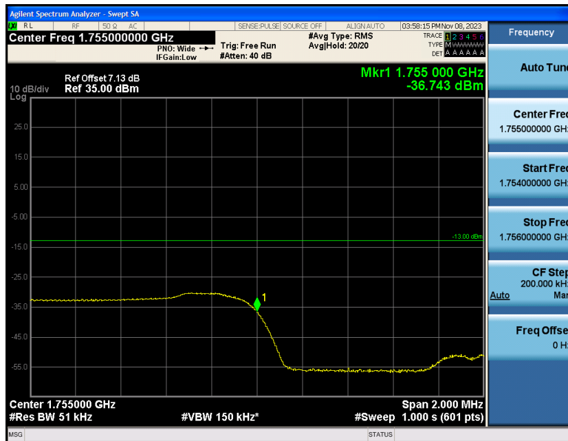
Band4-3MHz-16QAM-20385-1RB#14
