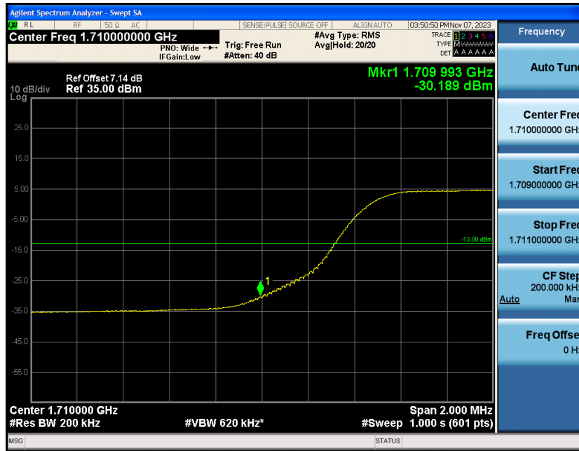
Band4-10MHz-QPSK-20000-1RB#49
