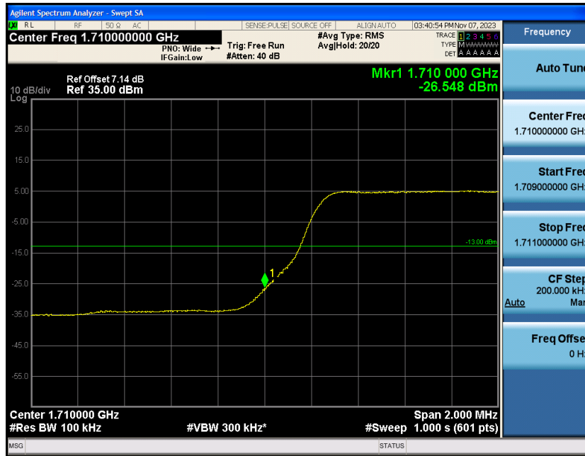
Band4-5MHz-16QAM-20375-1RB#0
