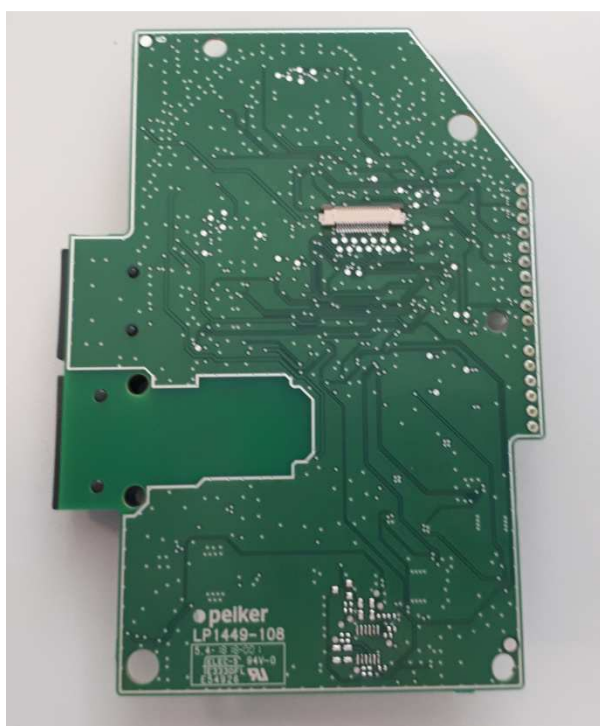
main-board, bottom view
