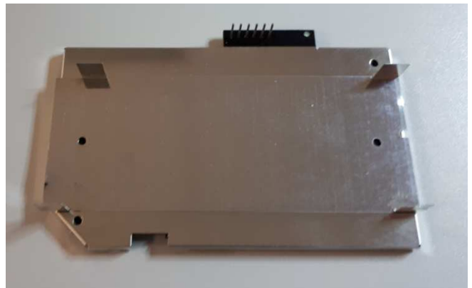
Charging coil element with connector, ferrite plate and metal shield, view from top and bottom side.
