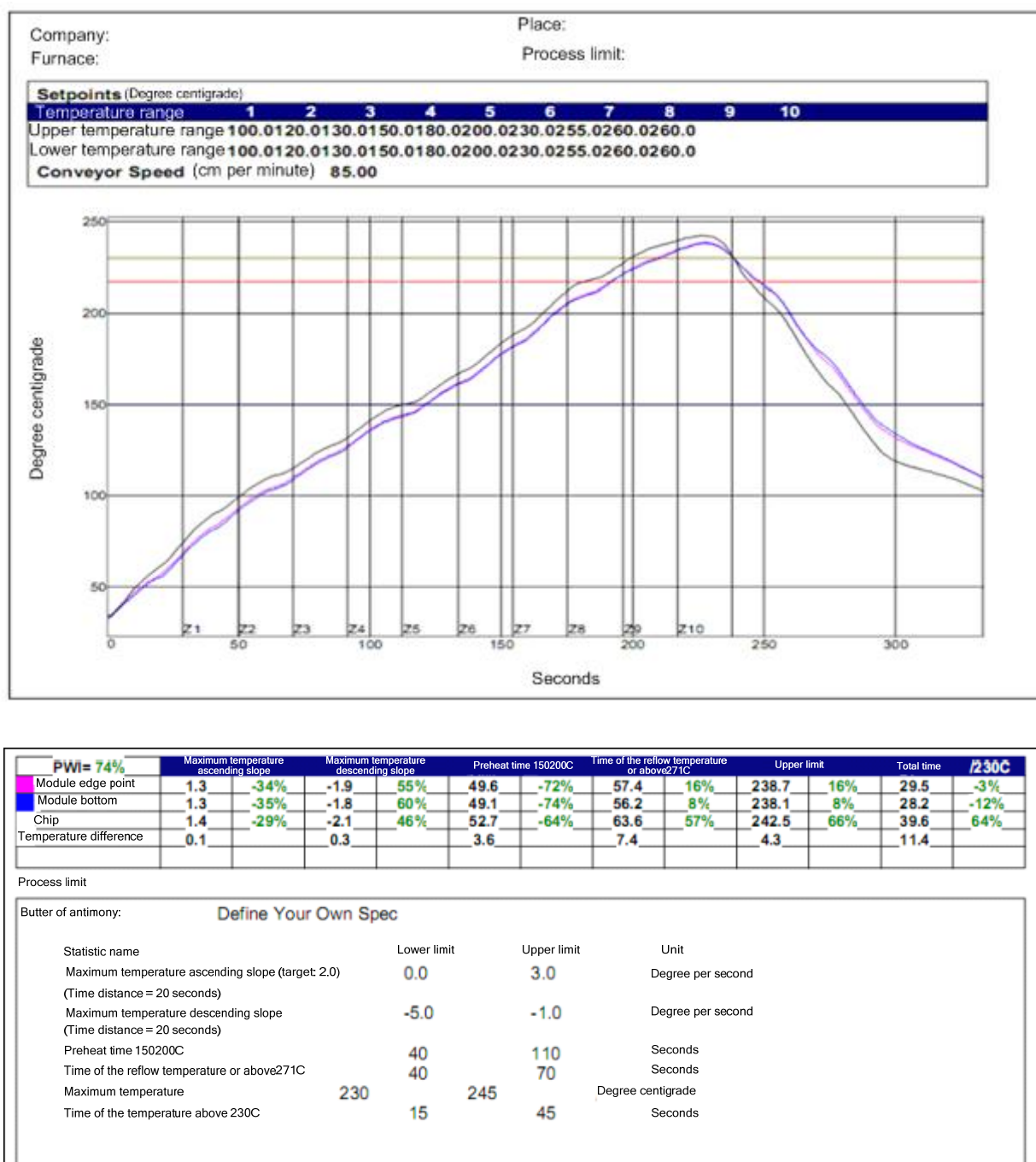
Figure 6-2 The reference temperature curve
