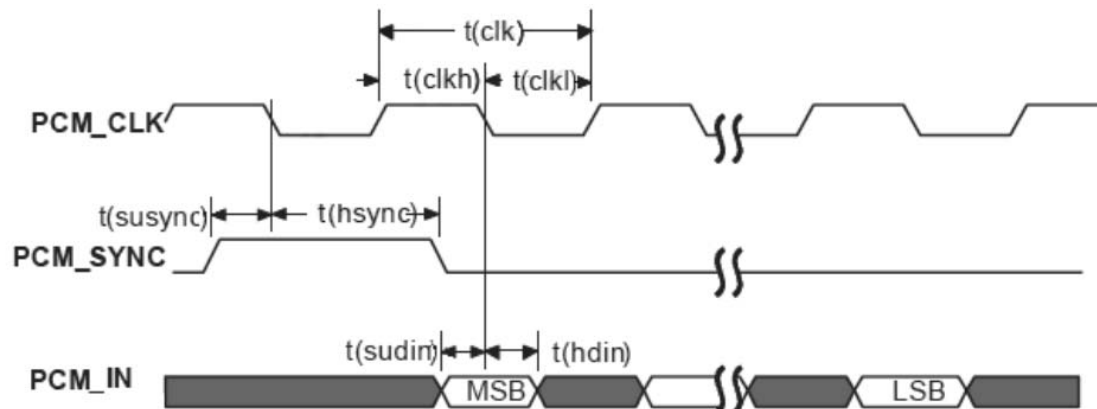
Figure 3-8 Codec to L600 module timing
