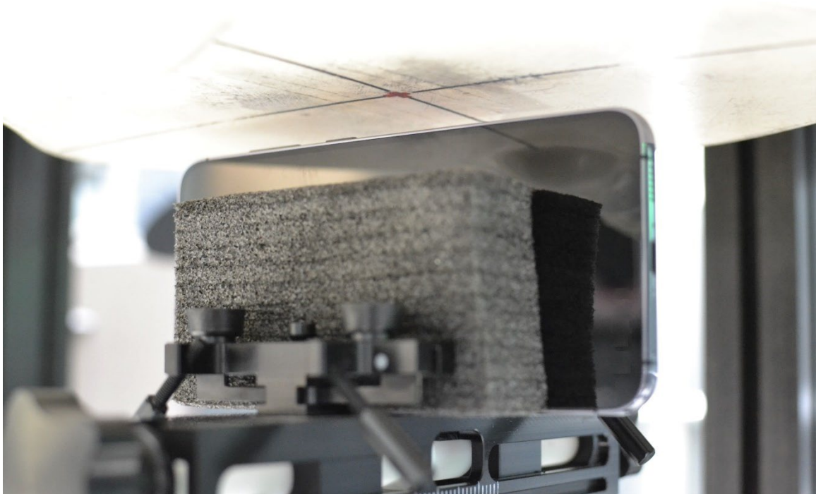
SAR Test Setup Photo 17 – Hotspot, Right Edge at 10mm
