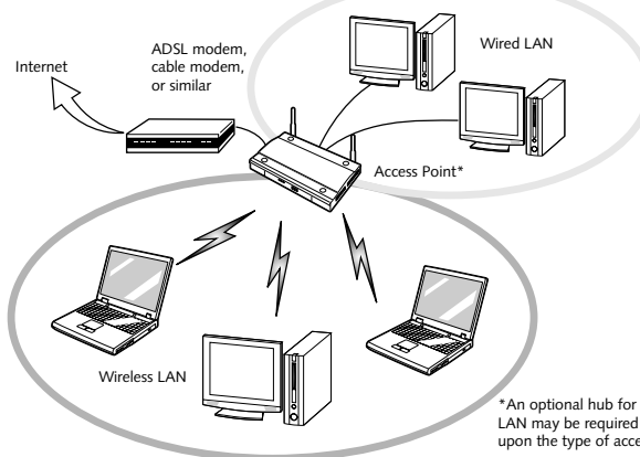
Figure A-2. Access Point (Infrastructure) Mode Network
