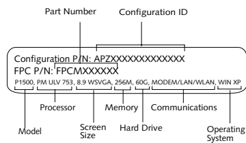
Figure 7-1. Configuration Label
