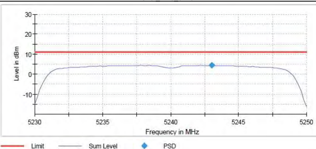
11AC20 Ant6 5240
