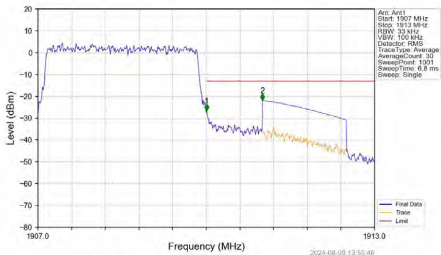
Band2_3MHz_16QAM_HCH_1908.5MHz_RB_15_0_NTNV
