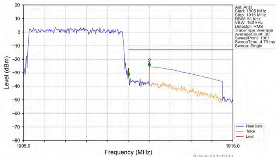
Band2_5MHz_16QAM_HCH_1907.5MHz_RB_25_0_NTNV
