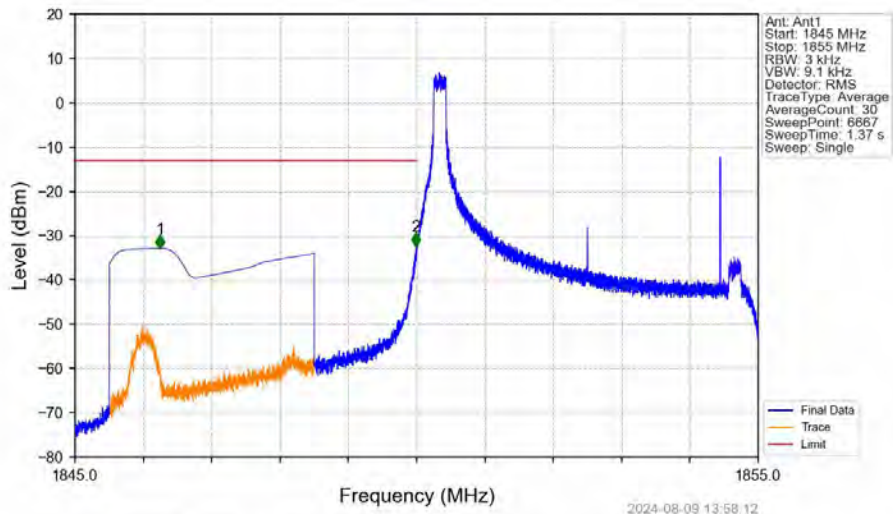
Band2_5MHz_16QAM_LCH_1852.5MHz_RB_1_0_NTNV
