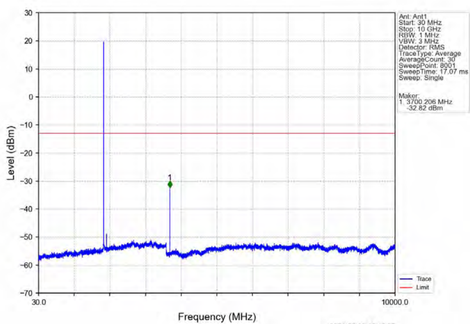
Band2_1.4MHz_16QAM_LCH_1850.7MHz_RB_1_0_NTNV
