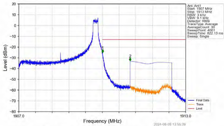
Band2_3MHz_16QAM_HCH_1908.5MHz_RB_1_14_NTNV
