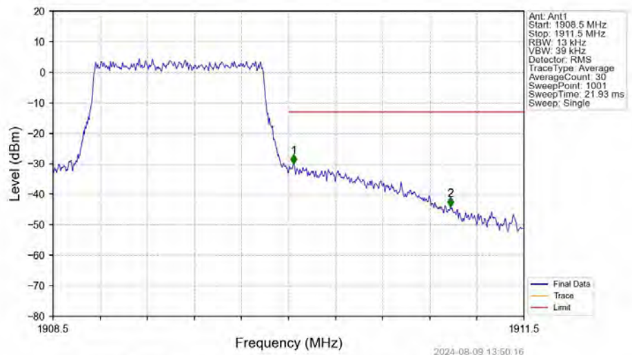
Band2_1.4MHz_QPSK_HCH_1909.3MHz_RB_6_0_NTNV
