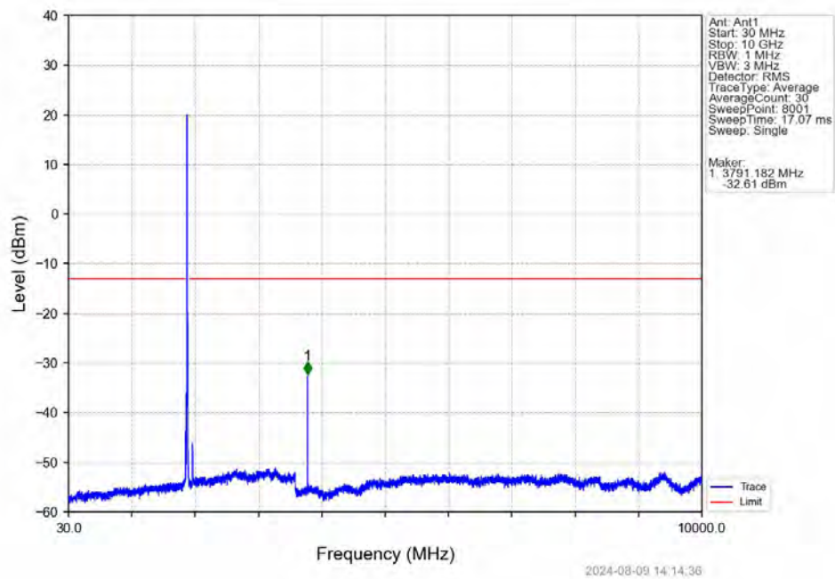
Band2_15MHz_16QAM_HCH_1902.5MHz_RB_1_0_NTNV
