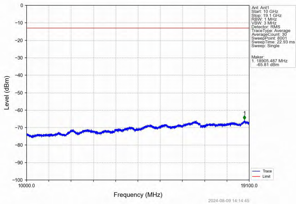
Band2_15MHz_16QAM_HCH_1902.5MHz_RB_1_0_NTNV
