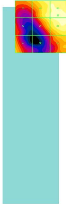
Figure 11-1 Sample E-field Scan Overlay (T-Coil Centered Scan pictured. See Test Setup Photographs for Acoustic Scan Overlay and actual WD overlay.)
