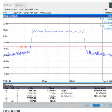
1-N66-PC3-15-10-L-7-CP-16QAM-Outer_Full-52@0-Ant1-9.278-9.980-≤10-PASS
