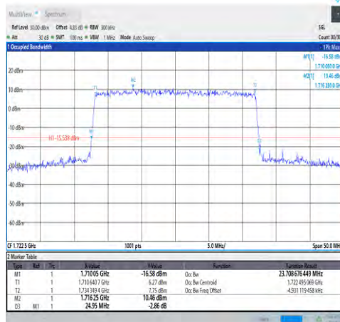
1-N66-PC3-15-25-L-7-CP-16QAM-Outer_Full-133@0-Ant1-23.709-24.950-≤25-PASS
