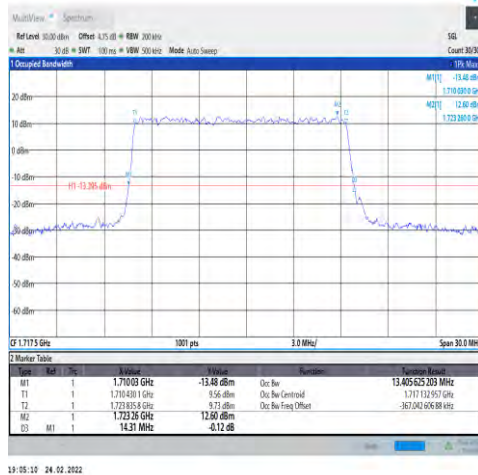
1-N66-PC3-15-15-L-1-DFT-QPSK-Outer_Full -75@0-Ant1-13.406-14.310-≤15-PASS
