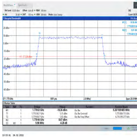
1-N66-PC3-15-10-H-8-CP-64QAM-Outer_Full I-52@0-Ant1-9.288-9.980-≤10-PASS
