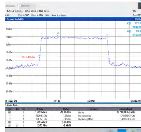
1-N66-PC3-15-25-L-8-CP-64QAM-Outer_Full-133@0-Ant1-23.733-25.150-≤25-PASS
