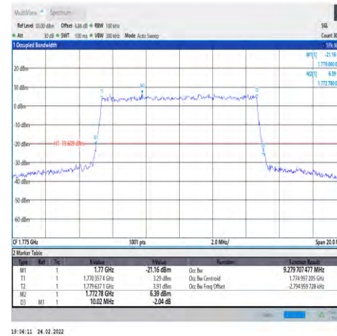
1-N66-PC3-15-10-H-9-CP-256QAM-Outer_Full ull-52@0-Ant1-9.28-10.020-≤10-PASS
