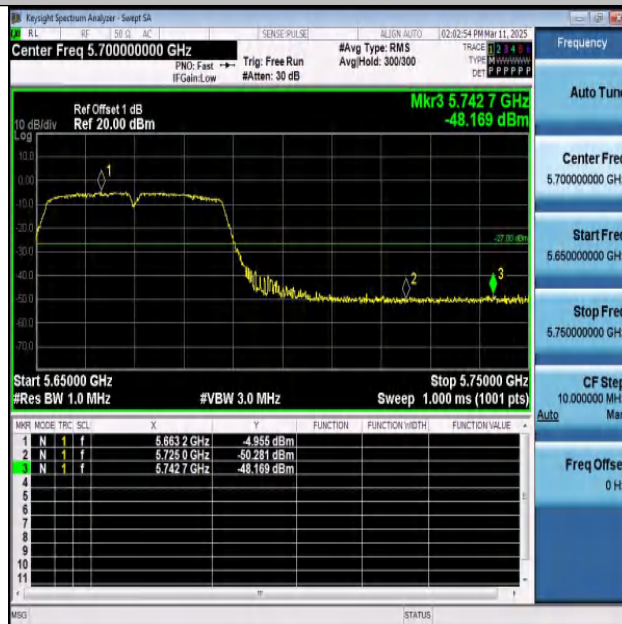
11N40SISO-Ant1-5670-PASS
