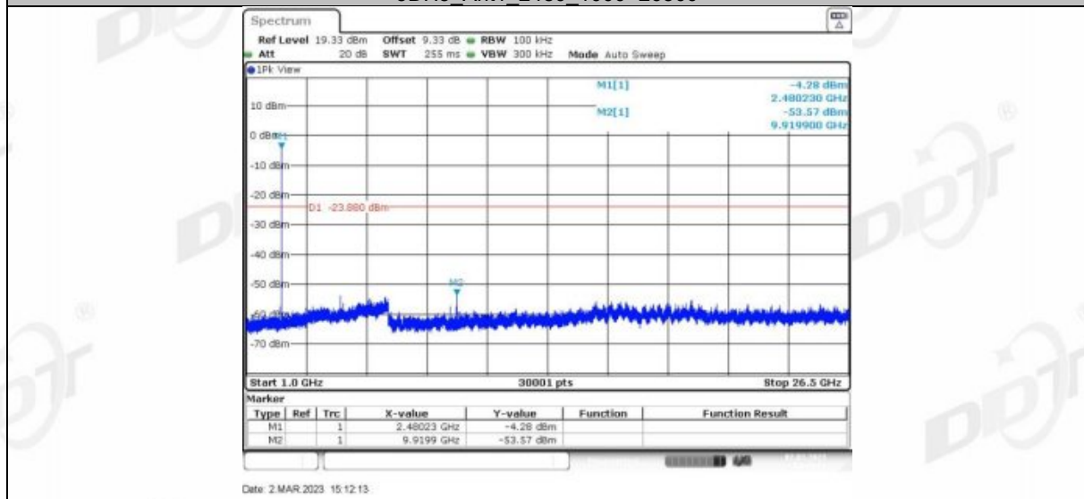
3DH5_Ant1_2480_1000~26500
