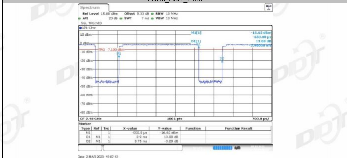
3DH5_Ant1_2402
