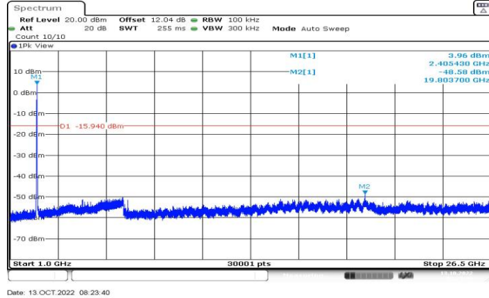
11G_Ant1_2412_1000-26500
