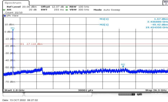
11N20SISO_Ant1_2437_1000~26500
