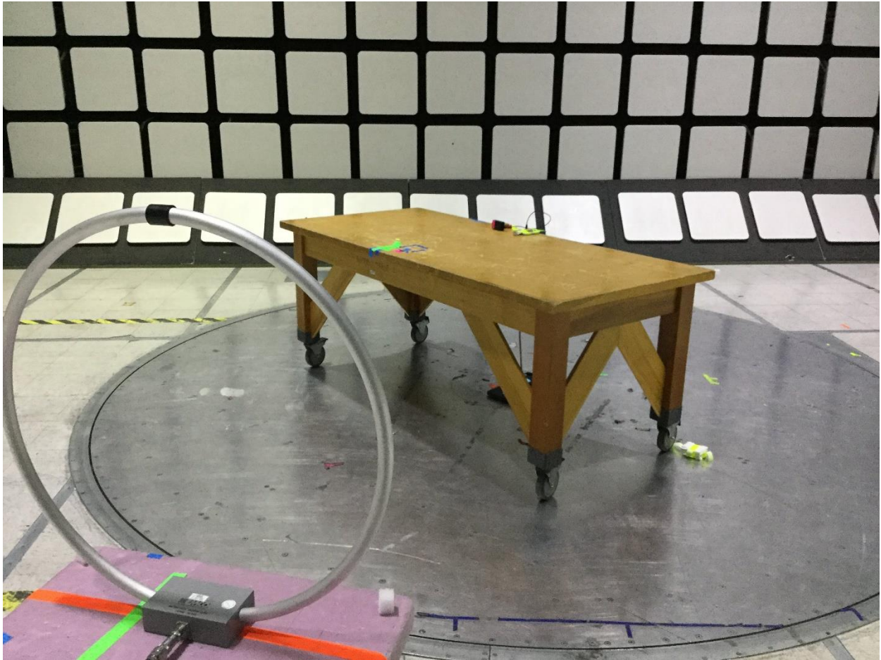
13 – 30 MHz test setup
