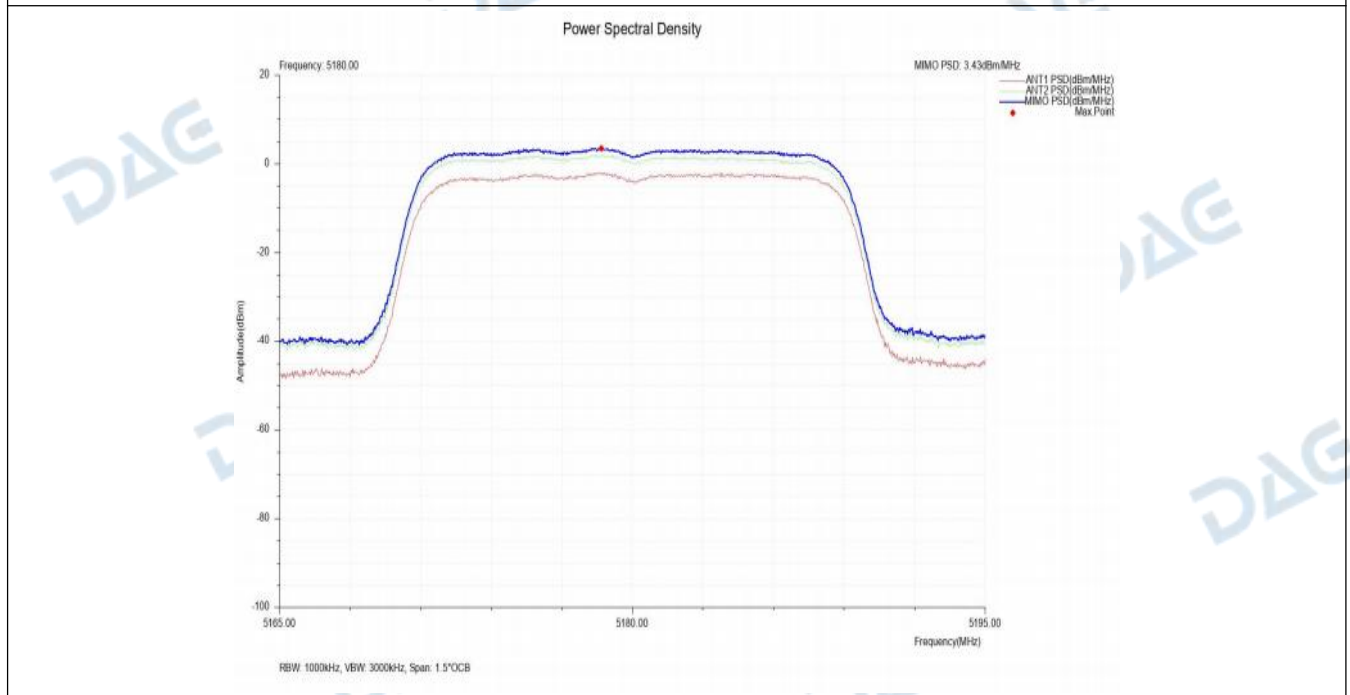
NVNT_MIMO_TX_802_11n(HT20)_Power_Spectral_Density_5180
