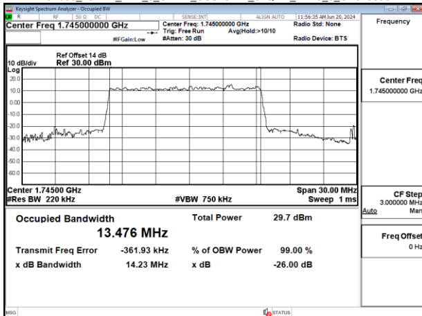
Band66_15MHz_DFT_s_OFDM_SCS15kHz_64QAM_RB75_0_CH349000
