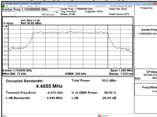
Band66_5MHz_DFT_s_OFDM_SCS15kHz_QPSK_RB25_0_CH349000
