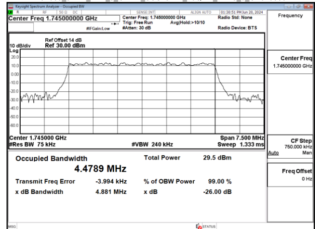
Band66_5MHz_DFT_s_OFDM_SCS15kHz_16QAM_RB25_0_CH349000
