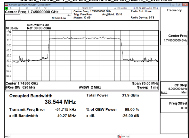
Band66_40MHz_DFT_s_OFDM_SCS15kHz_BPSK_RB216_0_CH349000
