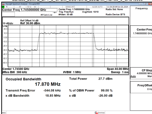
Band66_20MHz_DFT_s_OFDM_SCS15kHz_256QAM_RB100_0_CH349000
