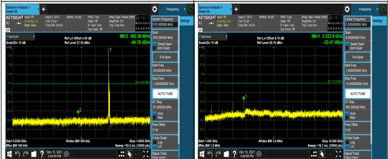
Band12-10MHz-16QAM-23130-1RB#0-Range1:30~1000MHz
