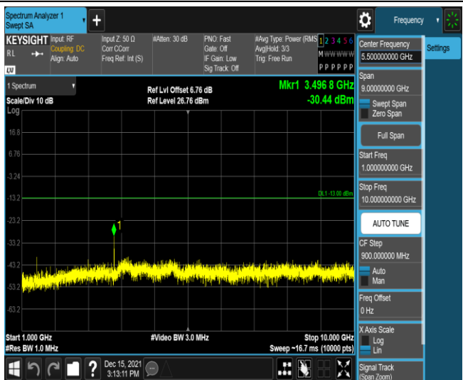
Band12-1.4MHz-16QAM-23095-1RB#0-Range2:100 0~10000MHz
