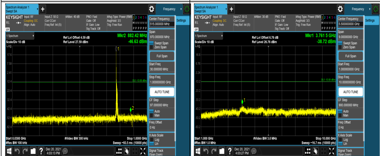
Band13-10MHz-QPSK-23230-1RB#0-Range1:30~10000MHz
