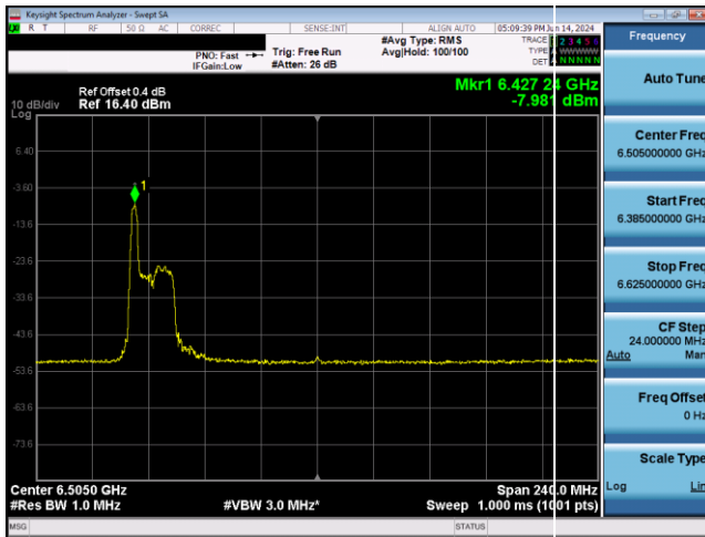
Plot 7-819. LPI Power Spectral Density Plot SDM Antenna 5T (160MHz 802.11ax RU26 (UNII Band 6) – Ch. 111)
