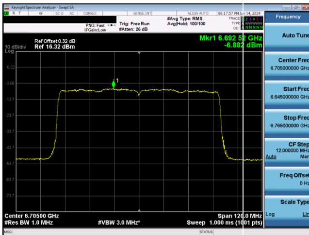
Plot 7-849. LPI Power Spectral Density Plot SDM Antenna 5T (80MHz 802.11ax RU996 (UNII Band 7) – Ch. 151)
