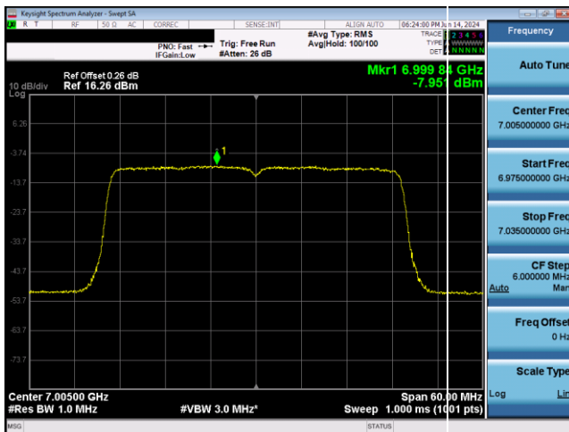
Plot 7-873. LPI Power Spectral Density Plot SDM Antenna 5T (40MHz 802.11ax RU484 (UNII Band 8) – Ch. 211)
