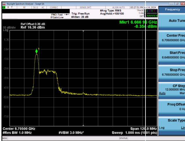
Plot 7-843. LPI Power Spectral Density Plot SDM Antenna 5T (80MHz 802.11ax RU26 (UNII Band 7) – Ch. 151)
