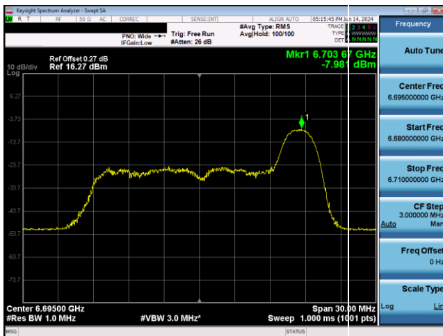
Plot 7-831. LPI Power Spectral Density Plot SDM Antenna 5T (20MHz 802.11ax RU26 (UNII Band 7) – Ch. 149)
