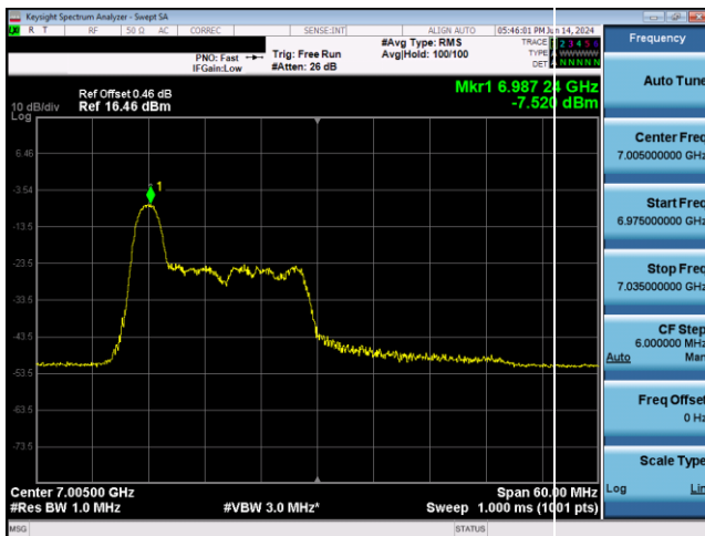
Plot 7-867. LPI Power Spectral Density Plot SDM Antenna 5T (40MHz 802.11ax RU26 (UNII Band 8) – Ch. 211)
