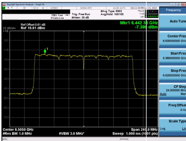
Plot 7-825. LPI Power Spectral Density Plot SDM Antenna 5T (160MHz 802.11ax RU996x2 (UNII Band 6) – Ch. 111)
