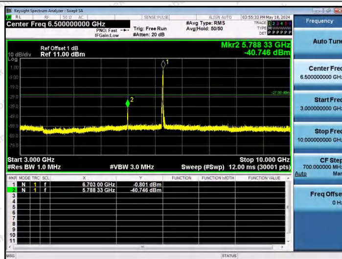
11AX40SISO-Ant1-6685-52Tone-RU44-3000~10000-PASS
