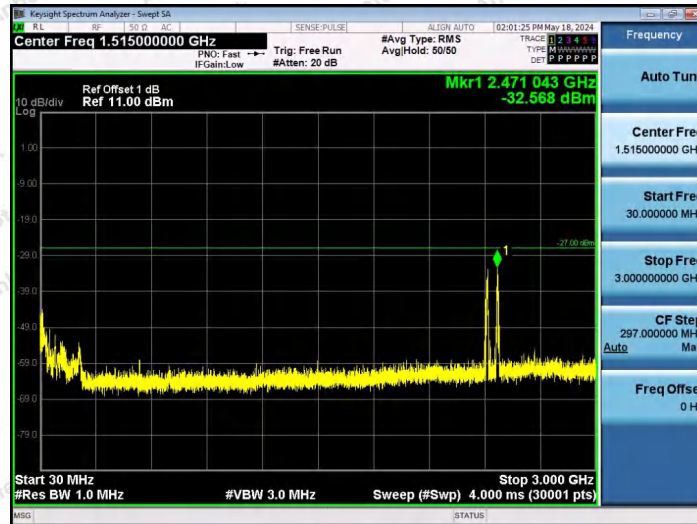
11AX40SISO-Ant1-6445-26Tone-RU0-30~3000-PASS
