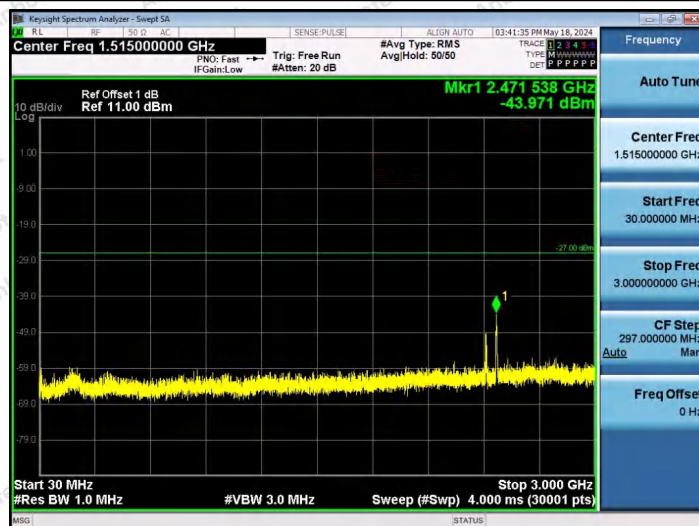
11AX40SISO-Ant1-6565-242Tone-RU61-30~3000-PASS
