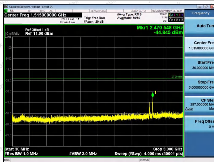
11AX40SISO-Ant1-6565-106Tone-RU56-30~3000-PASS
