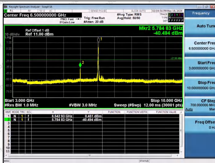
11AX40SISO-Ant1-6525-52Tone-RU44-3000~10000-PASS
