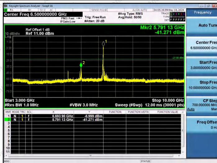
11AX40SISO-Ant1-6685-242Tone-RU62-3000~10000-PASS
