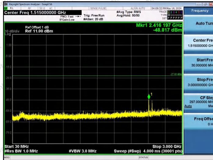
11AX40SISO-Ant1-6845-26Tone-RU0-30~3000-PASS
