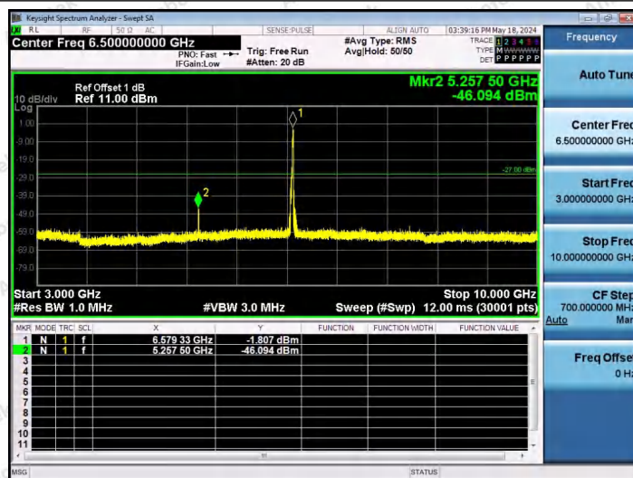
11AX40SISO-Ant1-6565-106Tone-RU56-3000~10000-PASS
