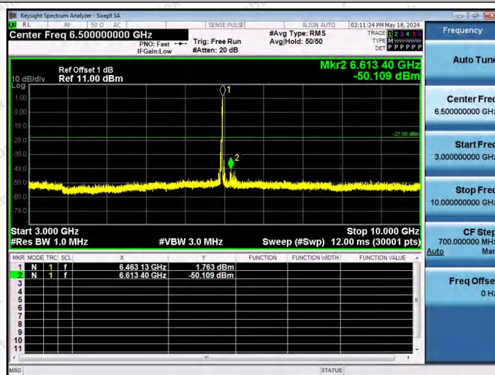
11AX40SISO-Ant1-6445-52Tone-RU44-3000~10000-PASS
