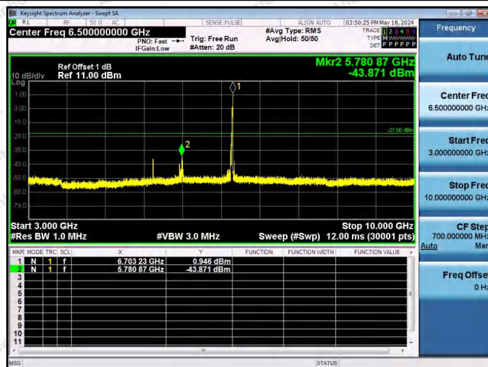
11AX40SISO-Ant1-6685-26Tone-RU17-3000~10000-PASS
