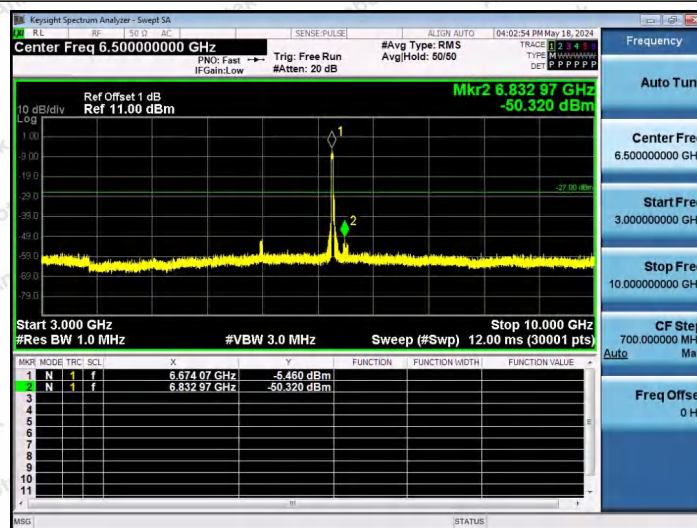
11AX40SISO-Ant1-6685-242Tone-RU61-3000~10000-PASS
