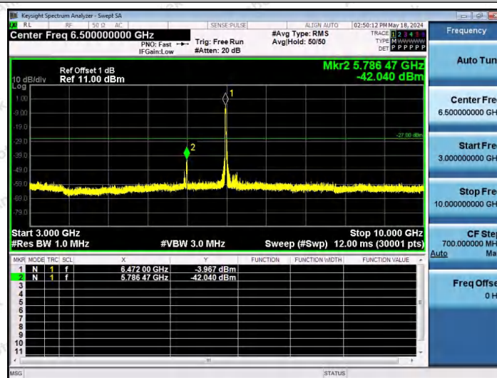
11AX40SISO-Ant1-6485-242Tone-RU61-3000~10000-PASS
