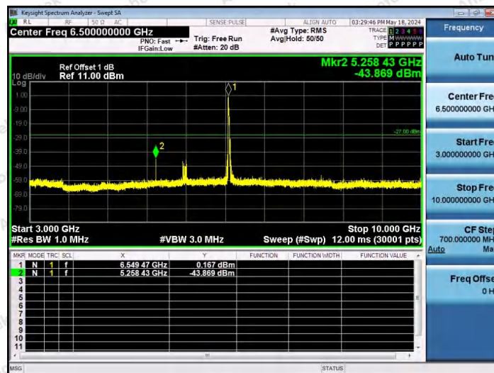
11AX40SISO-Ant1-6565-52Tone-RU37-3000~10000-PASS
