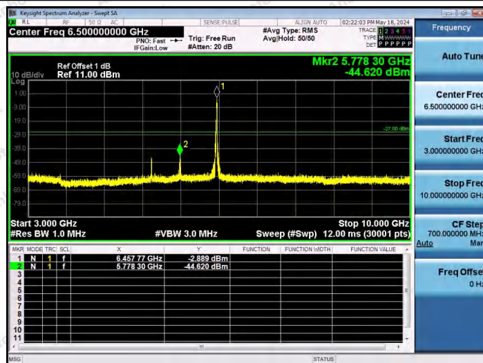
11AX40SISO-Ant1-6445-242Tone-RU62-3000~10000-PASS
