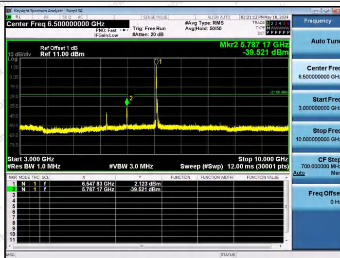
11AX40SISO-Ant1-6565-26Tone-RU0-3000~10000-PASS
