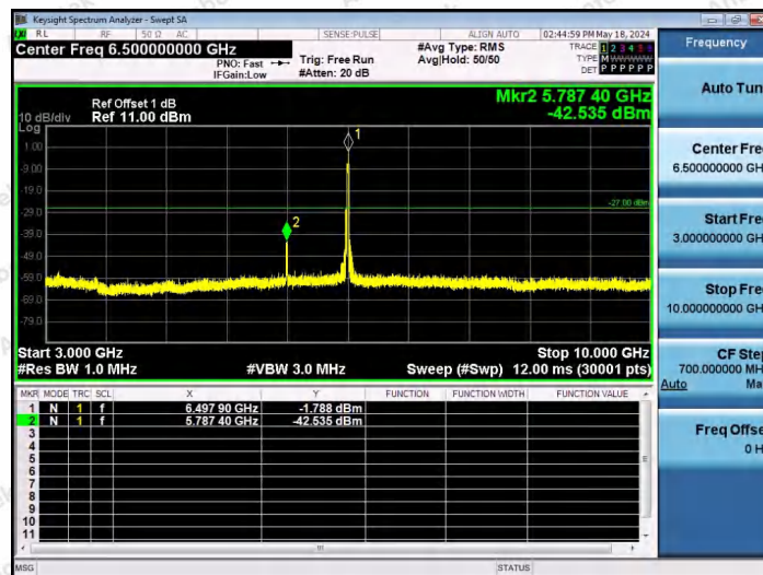
11AX40SISO-Ant1-6485-106Tone-RU56-3000~10000-PASS
