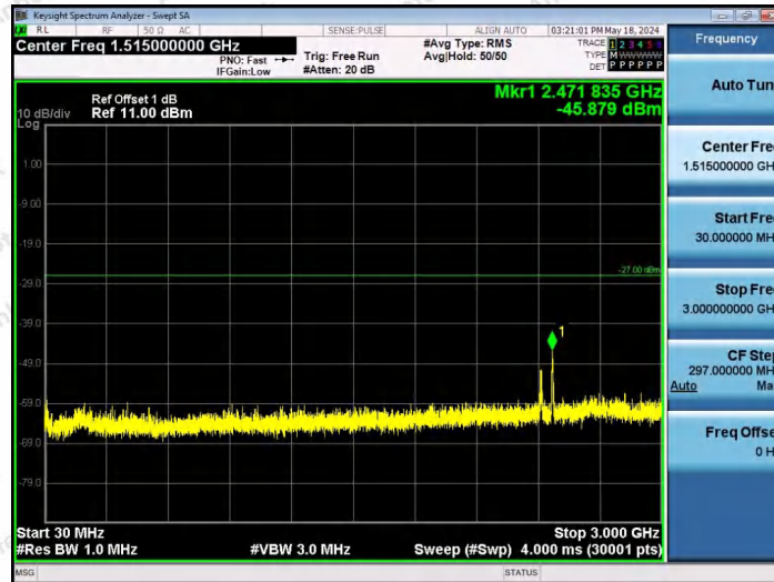
11AX40SISO-Ant1-6565-26Tone-RU0-30~3000-PASS
