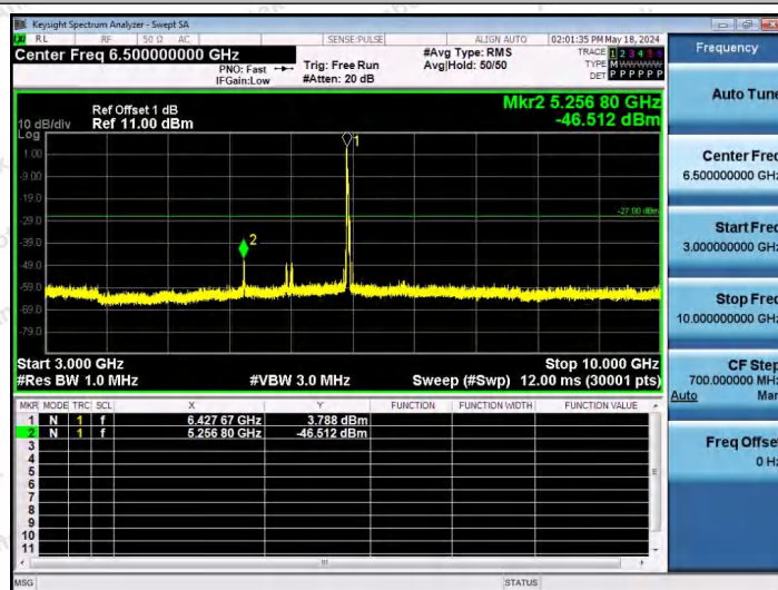
11AX40SISO-Ant1-6445-26Tone-RU0-3000~10000-PASS
