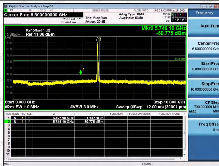
11AX40SISO-Ant1-6445-52Tone-RU37-3000~10000-PASS
