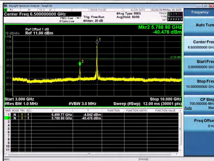
11AX40SISO-Ant1-6485-242Tone-RU62-3000~10000-PASS
