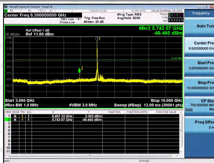
11AX40SISO-Ant1-6485-26Tone-RU0-3000~10000-PASS
