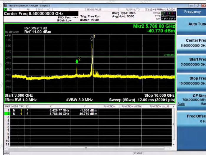
11AX40SISO-Ant1-6445-106Tone-RU53-3000~10000-PASS
