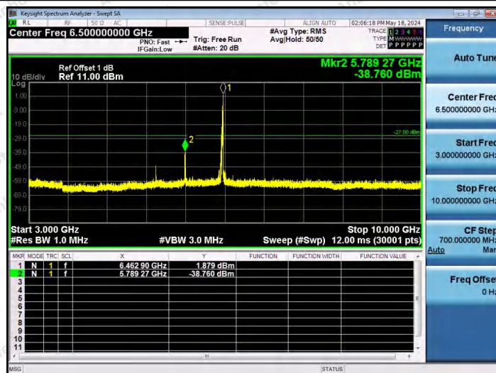
11AX40SISO-Ant1-6445-26Tone-RU17-3000~10000-PASS
