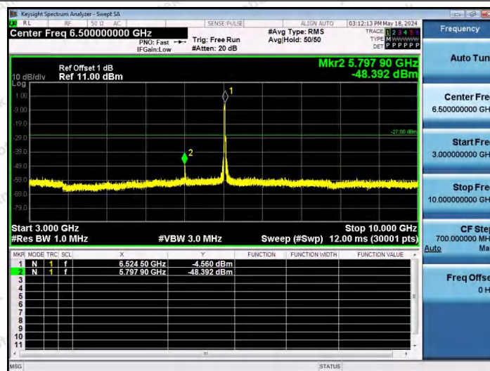
11AX40SISO-Ant1-6525-242Tone-RU61-3000~10000-PASS
