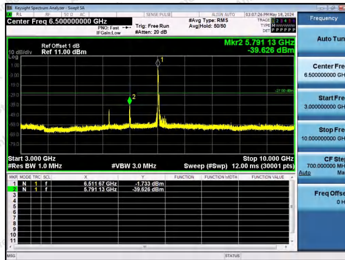
11AX40SISO-Ant1-6525-106Tone-RU53-3000~10000-PASS
