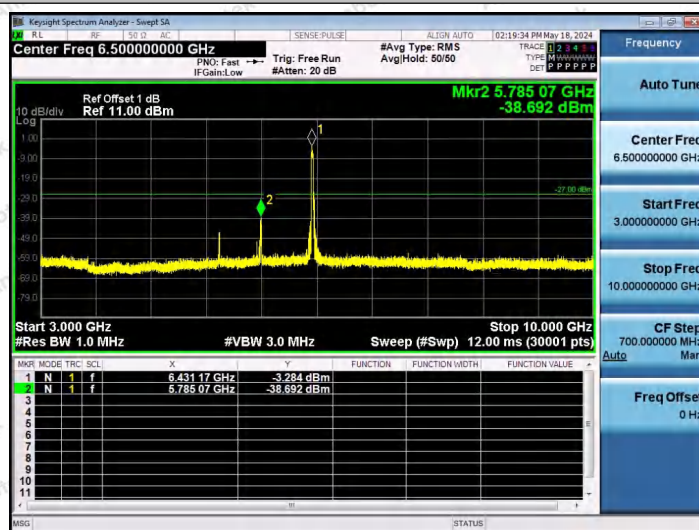
11AX40SISO-Ant1-6445-242Tone-RU61-3000~10000-PASS
