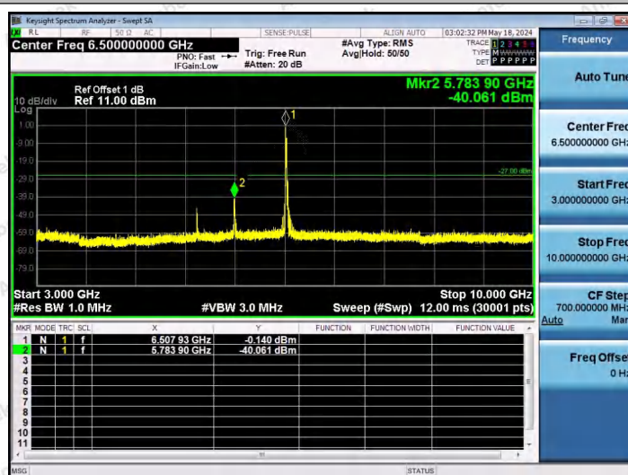
11AX40SISO-Ant1-6525-52Tone-RU37-3000~10000-PASS
