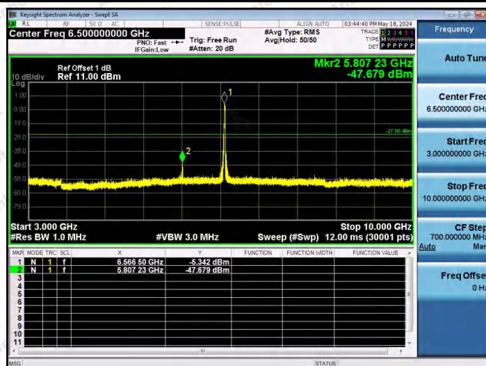
11AX40SISO-Ant1-6565-242Tone-RU62-3000~10000-PASS
