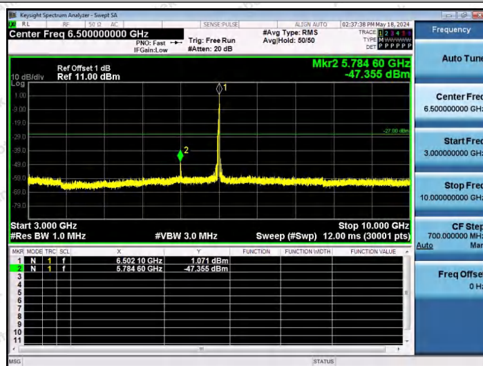
11AX40SISO-Ant1-6485-52Tone-RU44-3000~10000-PASS
