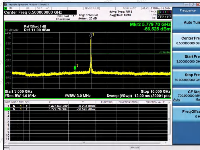
11AX40SISO-Ant1-6485-106Tone-RU53-3000~10000-PASS
