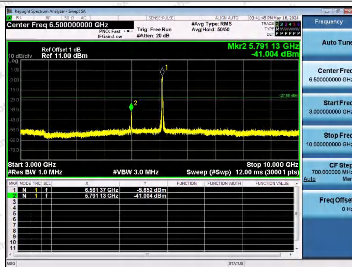
11AX40SISO-Ant1-6565-242Tone-RU61-3000~10000-PASS
