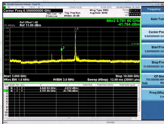
11AX40SISO-Ant1-6525-106Tone-RU56-3000~10000-PASS
