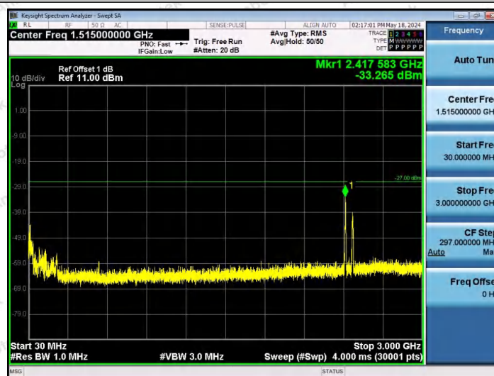
11AX40SISO-Ant1-6445-106Tone-RU56-30~3000-PASS
