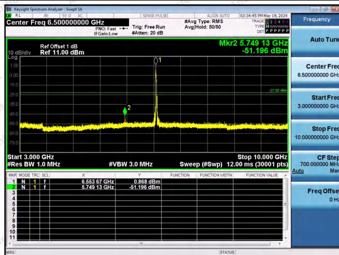
11AX40SISO-Ant1-6565-106Tone-RU53-3000~10000-PASS
