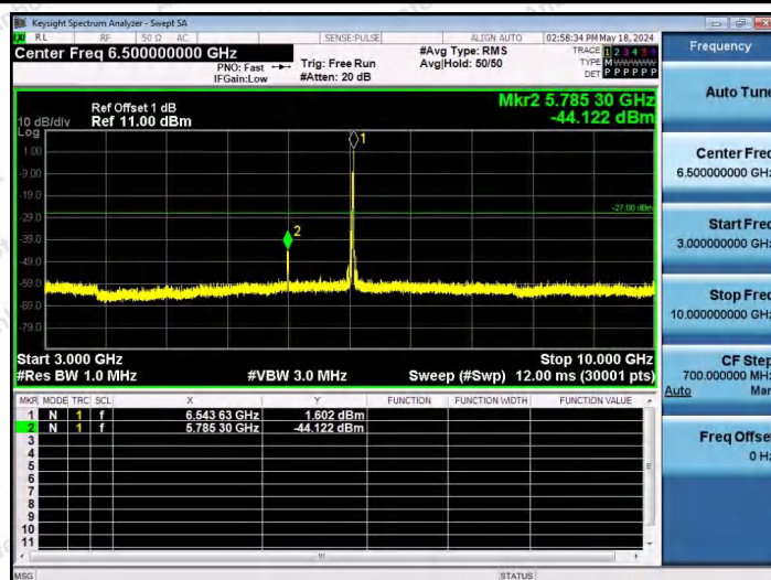
11AX40SISO-Ant1-6525-26Tone-RU17-3000~10000-PASS
