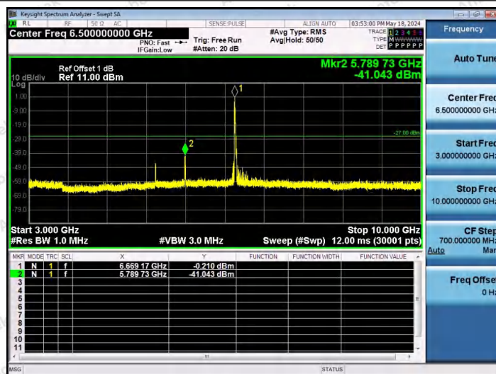
11AX40SISO-Ant1-6685-52Tone-RU37-3000~10000-PASS
