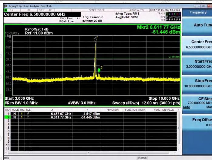
11AX40SISO-Ant1-6445-106Tone-RU56-3000~10000-PASS
