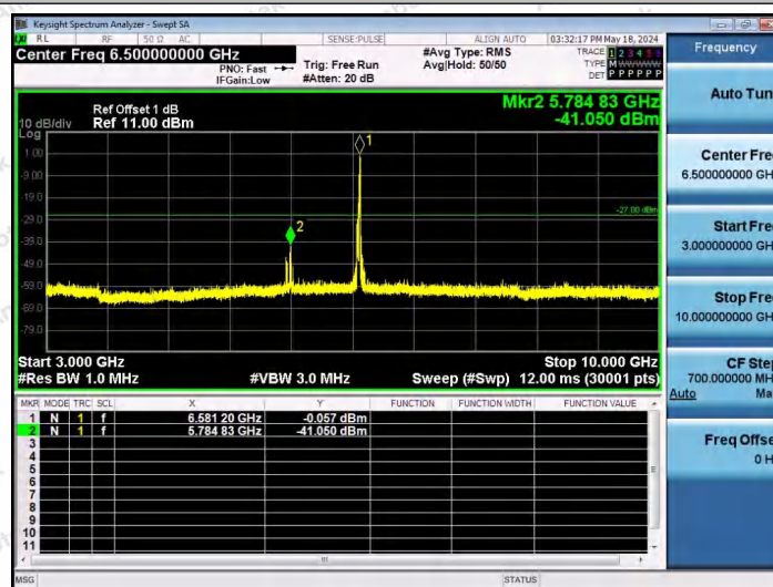
11AX40SISO-Ant1-6565-52Tone-RU44-3000~10000-PASS
