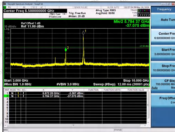
11AX40SISO-Ant1-6685-106Tone-RU53-3000~10000-PASS
