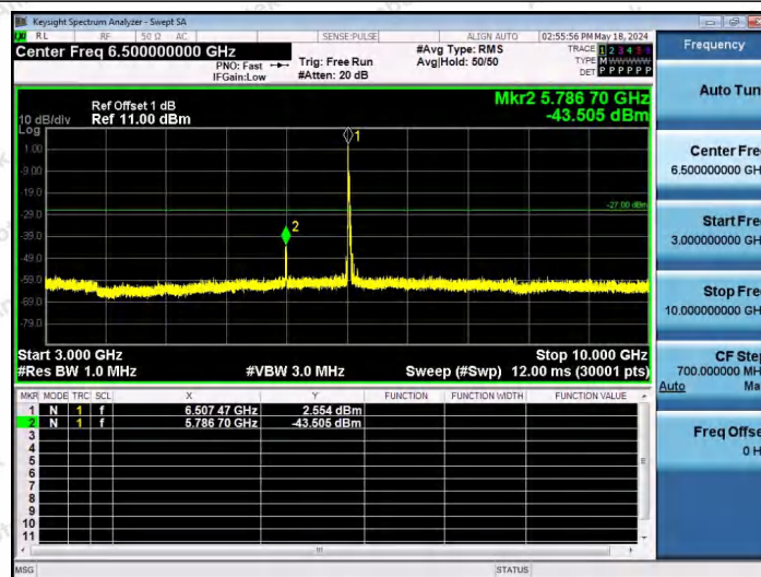
11AX40SISO-Ant1-6525-26Tone-RU0-3000~10000-PASS
