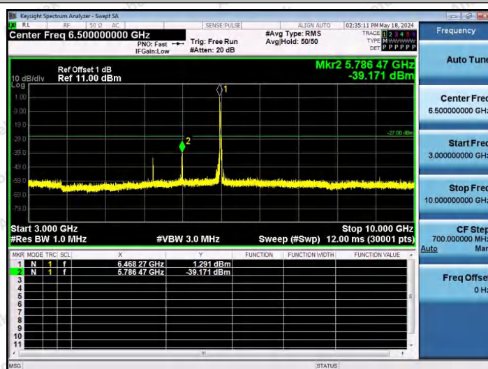
11AX40SISO-Ant1-6485-52Tone-RU37-3000~10000-PASS
