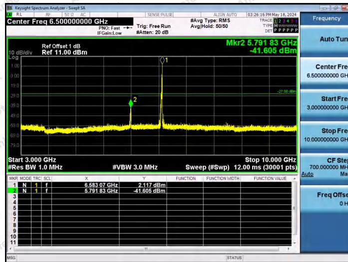
11AX40SISO-Ant1-6565-26Tone-RU17-3000~10000-PASS
