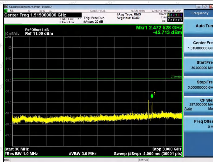
11AX40SISO-Ant1-6525-106Tone-RU56-30~3000-PASS
