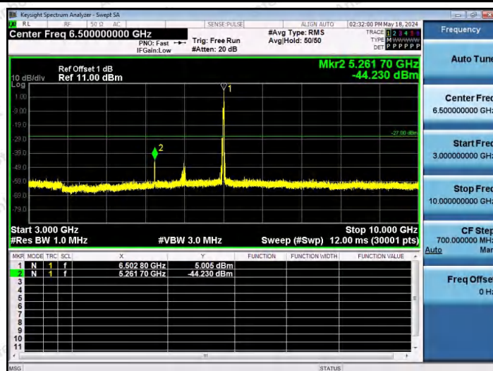
11AX40SISO-Ant1-6485-26Tone-RU17-3000~10000-PASS
