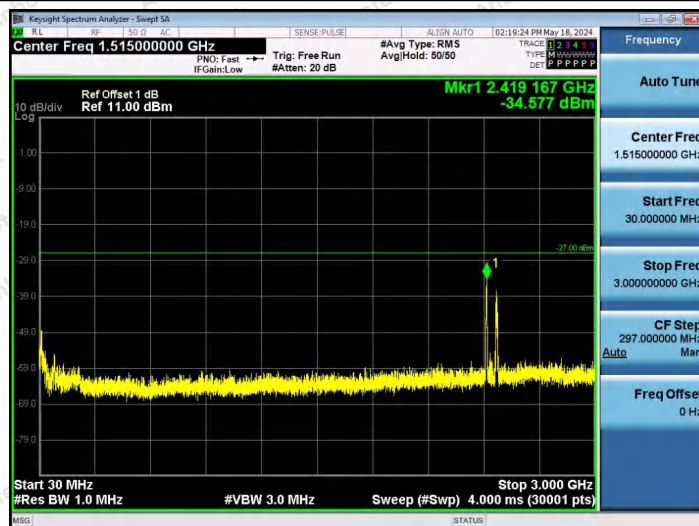
11AX40SISO-Ant1-6445-242Tone-RU61-30~3000-PASS
