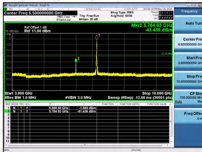
11AX40SISO-Ant1-6685-106Tone-RU56-3000~10000-PASS
